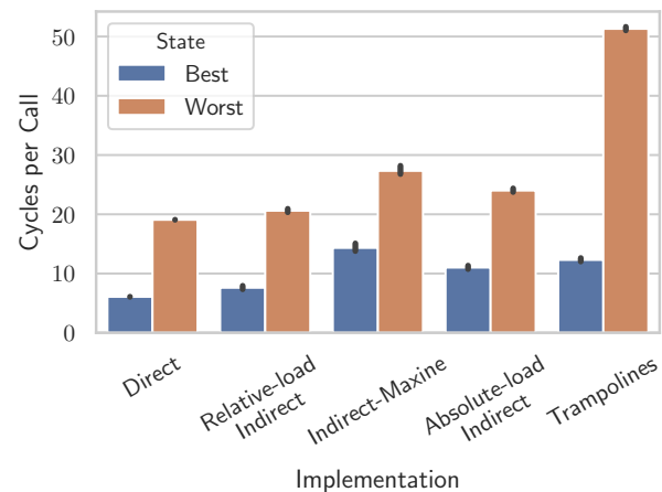
Figure 4. Micro-benchmark results from Odroid-C2 including Maxine’s variation of Indirect-Relative.
