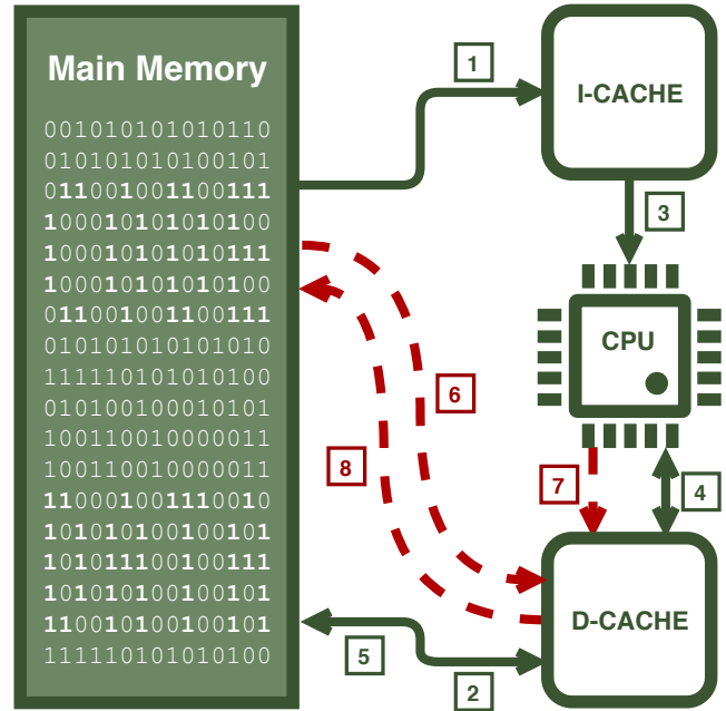
Figure 1. Code-patching illustration.
