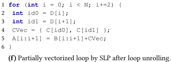
Figure 3. Example shows how the Potential SLP graph obtained by VALU mirrors the SLP’s analysis in the unrolled loop.
