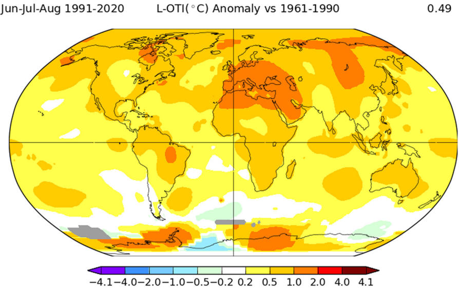
Figure 2. Global distribution of June–August temperature anomaly for 1991–2020 with respect to 1961–1990 base period. From GISTEMP Team (2022) and Lenssen and others (2019).
