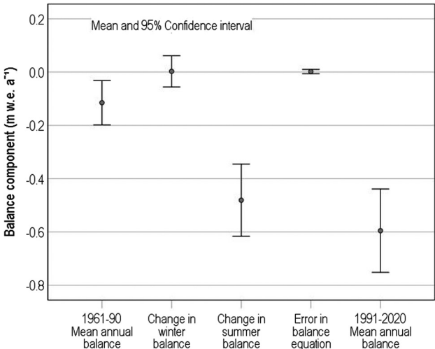
Figure 3. Means and 95% confidence intervals of the five terms in the balance equation for 25 glaciers. Error on x-axis refers to error in Eqn (3).
