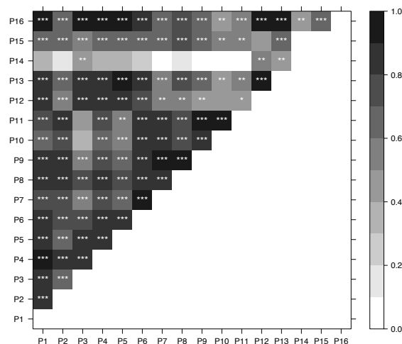
Figure 4. Mantel tests on transition matrices: *** stands for p < 0.001 , ** p < 0.01 and * p < 0.05 , where correlations r > 0.45 .
