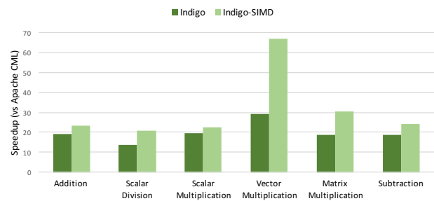
Figure 11: Speedup of Indigo matrices vs Apache CML.
