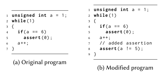
Figure 4: Code snippet example.
