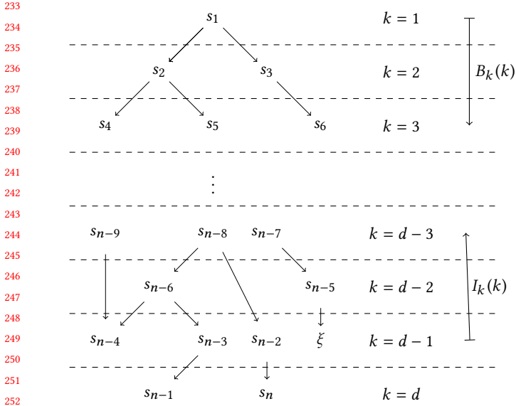
Figure 3: Visual representation of our proposed extension. Each dashed section represents the states reachable after k iterations. The arrows show the “direction” of the verification by the base case B_k(k) and the inductive step I_k(k) . The forward condition F_k(k) is not shown in this representation but it is a forward check, similar to B_k(k) .
