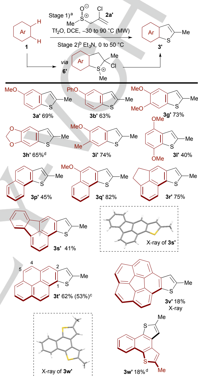
Scheme 3. Scope of the transition metal-free, one-pot synthesis of \pi -extended benzothiophenes. a Stage 1: 1 (0.5 mmol, 1.0 equiv), 2a' (0.5 mmol, 1.0 equiv), Tf 2 O (0.55 mmol, 1.1 equiv), DCE (2.0 mL), -30 °C to 90 °C (MW heating). b Stage 2: Et 3 N (3.0 mmol, 6.0 equiv), 0 °C to 50 °C. c Yield on a larger scale; 0.50 g of 1t gave 0.36 g of 3t' . d Overall yield from 3p' .
