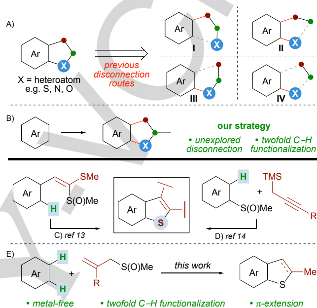
Scheme 1. A) Current routes for heteroarene synthesis. B) Our strategy: direct synthesis of benzo-fused heteroaromatics. C/D) Interrupted Pummerer chemistry for benzothiophene synthesis. E) This work: metal-free synthesis of (dihydro)benzothiophenes.
