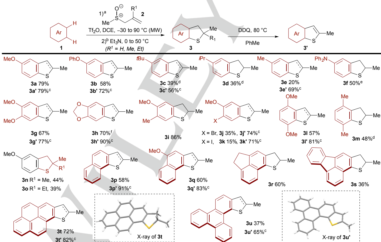
Scheme 2. Scope of the transition metal-free, one-pot synthesis of (2,3-dihydro)benzothiophenes. a Stage 1: 1 (0.5 mmol, 1.0 equiv), 2 (0.5 mmol, 1.0 equiv), Tf 2 O (0.55 mmol, 1.1 equiv), DCE (2.0 mL), -30 °C to 90 °C (MW heating). b Stage 2: Et 3 N (3.0 mmol, 6.0 equiv), 0 °C to 50 °C. c Oxidation: 3 (1.0 equiv), DDQ (1.6 equiv), PhMe (1.0 M) 80 °C. Yield from 3 . d Stage 1: 1 (2.5 mmol, 5.0 equiv). e NMR yield. f Stage 1: -30 °C to 60 °C (MW heating). MW = microwave; DDQ = 2,3-dichloro-5,6-dicyano-1,4-benzoquinone.
