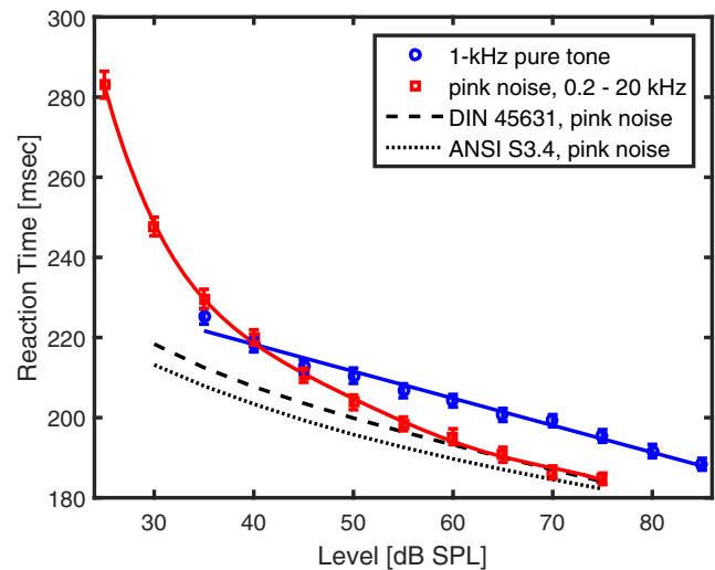
Fig. 2 Results of Experiment 2: Geometric mean reaction times of 21 listeners as a function of sound pressure level for 1-kHz pure tones (blue circles) and pink noise (red squares). Error bars indicate one standard error of the mean into each direction. The dashed line shows predictions made by the DIN 45631 loudness model, using the distance to the regression line of the 1-kHz pure tone for equalizing the LDEL with the LDERT. The dotted line shows the same for ANSI S3.4-2007
