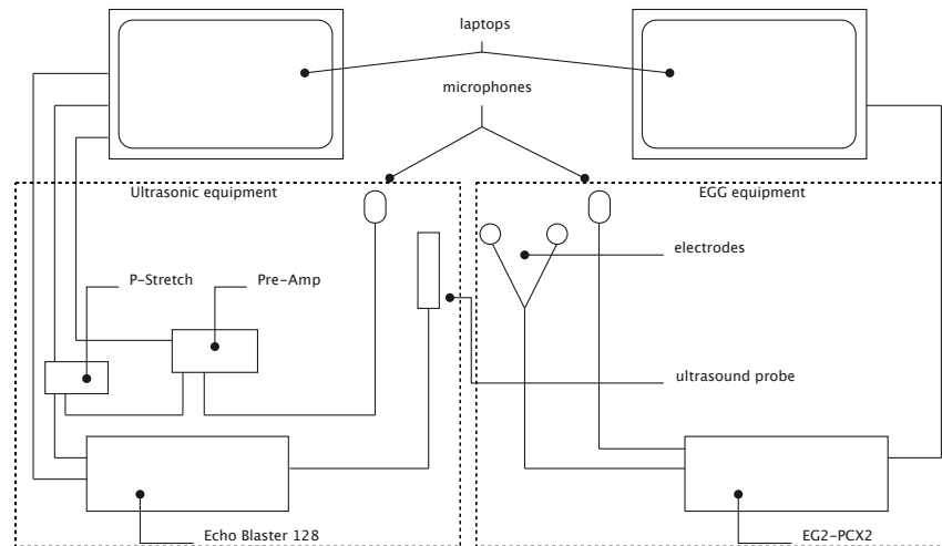
Figure 3.1: Schematics of the equipment set-up of Study I. Stabilisation headset not shown.
