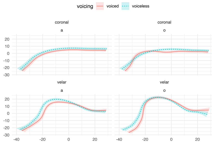
Figure A.16: Tongue contours of voiceless and voiced stops in PL05.
