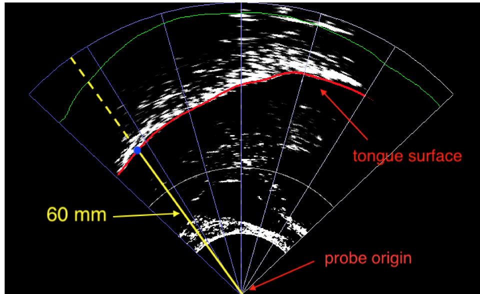
Figure 6.1: Schematics of the operationalisation of tongue root position, based on Kirkham & Nance (2017). The tongue root surface corresponds to the lower edge of the white band in the image. The tongue tip is on the right side. The outline of the fan-like coordinate systems is shown. The yellow line starting from the probe origin is the selected fan-line from which tongue root position is calculated (see text for the method of fan-line selection). Tongue root position thus corresponds to the distance (in millimetres) between the probe origin and the intersecting point of the tongue surface with the selected fan-line.
