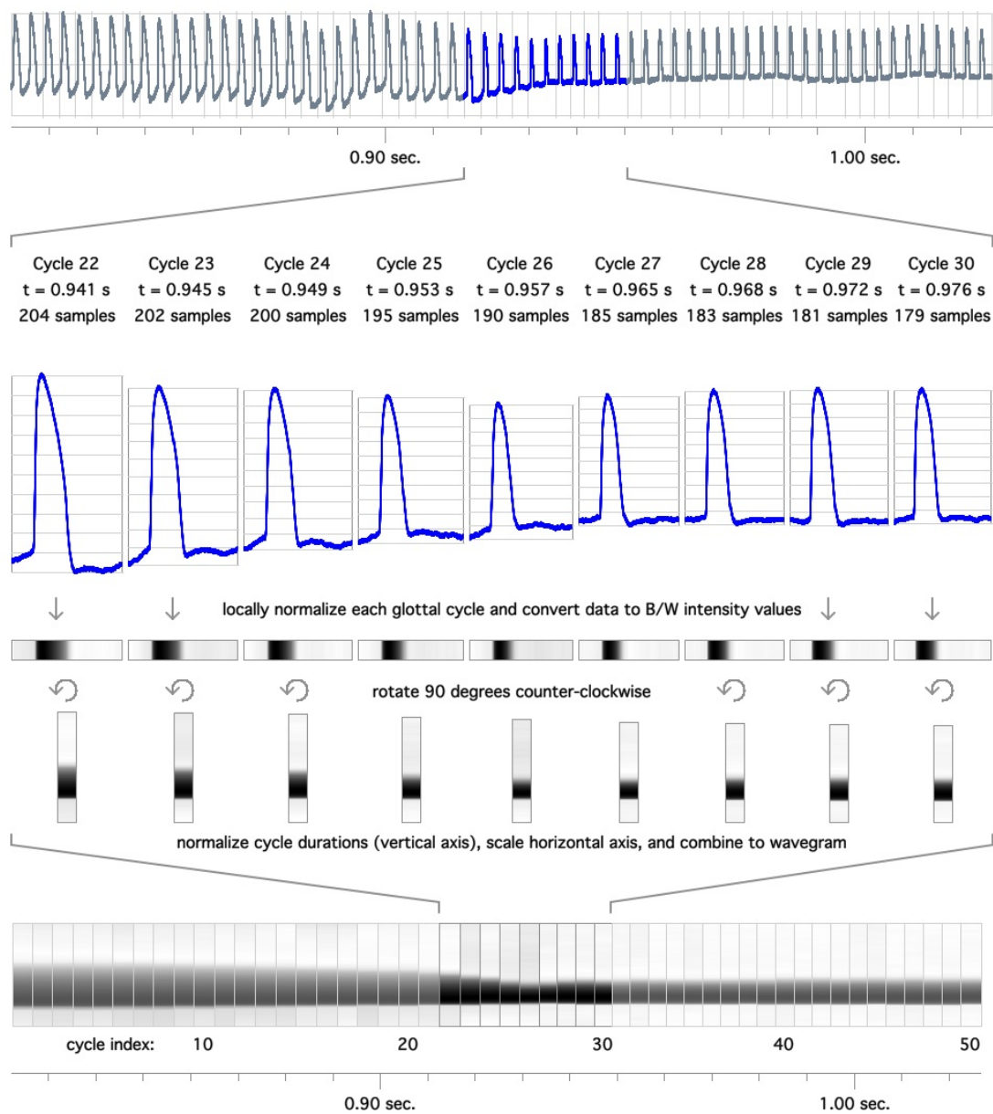
Figure 7.3: The wavegram. Created by Christian T. Herbst under a CC BY-SA 3.0 license.
