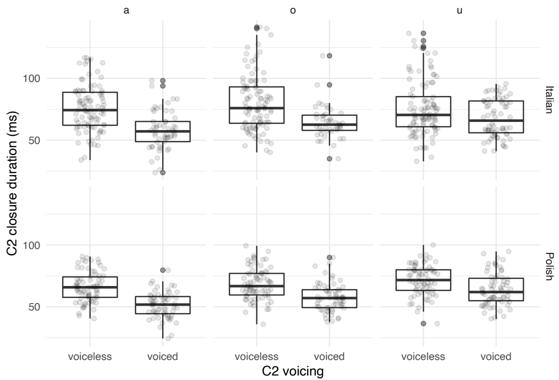
Figure 4.3: Raw data and boxplots of closure duration in milliseconds of voiceless and voiced stops in Italian (top row) and Polish (bottom row) when preceded by the vowels /a, o, u/.
