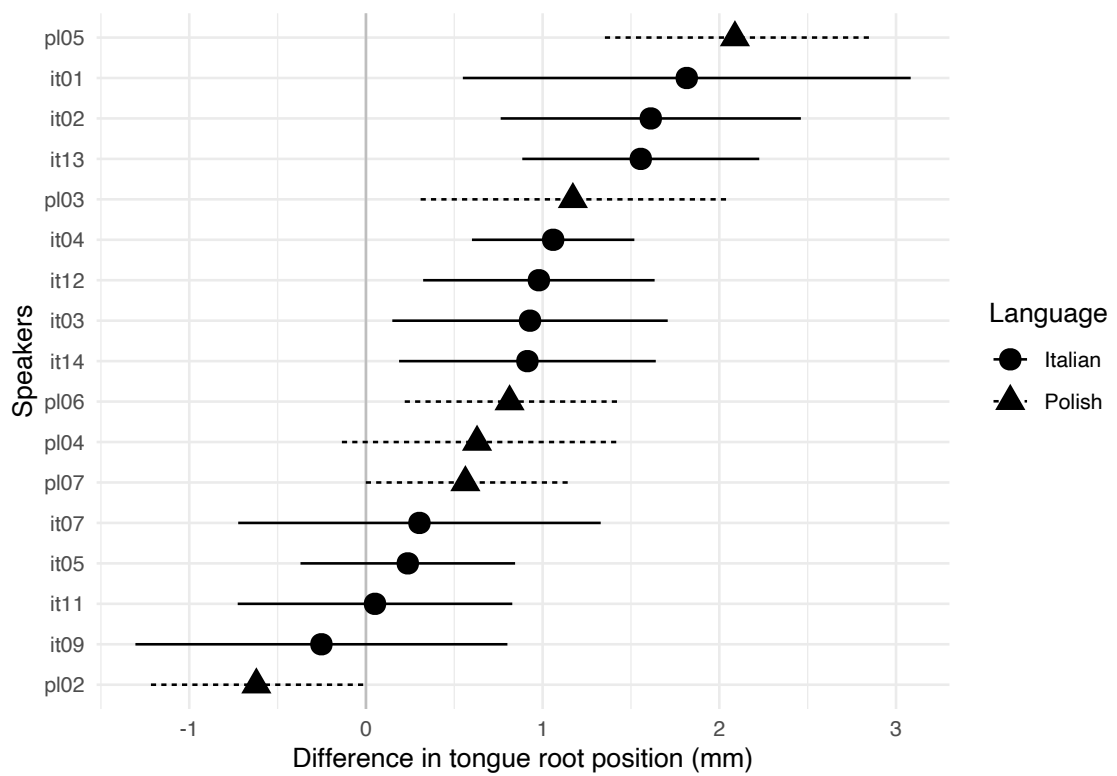
Figure 6.7: By-speaker raw mean difference in tongue root position between voiceless and voiced stops at closure onset (in millimetres). The horizontal segments are the standard errors of the mean differences.
