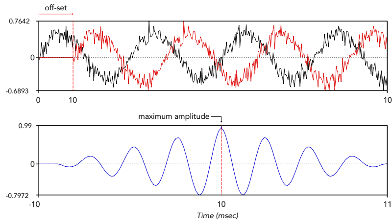
Figure 3.3: Synchronisation of two sounds by cross-correlation. The top panel shows the waveforms of two identical sounds, one of which has been offset by 10 ms. The bottom panel shows the cross-correlation of the two sounds in the top panel. The offset of the sounds corresponds to the time of maximum amplitude in the cross-correlated sound.
