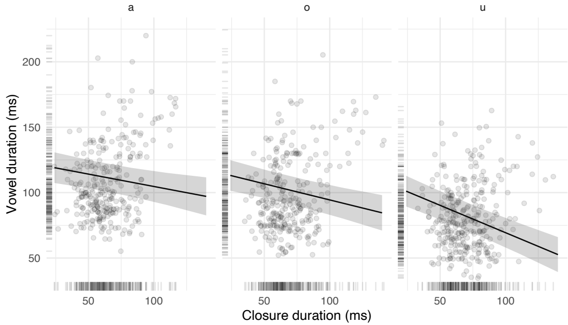
Figure 4.4: Raw data, estimated regression lines, and 95 per cent confidence intervals of the effect of closure duration on vowel duration for the vowels /a, o, u/ (from a mixed-effects model fitted to data pooled from Italian and Polish, see text for details).
