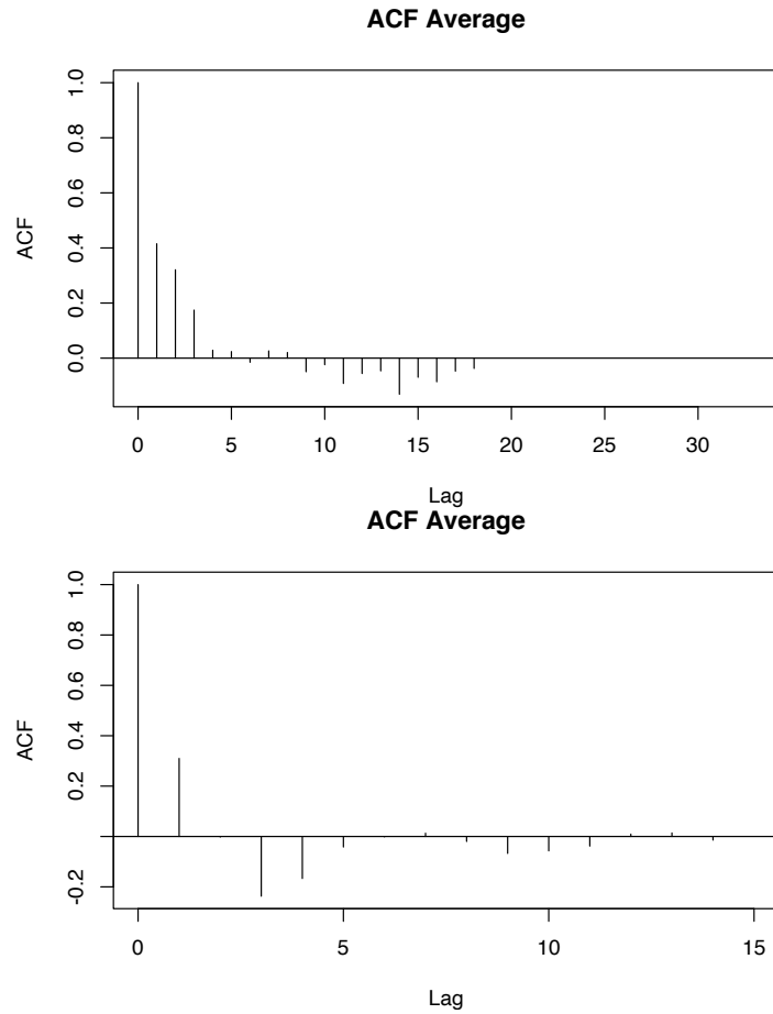
Figure A.6: Autocorrelation plots of a model fitted without (top) and with (bottom) a first-order autoregressive model (AR1).
