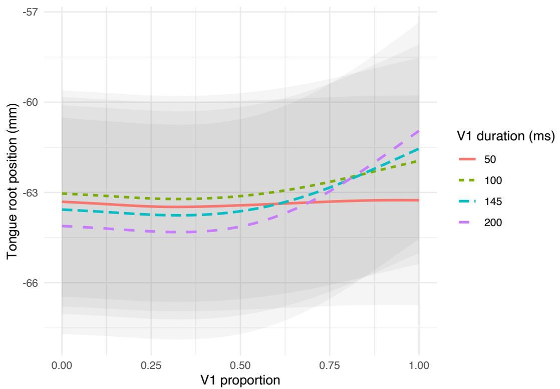
Figure 6.5: Predicted tongue root position during vowels at 4 exemplifying values of vowel duration, with 95% confidence intervals. Predictions from a GAMM (see Section 6.3.4).
