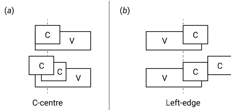
Figure 8.1: Gestural organisation patterns for onsets (a) and codas (b). C = consonant, V = vowel (design based on Marin & Pouplier 2010).
