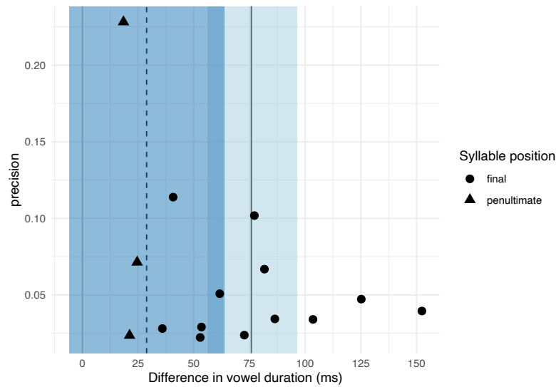
Figure B.4: By-study funnel plot showing the estimate against the precision. The vertical thick and dashed lines are the meta-analytical means of the effect in final and penultimate position.
