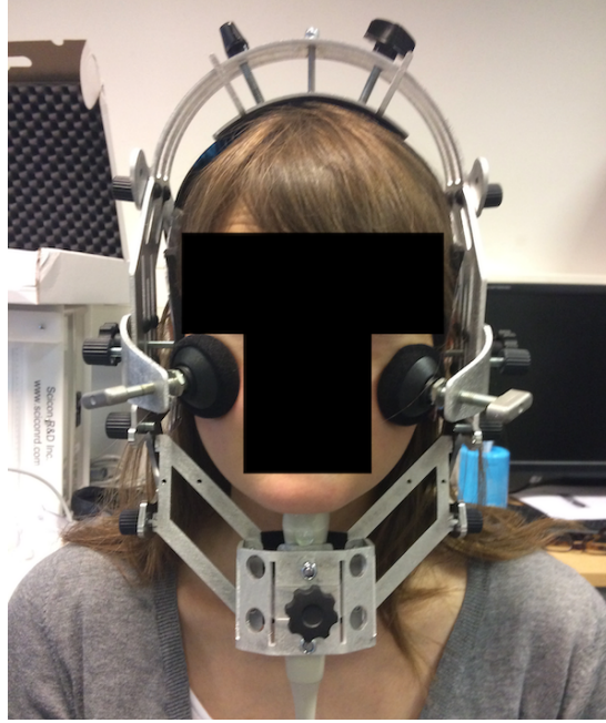
Figure 3.2: Ultrasonic probe stabilisation headset.
