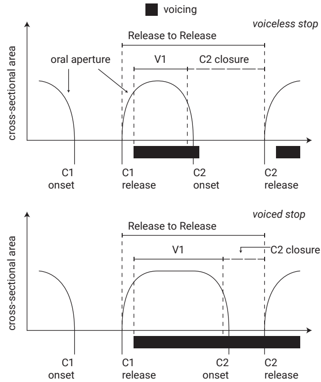
Figure 4.7: A schematic representation of the oral cavity cross-sectional area, as inferred from acoustics. Design based on Esposito (2002). The top panel shows a CVC sequence with a voiceless C2, the bottom panel with a voiced C2. Oral cavity aperture (on the y-axis, as the inverse of oral constriction) through time (on the x-axis) is represented by the black line. Lower values represent a more constricted oral tract (a contoid configuration), while higher values indicate a more open oral tract (a vocoid configuration). The black bars below the time axis represent voicing (vocal fold vibration). Various landmarks and intervals are indicated in the schematic.
