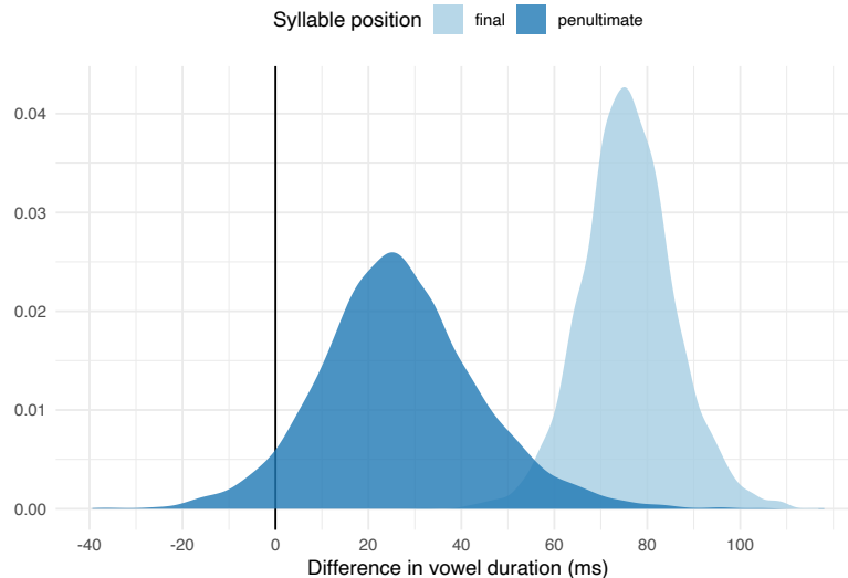
Figure B.2: Meta-analytical posterior distributions of the voicing effect in syllable-final and penultimate position.
