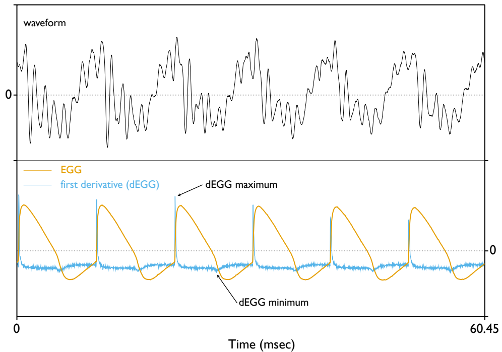
Figure 7.2: The electroglottographic signal (EGG) with corresponding first derivative (dEGG).
