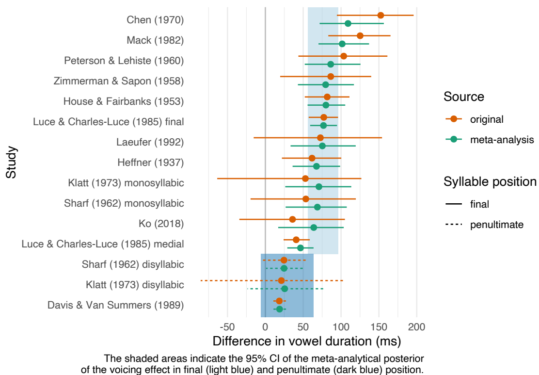
Figure B.3: Estimated voicing effect from the original source and from the meta-analysis.
