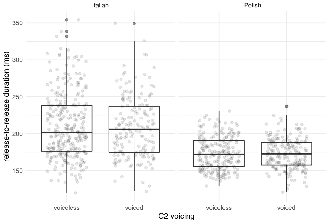
Figure 4.5: Raw data and boxplots of the duration in milliseconds of the release-to-release interval in Italian (left) and Polish (right) when C2 is voiceless or voiced.
