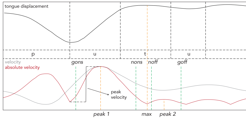
Figure 3.4: Gestural landmarks of tongue movements in the word putu . The top panel shows tongue tip displacement, while the bottom panel shows tangential and absolute velocity.
