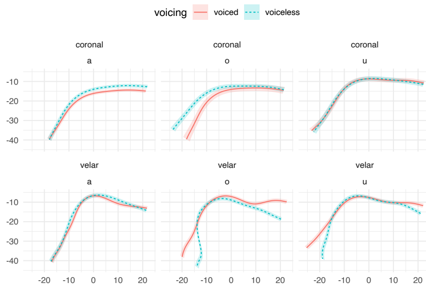
Figure A.12: Tongue contours of voiceless and voiced stops in IT11.
