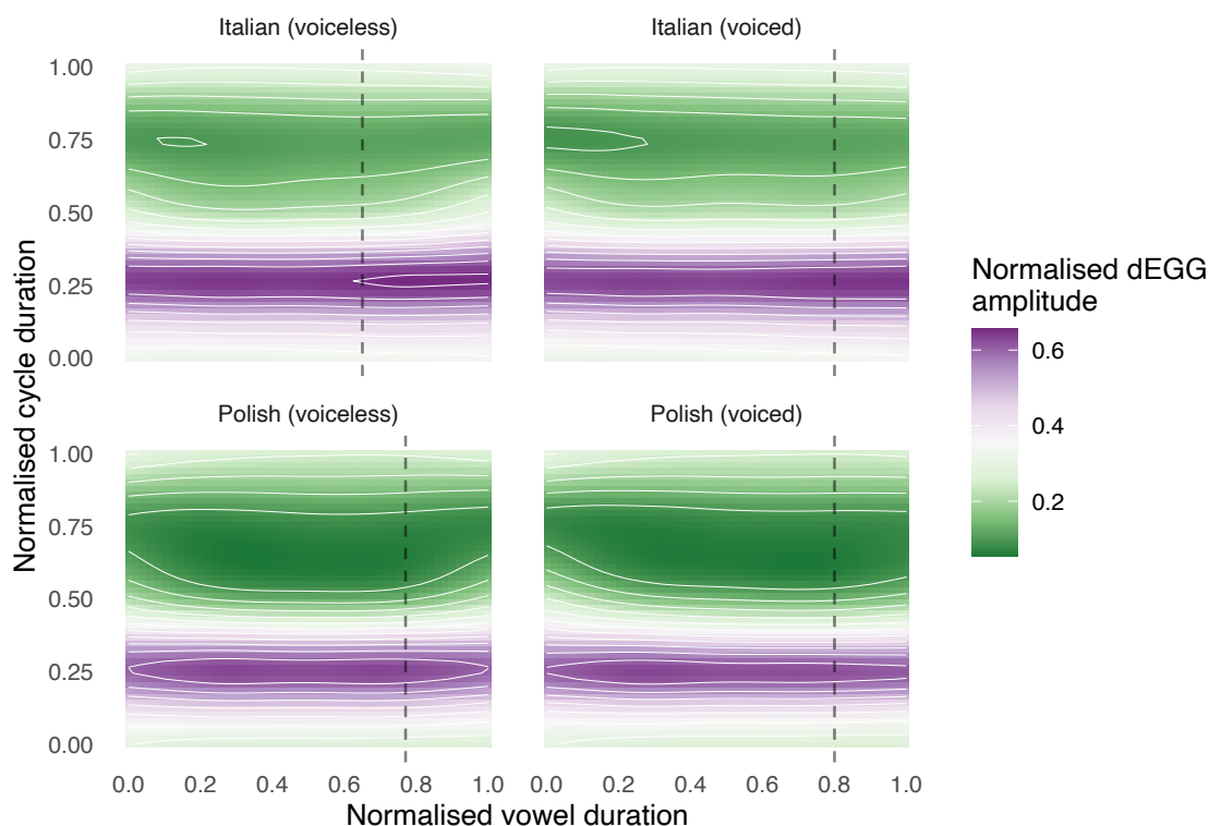
Figure 7.5: Fitted wavegram of vowels followed by voiceless and voiced stops in Italian and Polish (Section 3).
