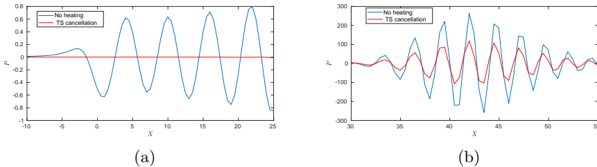
Figure 14: Comparisons of the pressure perturbation with \omega = 2.5 at T = (4 + 1/4)T_{per} with and without wave cancellation using (4.4): (a) for the restricted range in x , and in (b) over an extended range showing the wave packet.
