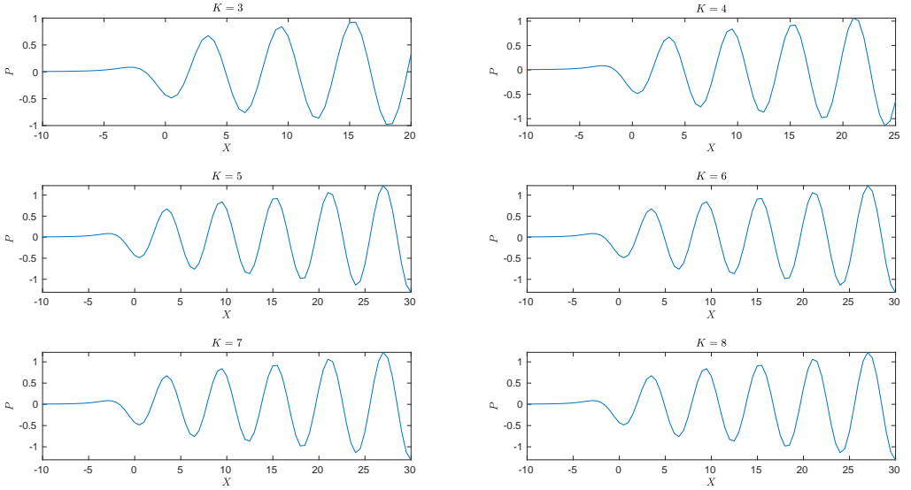
Figure 11: Results for the pressure perturbation with \omega_0 = 2.5 (unstable) at times \tau = (K + \frac{1}{4})T_{per} , K = 3, 4, 5, 6, 7, 8 and no vibrator, forced by unsteady heating.
