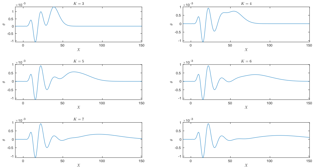
Figure 12: Temperature profile \theta(X, Y_j, \tau) with g(X, \tau) = h(X)q(\tau) , h(x) = 0 and \omega = 2.5 with Y_j \approx 7.759 at times \tau = (K + \frac{1}{4})T_{per} , K = 3, 4, 5, 6, 7, 8 .
