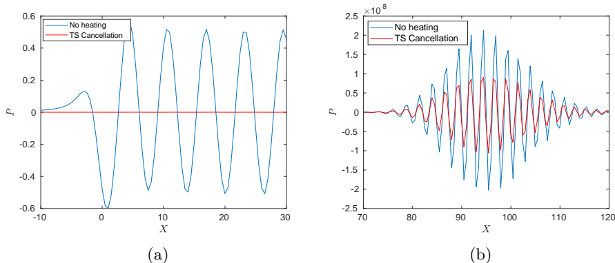
Figure 17: Comparison of the pressure perturbations at T = (8 + 1/4)T_{per} with and without wave cancellation using (4.4) for the neutral case with \omega_0 = 2.298 (a) for restricted range in X , and in (b) over an extended range showing the wave packet.
