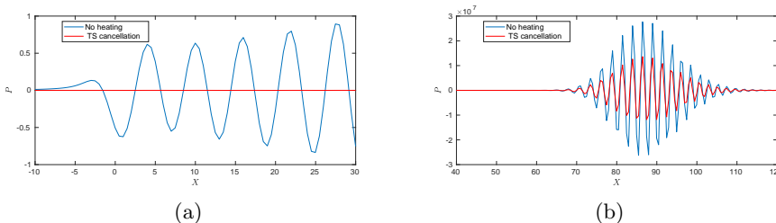
Figure 15: Comparison of the pressure perturbations with \omega = 2.5 at T = (8 + 1/4)T_{per} with and without wave cancellation using (4.4): (a) for restricted range in x , and in (b) over an extended range showing the wave packet.
