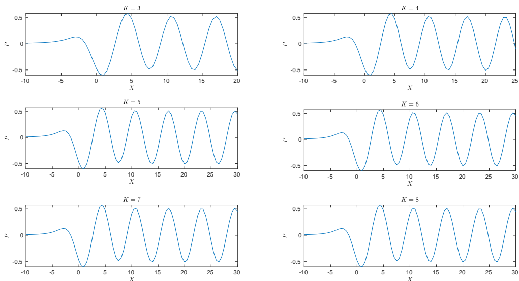
Figure 7: Results for the pressure perturbation with \omega_0 = 2.298 (neutral) at times \tau = (K + \frac{1}{4})T_{per} , K = 3, 4, 5, 6, 7, 8 , with g(\tau, X) = 0 (no heating).
