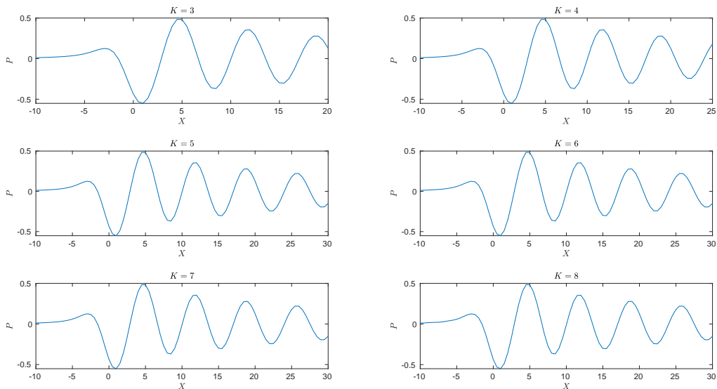
Figure 6: Results for the pressure perturbation with \omega_0 = 2 (stable) at times \tau = (K + \frac{1}{4})T_{per} , K = 3, 4, 5, 6, 7, 8 , with g(\tau, X) = 0 (no heating).
