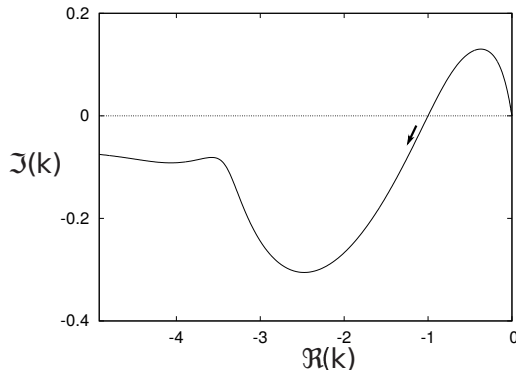
Figure 5: Locus of the root \omega_{1,1}(k) = i\omega_0 with \omega_0 varying from 0 to \infty . The arrow indicates the direction of \omega_0 increasing.
