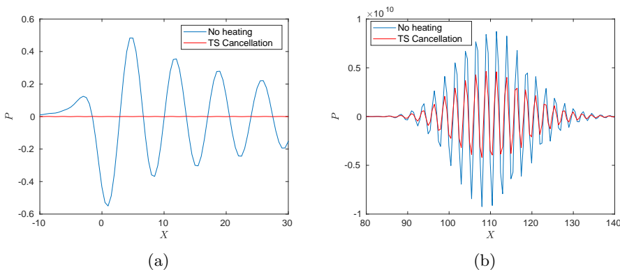
Figure 16: Comparison of the pressure perturbations at T = (8 + 1/4)T_{per} with and without wave cancellation using (4.4) for the stable case with \omega_0 = 2 . (a) for restricted range in x , and in (b) over an extended range showing the wave packet.
