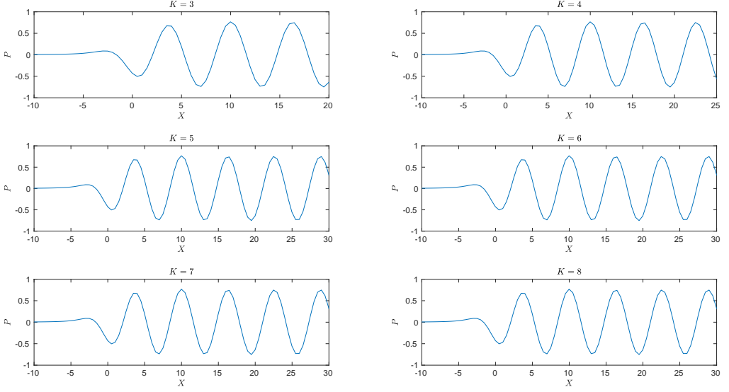
Figure 10: Results for the pressure perturbation with \omega_0 = 2.298 (neutral) at times \tau = (K + \frac{1}{4})T_{per} , K = 3, 4, 5, 6, 7, 8 and no vibrator, forced by unsteady heating.
