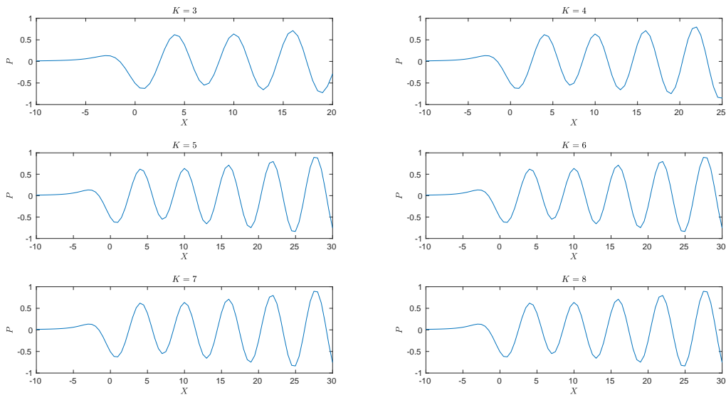
Figure 8: Results for the pressure perturbation with \omega_0 = 2.5 (unstable) at times \tau = (K + \frac{1}{4})T_{per} , K = 3, 4, 5, 6, 7, 8 , with g(\tau, X) = 0 (no heating).
