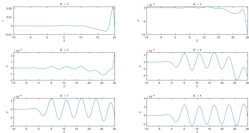
Figure 13: The pressure perturbation P_a(\tau, X) with \omega = 2.5 and T-S cancellation in action using the heating function given by (4.4) at times \tau = (K + \frac{1}{4})T_{per} , K = 3, 4, 5, 6, 7, 8 .
