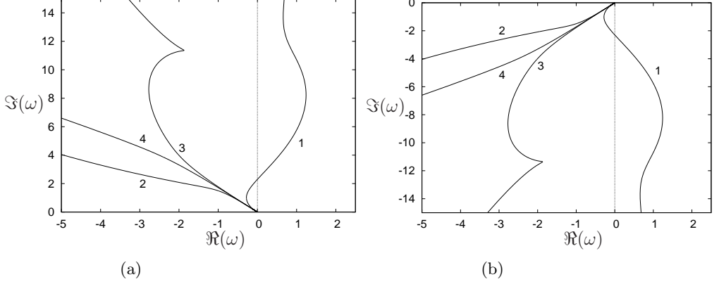
Figure 3: Locus of the (a) roots \omega_{1,j} of D^-(\xi_0, k) = 0 for k varying from (-\infty, 0) and (b) \omega_{2,j} of D^+(\xi_0, k) = 0 with k varying from (0, \infty) . The labels correspond to the different roots \omega_{1,j}, \omega_{2,j} , j = 1, 2, \dots
