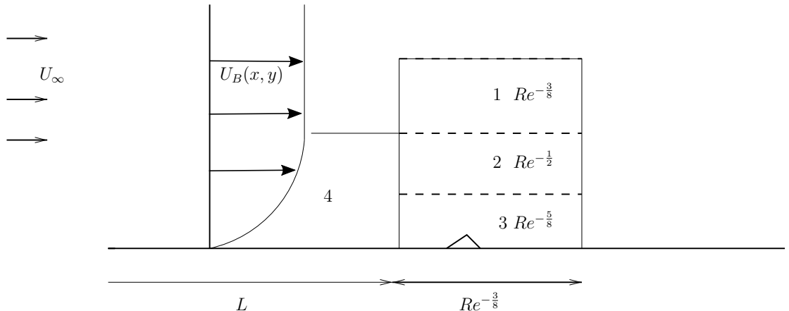
Figure 2: Schematic diagram showing the vibrator, triple-deck region and oncoming boundary layer flow. Region 1 with y = Re^{-3/8}y_1 is the upper-deck, region 2 with y = Re^{-1/2}y_2 is the main part of the boundary layer and region 3 with y = Re^{-5/8}y_3 the lower-deck. The oncoming boundary flow just ahead of the vibrator is represented by region 4.
