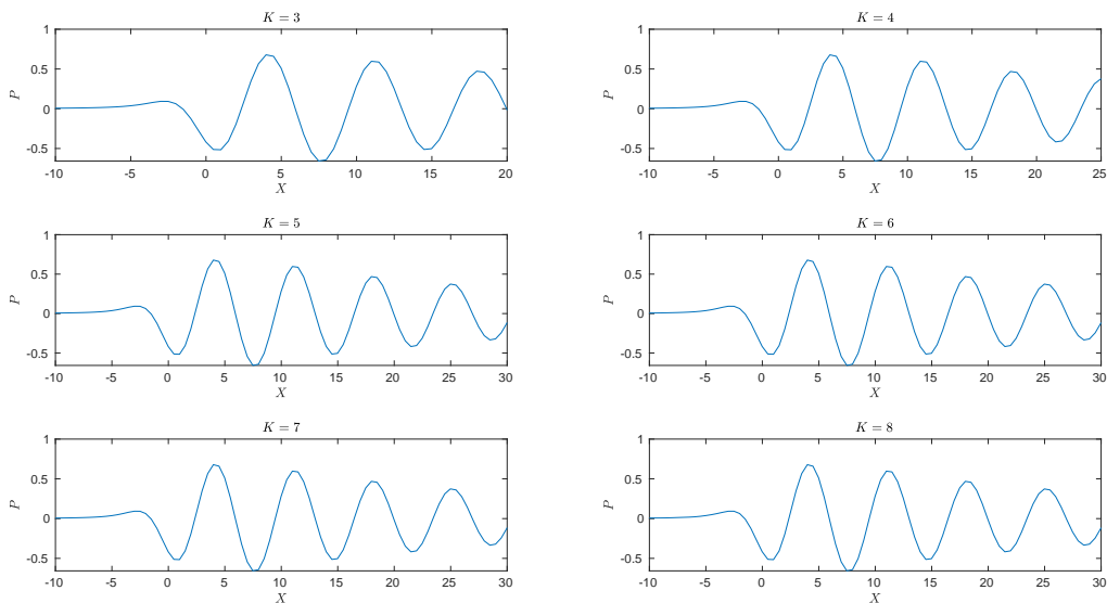
Figure 9: Results for the pressure perturbation with \omega_0 = 2 (stable) at times \tau = (K + \frac{1}{4})T_{per} , K = 3, 4, 5, 6, 7, 8 and no vibrator, forced by unsteady heating.
