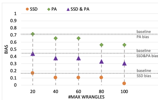
(a) Fairness bias
