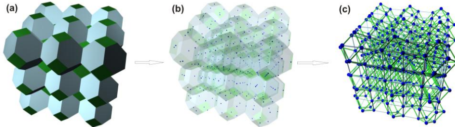
Figure 1. Discrete model for GB diffusion: (a) cellular representation of a polycrystal; (b) sites at cell faces; (c) site-bond model with bonds of variable diffusivities according to Eq. 4.
