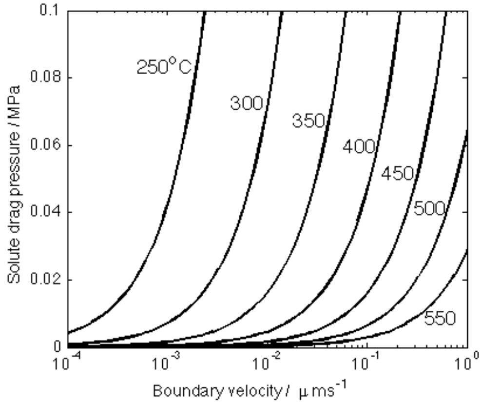
FIGURE 7. Calculated solute drag pressure as a function of boundary velocity for Y at temperatures ranging from 523–823 K (250–550 Celsius).
