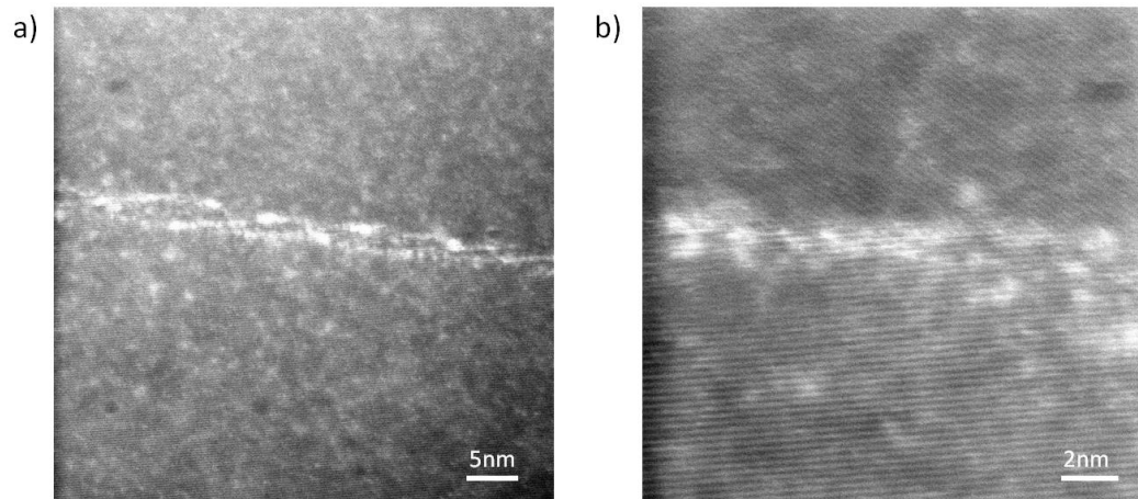
FIGURE 2. HAADF STEM images showing segregation of Y at grain boundaries at a) low and b) higher magnification.
