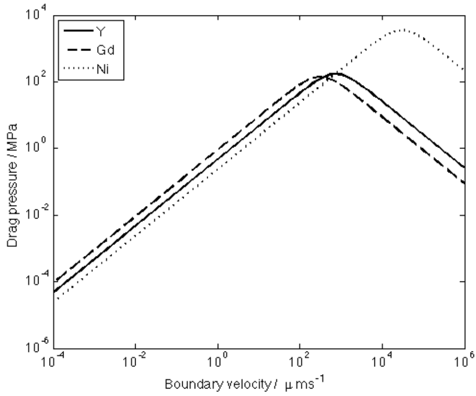
FIGURE 6. Calculated solute drag pressure as a function of boundary velocity for Y, Gd, and Ni at 673 K (400 Celsius).
