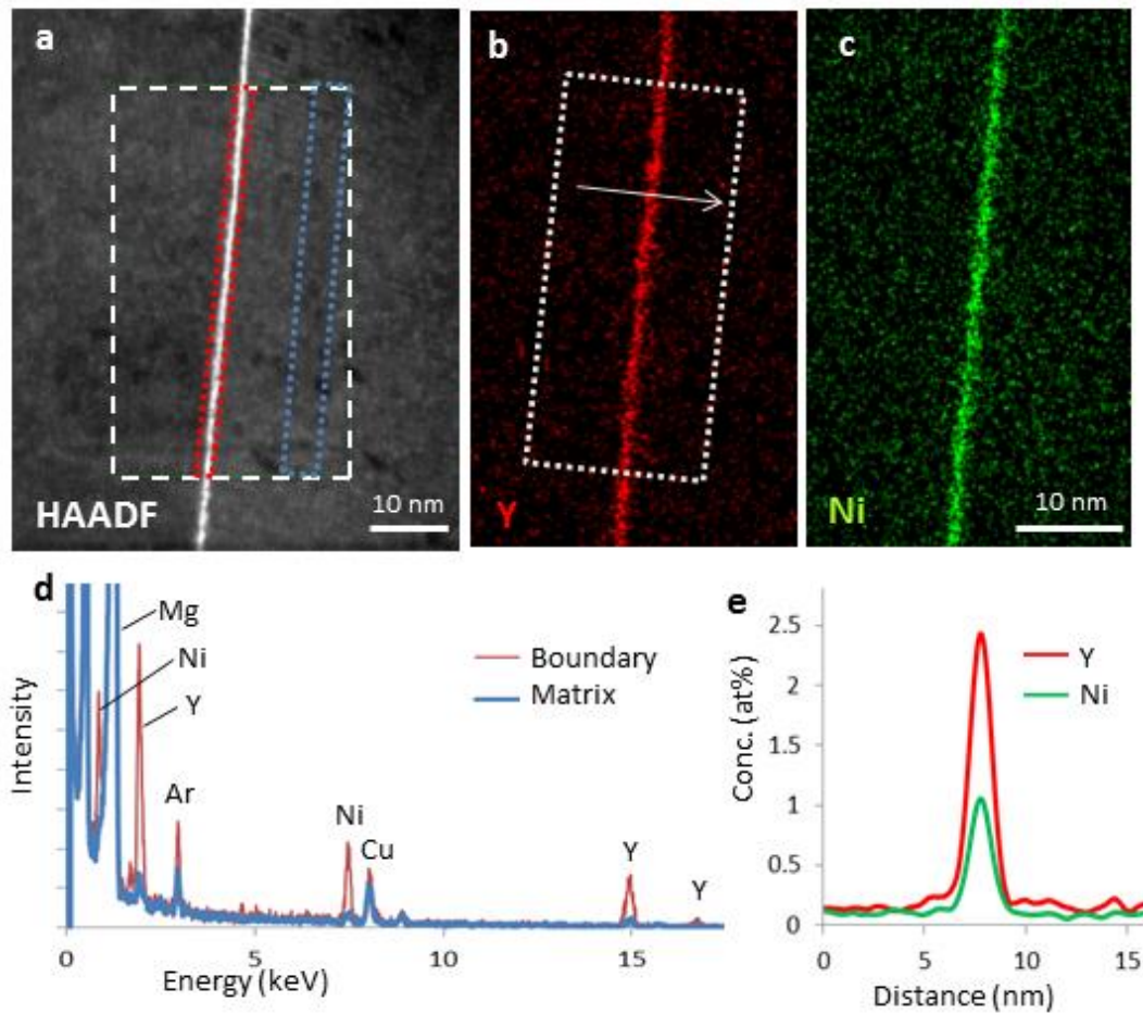
FIGURE 3. Energy dispersive X-ray spectrum imaging of grain boundary segregation. (a) HAADF STEM images showing grain boundary region. (b,c) Elemental maps for Y and Ni extracted from the EDX spectrum image. (d) EDX spectra summed over the region of grain boundary and of the matrix illustrated by the red and blue dashed line in (a). Summed spectra have been normalised to the Mg peak, The presence of Ar and Cu in both spectra are the result of ion polishing sample preparation and scattering from the TEM sample holder respectively. (e) Semi-quantitative analysis showing Y and Ni enrichment at the grain boundary for the region shown by the dashed rectangle in (b).
