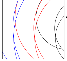
Figure 3: Part of sphere data in \mathbb{R}^2 observed on an open square U = (-1, 1)^2 : Spherical surfaces with three center points (black dots) where the radius of the sphere is coded with color. In \mathbb{R}^2 the sphere data consist of the set U and all pairs (t, \Sigma) , where \Sigma \subset U is a circular arc of radius t .
