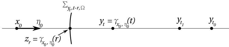
Figure 2: Notation used throughout the paper, following the geodesic \gamma .
