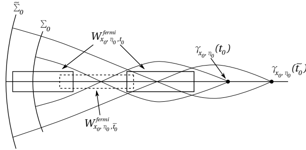
Figure 4: Reconstruction procedure in the case of conjugate points.
