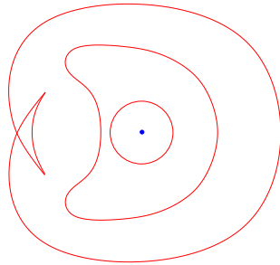
Figure 1: Generalized spheres centered at a point: For small radii the generalized spheres resemble the Euclidean spheres but for large radii cusps corresponding to caustics may appear. For example the outermost contour in the figure illustrates a generalized sphere containing two cusps. If we were to trace from this contour backwards to the center point along the rays we would see that some of the rays cross each other. The sphere data consists of smooth subsurfaces of these generalized spheres.
