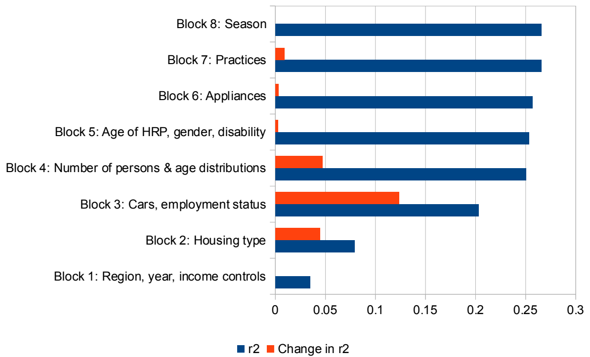
Figure 2: Contribution of variable blocks to explanatory power of the linear regression model reported in Table 2
