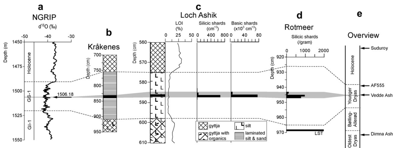
Fig. 2. The stratigraphic position of the Vedde Ash (VA). (a) In the NGRIP ice core the VA lies within Greenland Stadial 1 (GS-1) at 1506.18 metres depth (Mortensen et al., 2005; Rasmussen et al., 2006); (b) In Kråkenes, Norway, the VA is a visible layer midway through the Younger Dryas stadal sediments (Mangerud et al., 1984; Birks et al., 2000); (c) In Loch Ashik, Scotland, both rhyolitic and basaltic shards are found within silts associated with the Loch Lomond stadial (British Isles equivalent to the Younger Dryas), as confirmed by the loss-on-ignition (LOI) profile (this study; Davies et al., 2001; Pyne-O'Donnell, 2011); (d) in Rotmeer, Switzerland, only rhyolitic shards have been found as a cryptotephra layer (Blockley et al., 2007; Lane et al., in press-a). This layer lies approximately 25 cm above the Laacher See Tephra (LST). (e) Overview stratigraphical profile (not to scale) showing the position of the VA in relation to the chemically similar tephra layers discussed in this paper: the Suðuroy tephra (Wastegård, 2002); the AF555 tephra (Matthews et al., 2011); the Dimna Ash (Koren et al., 2008).
