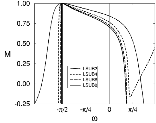
FIG. 2. Results for the CCM sublattice magnetization of the spin-half J_1 - J_2 model on the 2D square lattice, using the LSUB m approximation based on the Néel model state, with m = 2, 4, 6, 8 . Note that J_1 \equiv \cos \omega and J_2 \equiv \sin \omega .
