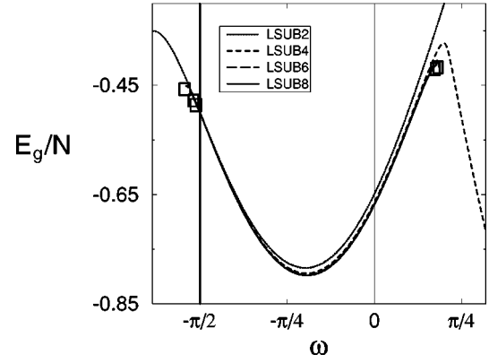
FIG. 1. Results for the CCM ground-state energy of the spin-half J_1 - J_2 model on the 2D square lattice, using the LSUB m approximation based on the Néel model state, with m=2,4,6,8 . LSUB m critical points \omega_F and \omega_A are indicated by the boxes. Note that J_1 \equiv \cos \omega and J_2 \equiv \sin \omega .
