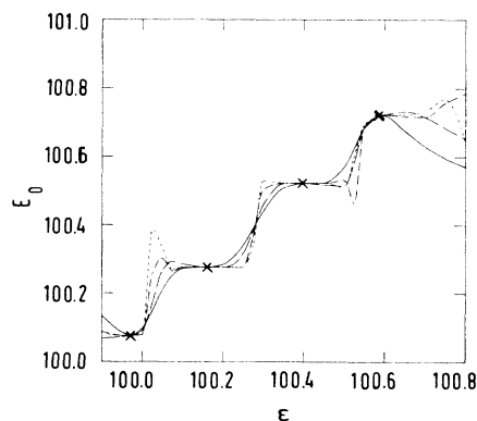
FIG. 1. Results for the energy, calculated via the ground-state formalism, of the tridiagonal Hamiltonian of Eq. (49), with \lambda=(0.2,0.4) and \lambda_0=(0.19,0.28) , with a matrix size M=4 . We have used a subspace size t=1 , and results are shown as a function of the free parameter \varepsilon , for perturbation order N=1 (solid line), 2 (long dashes), 5 (medium dashes), and 10 (short dashes). The points [E_i(\lambda_0), E_i(\lambda)] are marked with the symbol \times , emphasizing that, for this Hamiltonian, when \varepsilon = E_i(\lambda_0) , MRSPT produces the energy E_i(\lambda) exactly, even at first order.
