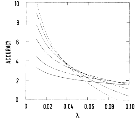
FIG. 7. Accuracy (as defined in Fig. 2) of the ground-state energy of the anharmonic oscillator vs \lambda calculated via standard RSPT as in Bender and Wu (Ref. 11). Perturbation orders shown are N=1, 2, 4, 6, 8 , and 10 and are marked as in Fig. 3.
