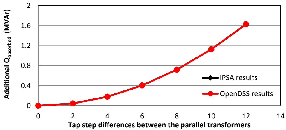
(a) Additional reactive power absorption of the transformers
