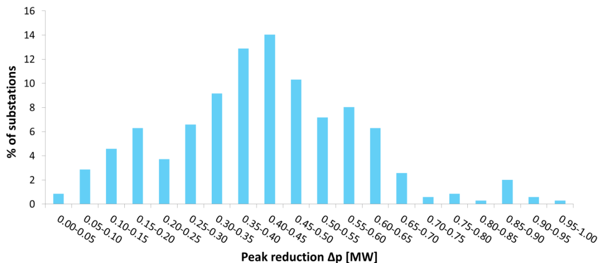
Figure 3 Peak reduction with np=1.1 and \Delta V=3\% for all primary substation in ENWL area
