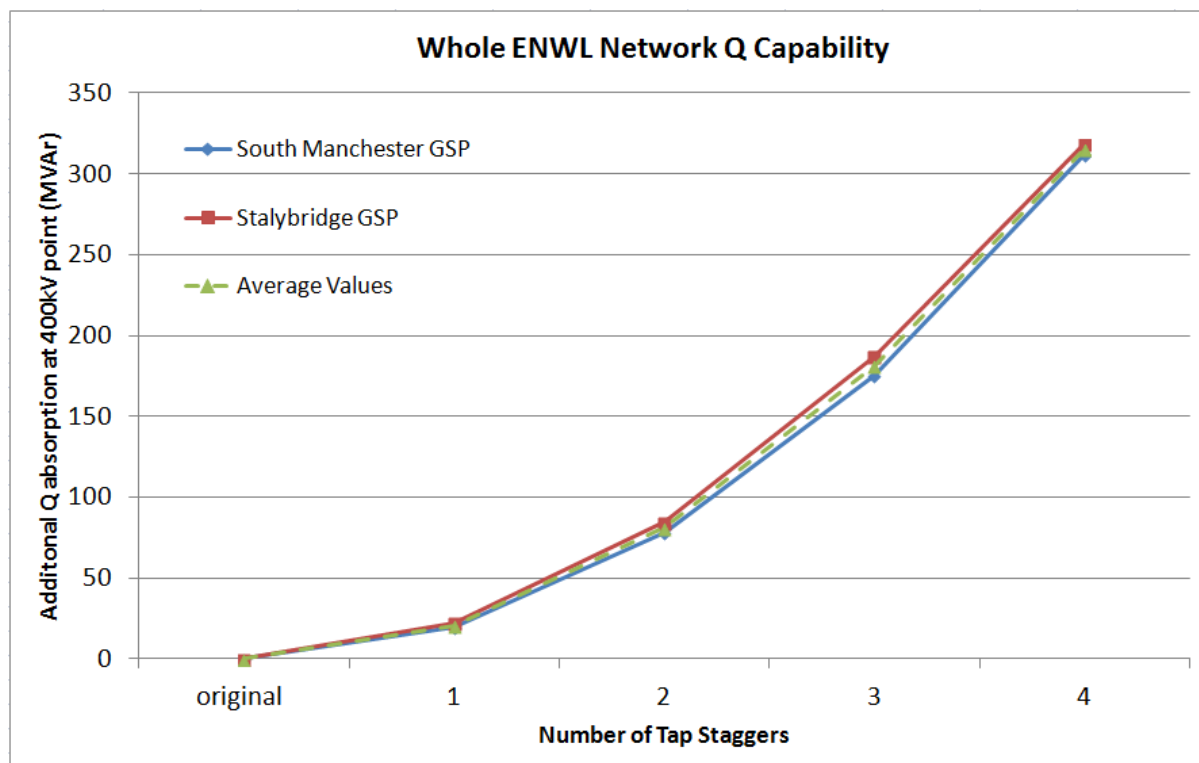
Figure 22. The comparison results between the averaging estimation and the actual estimated reactive power absorption capability of South Manchester and Stalybridge GSPs.
