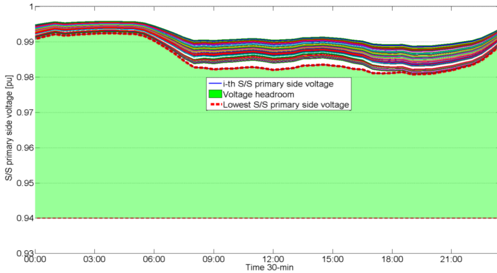
Figure 10 Estimated voltage headroom (green area) for voltage reduction for Romiley primary substation (3 rd September)
