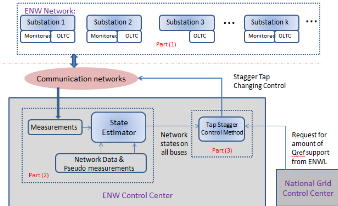
Figure 12: Methodology flow chart of WP2 – network additional Q absorbability study
