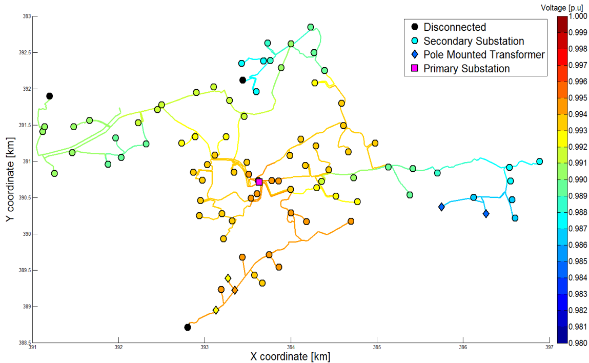
Figure 9 Romiley HV network voltage heat map at 18:30 (3 rd September)
