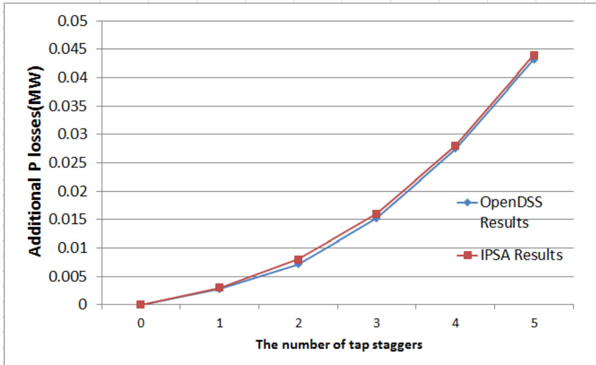
Fig.17(b):Active power loss against the number of tap stagers
