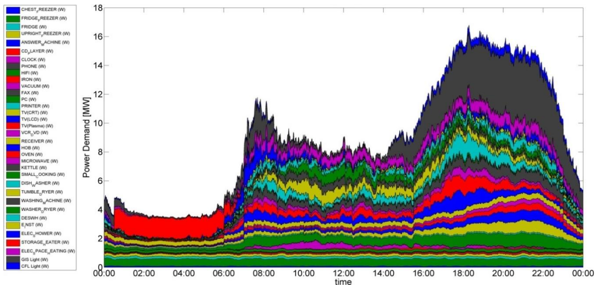
Figure 5 Aggregated active power and breakdown per appliance during peak demand for Didsbury primary substation
