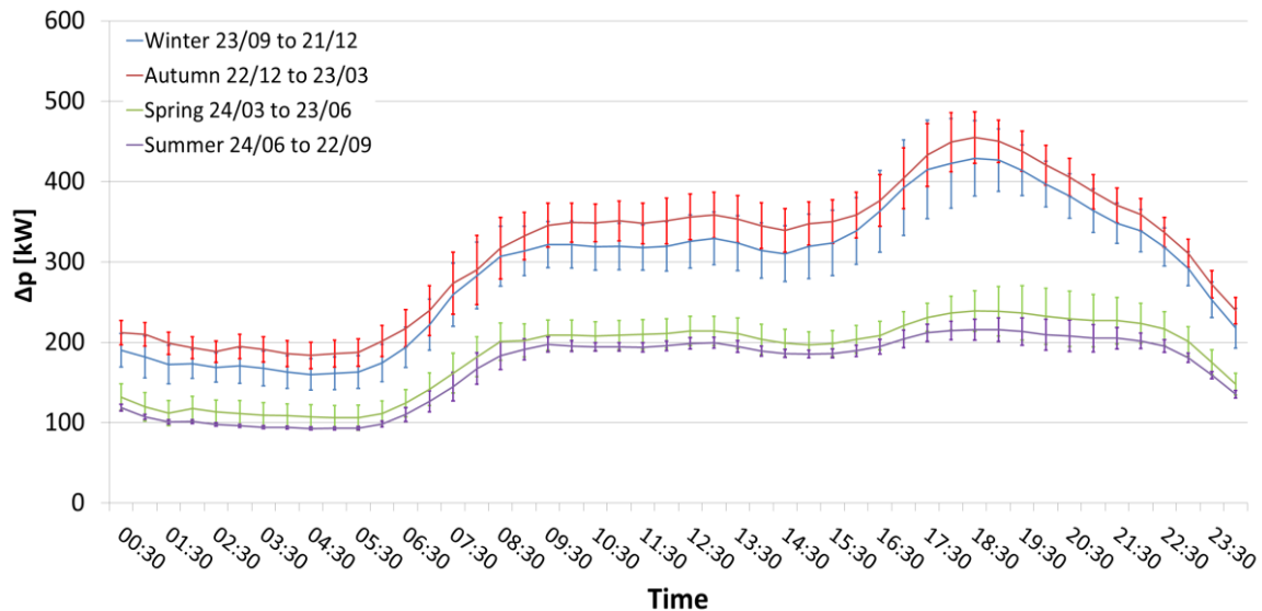
Figure 2 Seasonal average and standard deviation active power variation achievable in Didsbury primary substation
