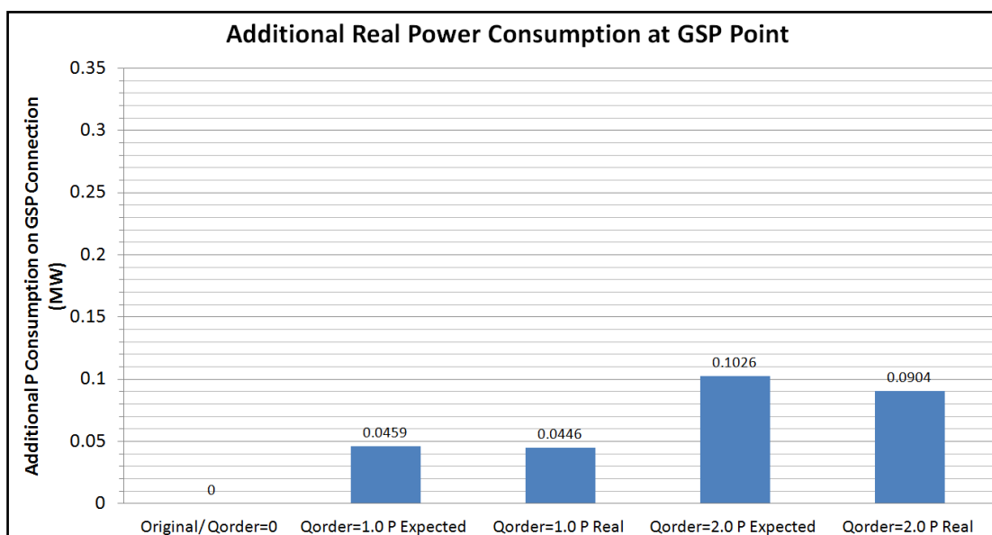
Figure 20: P changes at the power source point due to tap staggering
