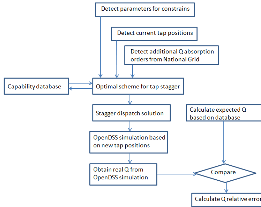
Figure 18: The flow chart of the implemented optimal tap stagger search method
