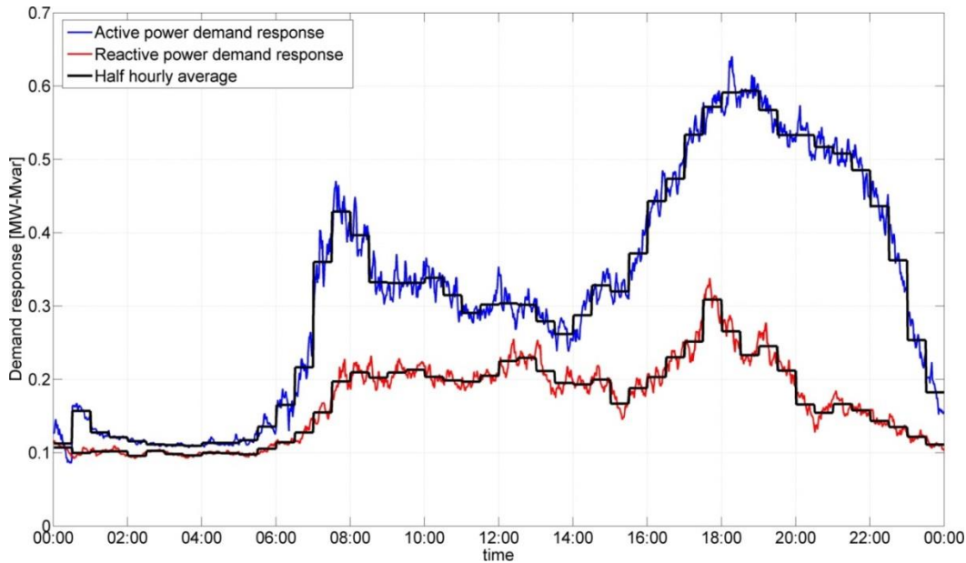
Figure 7 Potential active and reactive power variation at peak demand day for Didsbury primary with half hourly average ( \Delta V=3\% )
