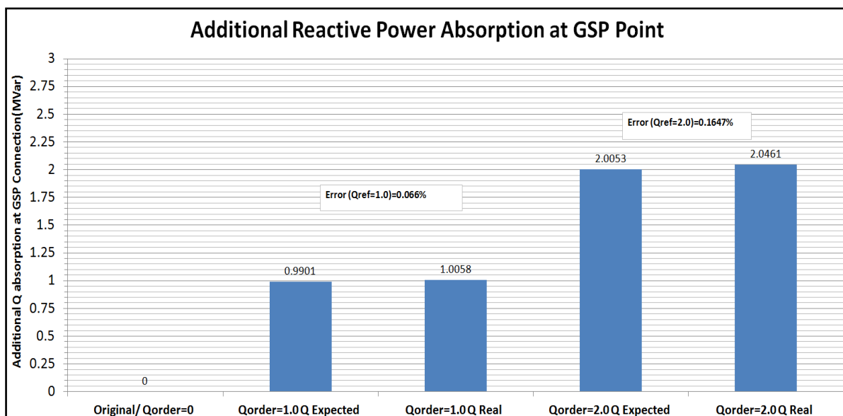
Figure 19 Q changes at the power source point due to tap staggering
