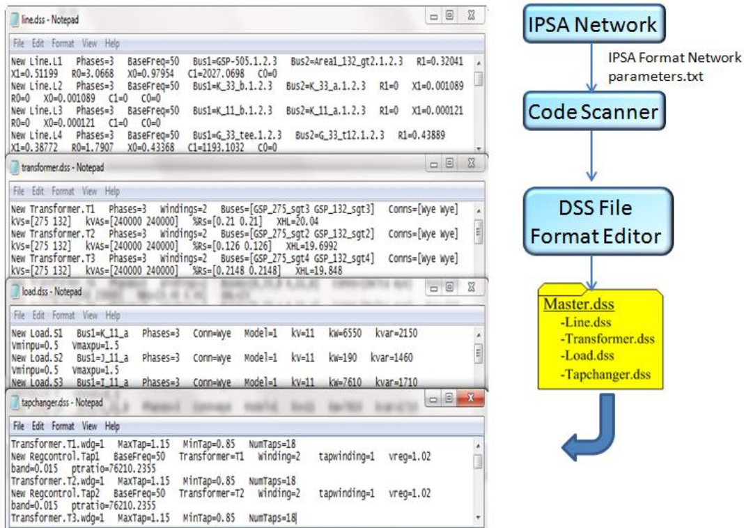
Figure 14: IPSA to OpenDSS Conversion Flow Chart
