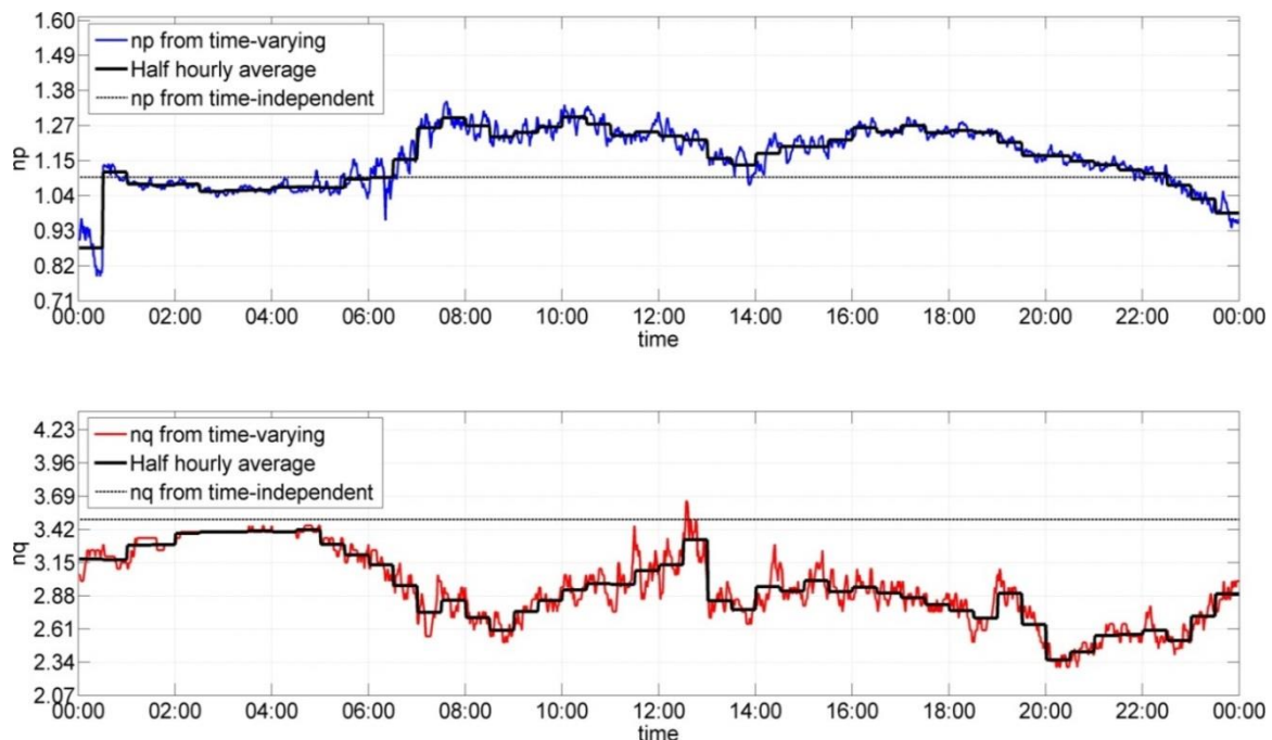
Figure 6 np and nq factor for the peak day for Didsbury primary substation
