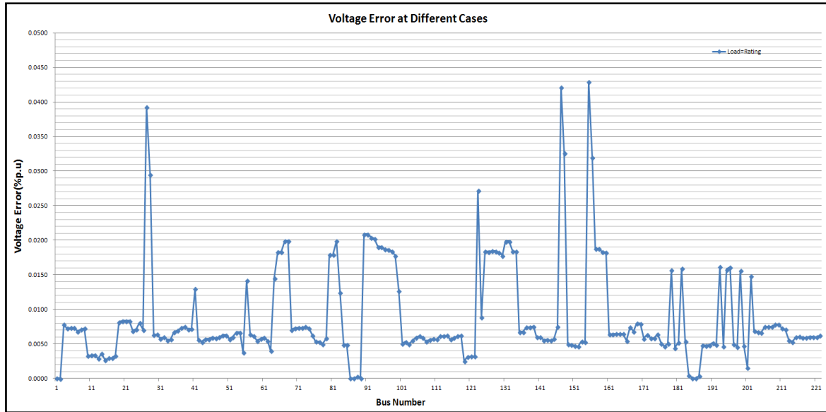
Figure 15(a): Voltage difference on all buses under the rated load conditions
