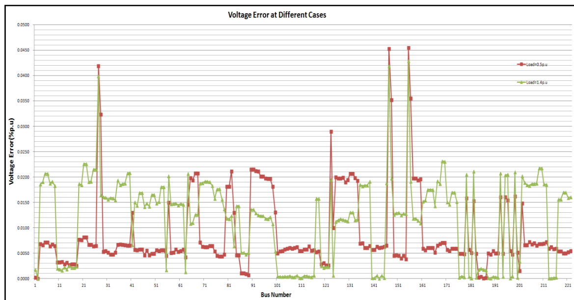
Figure 15(b): Voltage difference on all buses under 0.5p.u and 1.4 p.u load condition, respectively
