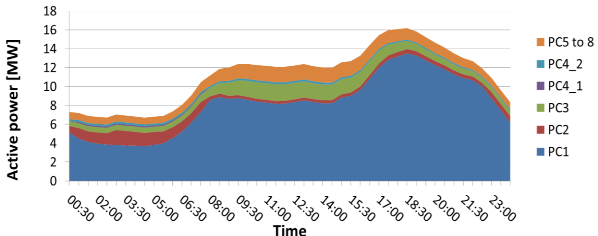
Figure 1 Estimated demand profile during the peak day, 13 th December 2012
