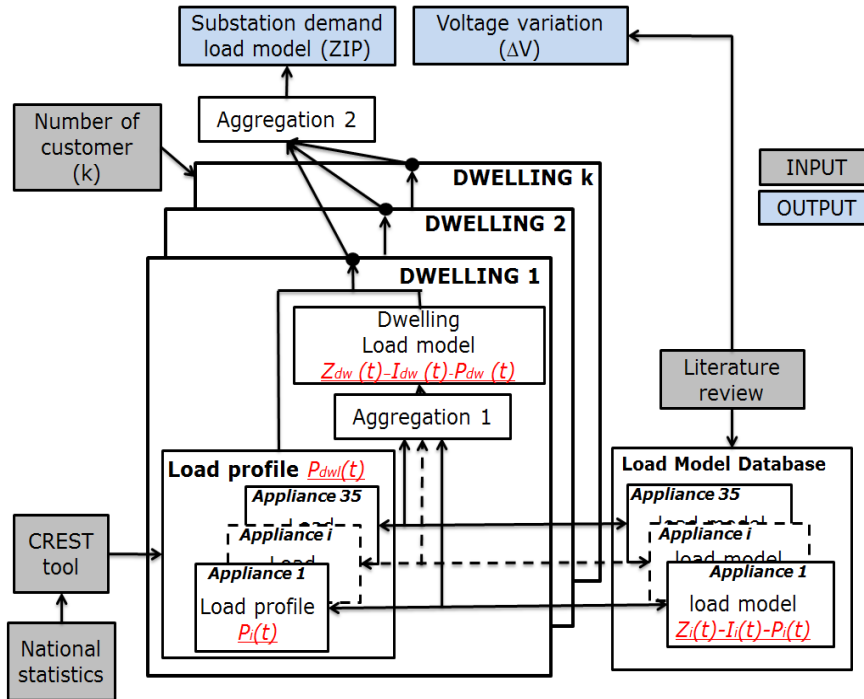
Figure 4 Adopted time-varying approach to model the residential demand, [4]
