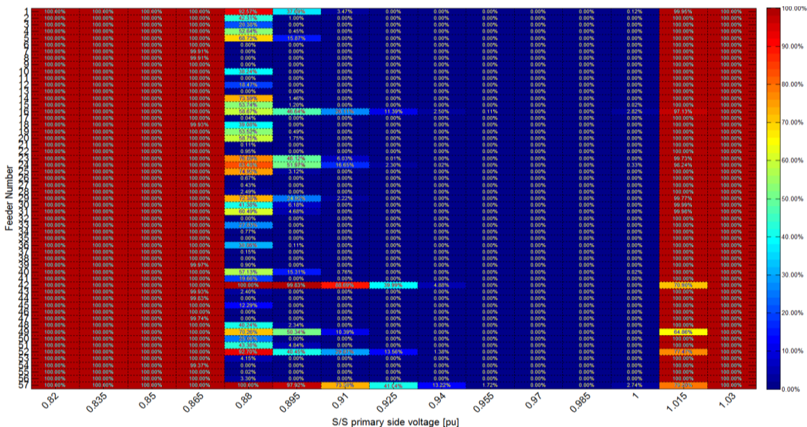
Figure 8 Average percentage of non-compliant customer per feeder and LV transformer primary side voltage
