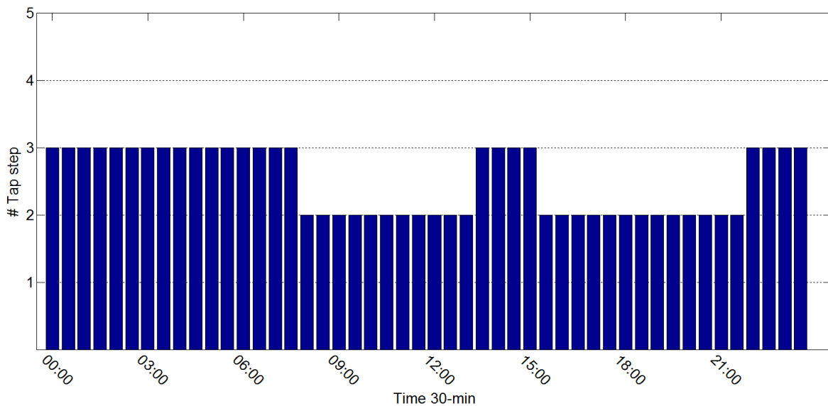
Figure 11 Potential number of tap changes for voltage reduction purposes in Romiley primary (3 rd September)
