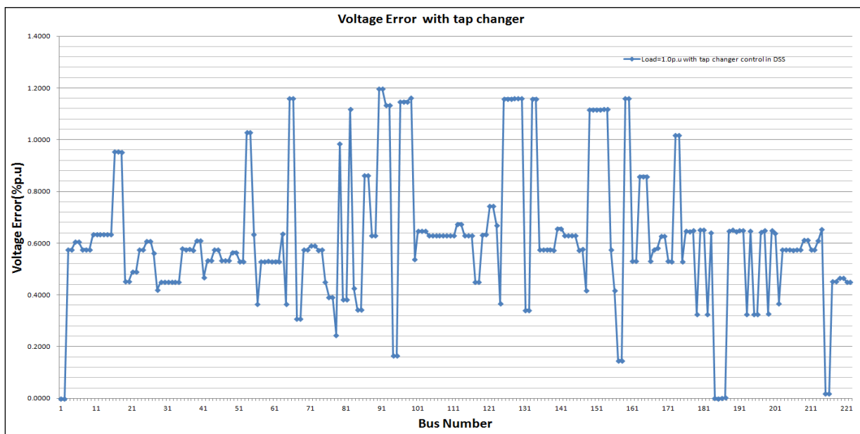
Figure 16: Validation results when AVC applies
