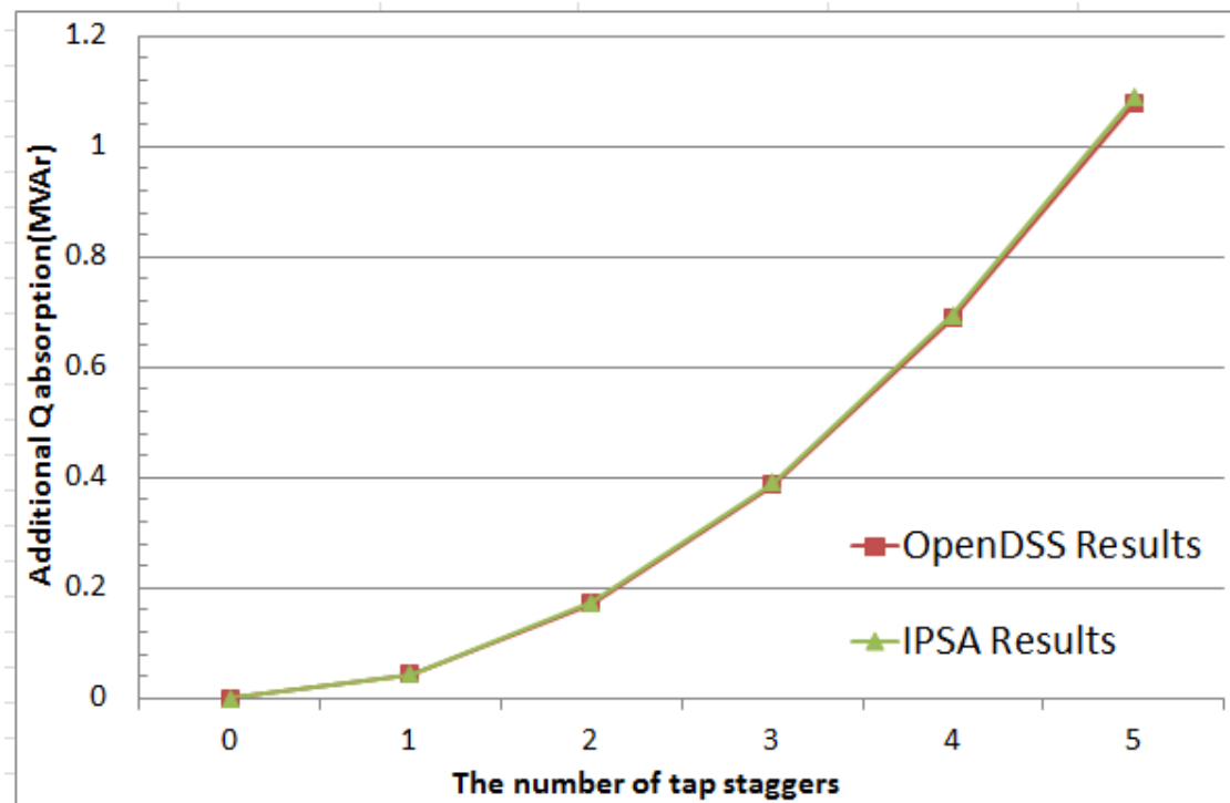
Fig.17(a): Additional reactive power absorption against the number of tap stagger
