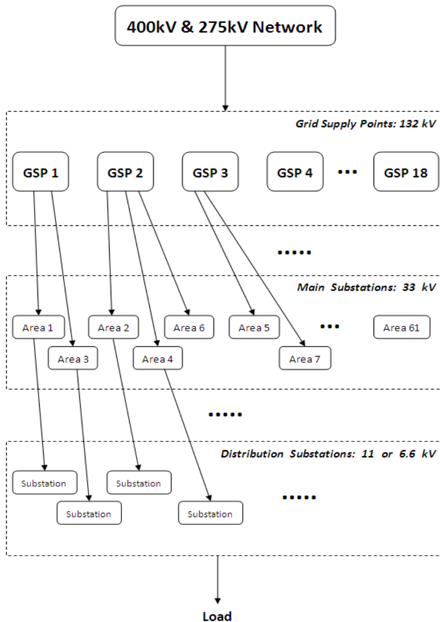
Figure21: The whole ENWL EHV networks
