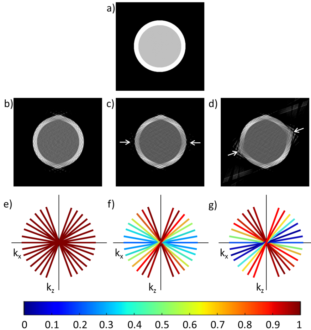
Figure 7. Demonstration of artefacts associated with variations in projection intensities. a) Simulated two-phase object to be reconstructed. b-d) Phantom images reconstructed from 15 simulated projections of the two phase image in (a) for a tilt range of \pm 70^\circ and angular intervals of 10^\circ . b) Reconstruction using projections of the same intensity, displaying missing wedge and streaking artefacts only. c) Reconstruction applying the intensity variations due to shadowing (measured when employing all 4 Super-X detectors with a single tilt tomography holder, as shown in Fig 2c). d) Reconstruction applying the intensity variations from only a pair of Super-X detectors on one axis, as shown in Fig 2b. (e-f) Representation in Fourier space of the projections used to reconstruct the images in (b-d) respectively. e) Constant intensity projections. f) Variable intensity projections weighted for the full Super-X detector geometry. g) Variable intensity projections weighted for one pair of Super-X detectors.
