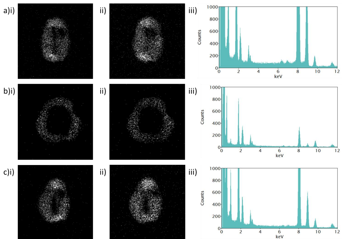
Figure 10. Projections at a) -60^\circ , b) 0^\circ and c) 60^\circ for i) Au L \alpha counts and ii) Ag L \alpha counts. iii) Spectra from the full spectrum images at a) -60^\circ , b) 0^\circ and c) 60^\circ .
