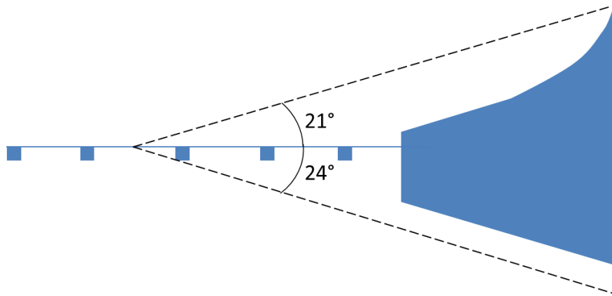
Figure 4. Schematic diagram showing the elevation angles from the sample at which the holder and grid bars will shadow emitted X-rays above and below the specimen in the direction of a single Super-X detector (45° azimuthal angle).
