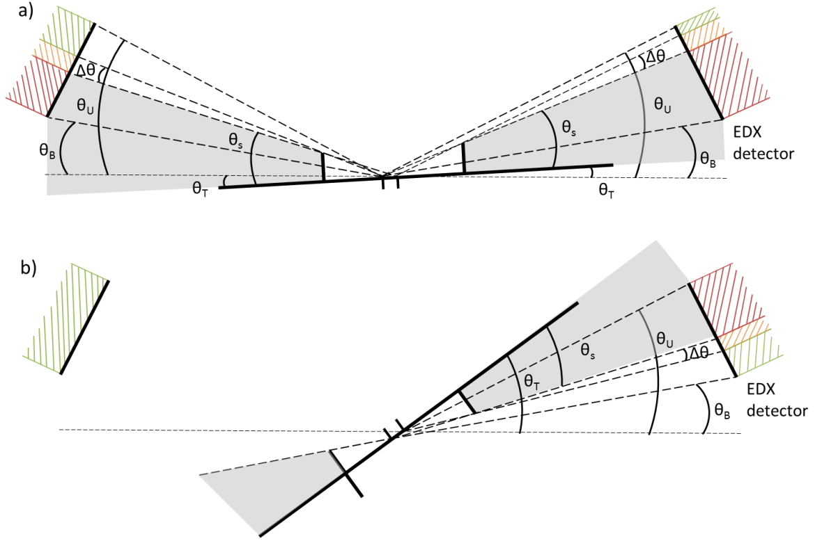
Figure 14. Diagram illustrating the geometry of angles used in determination of the extent of detector shadowing from (a) the top side of the sample holder and (b) the bottom side of sample holder (grid bars) .
