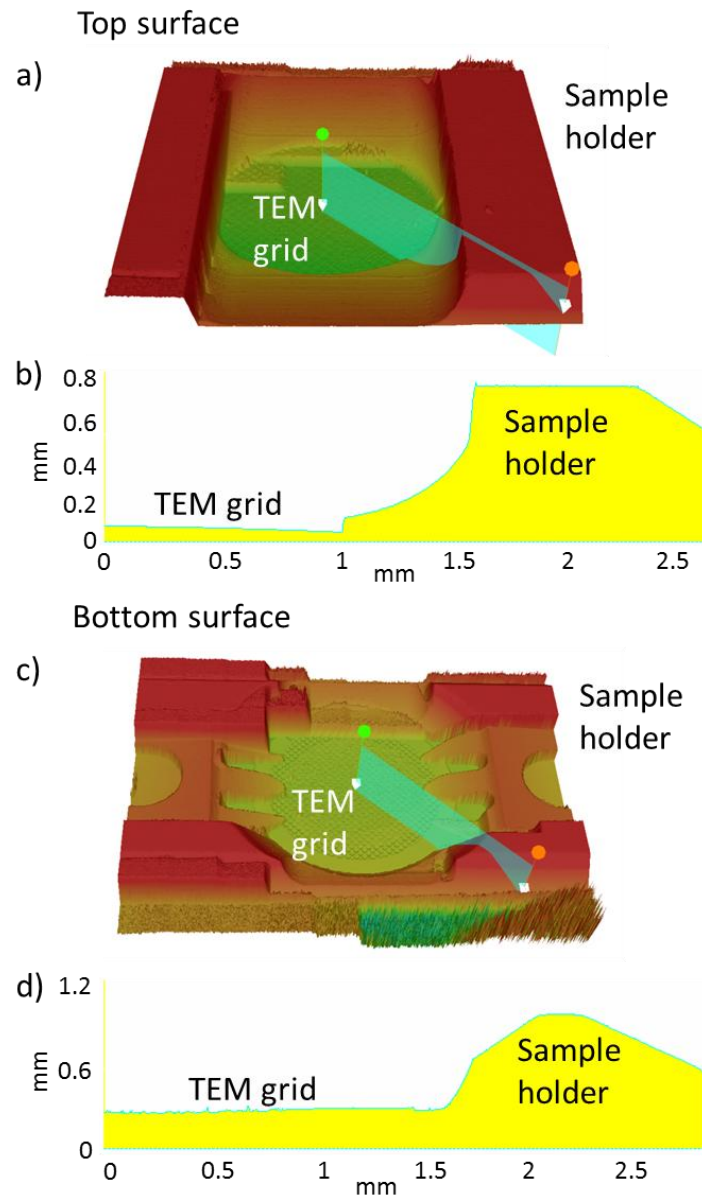
Figure 3. Optical profiles of the top and bottom surfaces of the Fischione 2020 holder. a) 3D profile of the top surface of the holder with the direction of line profile, b, illustrated. b) Line profile of plane indicated in a, displaying a polar angle of approximately 21^\circ from the centre of the grid to the highest point of the top surface of the holder. c) 3D profile of the bottom surface of the holder with
