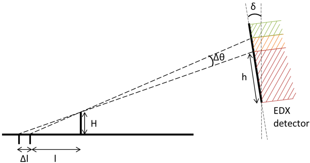
Figure 13. Diagram illustrating the variation in detector shadowing between two points on the sample separated by a distance \Delta l , shadowed by an object of height H at a distance l from the image area.
