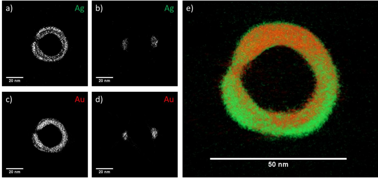
Figure 11. Example of a tomographic reconstruction using a time-dependent acquisition scheme performed for a AgAu nanoparticle. a) Orthoslice through the Ag reconstruction normal to the optic axis, displaying clear segregation of Ag to the surface of the nanoparticle. b) Orthoslice through the Ag reconstruction parallel to the optic axis. c) Orthoslice through the Au reconstruction normal to the optic axis. d) Orthoslice through the Au reconstruction parallel to the optic axis. e) Volume rendering of the Ag and Au reconstructions, Ag volume is green and Au volume is red.
