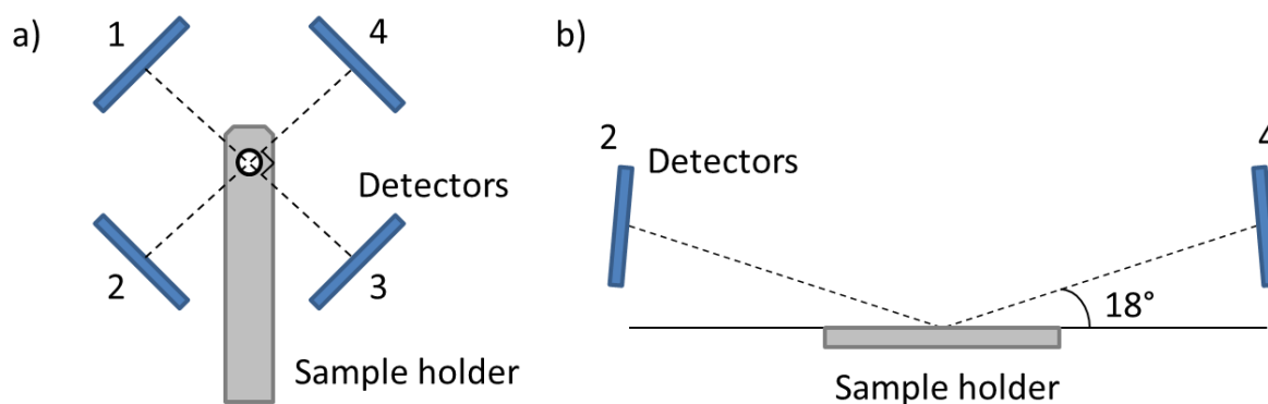
Figure 1. Schematic illustrating the geometry of the Super-X detectors in the FEI Titan G2 80-200 (S)TEM. (a) viewed in the direction of the electron beam and (b) viewed for a 2D cross-section passing through detectors 2 and 4 at 45° to the long axis of the specimen holder. Detectors are labelled 1-4 as used in FEI TIA software.
