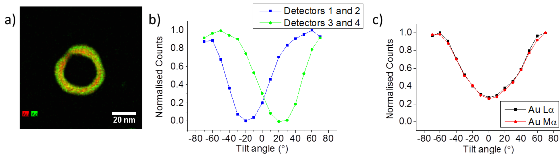
Figure 2. Calibration of Super-X detector shadowing in the Titan G2 for the Fischione 2020 single tilt tomography holder. a) EDX Au and Ag elemental map for a single AgAu nanoparticle at 0 degrees showing the particle that was used to perform the detector shadowing calibration, b) background subtracted Au L \alpha X-ray counts (9.7 keV) at each pair of detectors as a function of tilt angle, taken from EDX spectrum images acquired for the same AgAu nanoparticle using an acquisition time of 5 mins, 10° tilt increments and an angular range of \pm 70^\circ , c) background-subtracted summed X-ray counts for Au L \alpha (9.7 keV) and Au M \alpha (2.1 keV) peaks.
