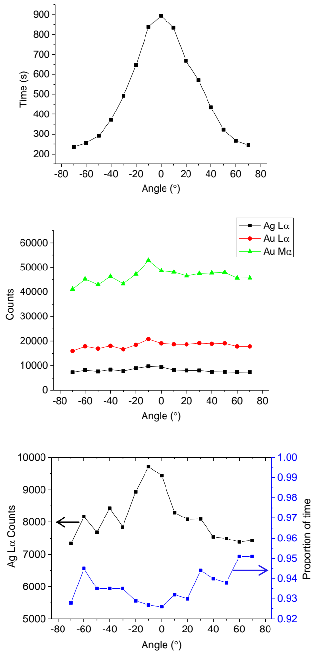
Figure 8. a) Total acquisition time at each angle employed in the time-varied acquisition scheme reported in this study. b) Au L \alpha , Au M \alpha and Ag L \alpha X-ray counts at each specimen tilt angle under the varied acquisition time scheme. The variation in counts of each elemental peak using the time-varied acquisition scheme are significantly reduced (variation < \pm 15\% ). c) Comparison of Ag L \alpha counts at each specimen tilt angle and to the proportion of the calibrated time the acquisition actually took.
