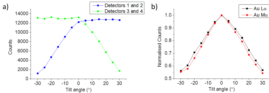
Figure 6. Calibration of Super-X detector shadowing in the Titan G2 for the FEI high-visibility low-background double tilt holder using a similar particle to that shown in Fig 2a. a) Au L \alpha counts at each pair of detectors as a function of tilt angle, b) background-subtracted Au L \alpha (9.7 keV) and Au M \alpha (2.1 keV) X-ray counts extracted from EDX spectrum images acquired for the same AgAu nanoparticle using an acquisition time of 5 mins and 5° tilt increments for angles of \pm 30^\circ .
