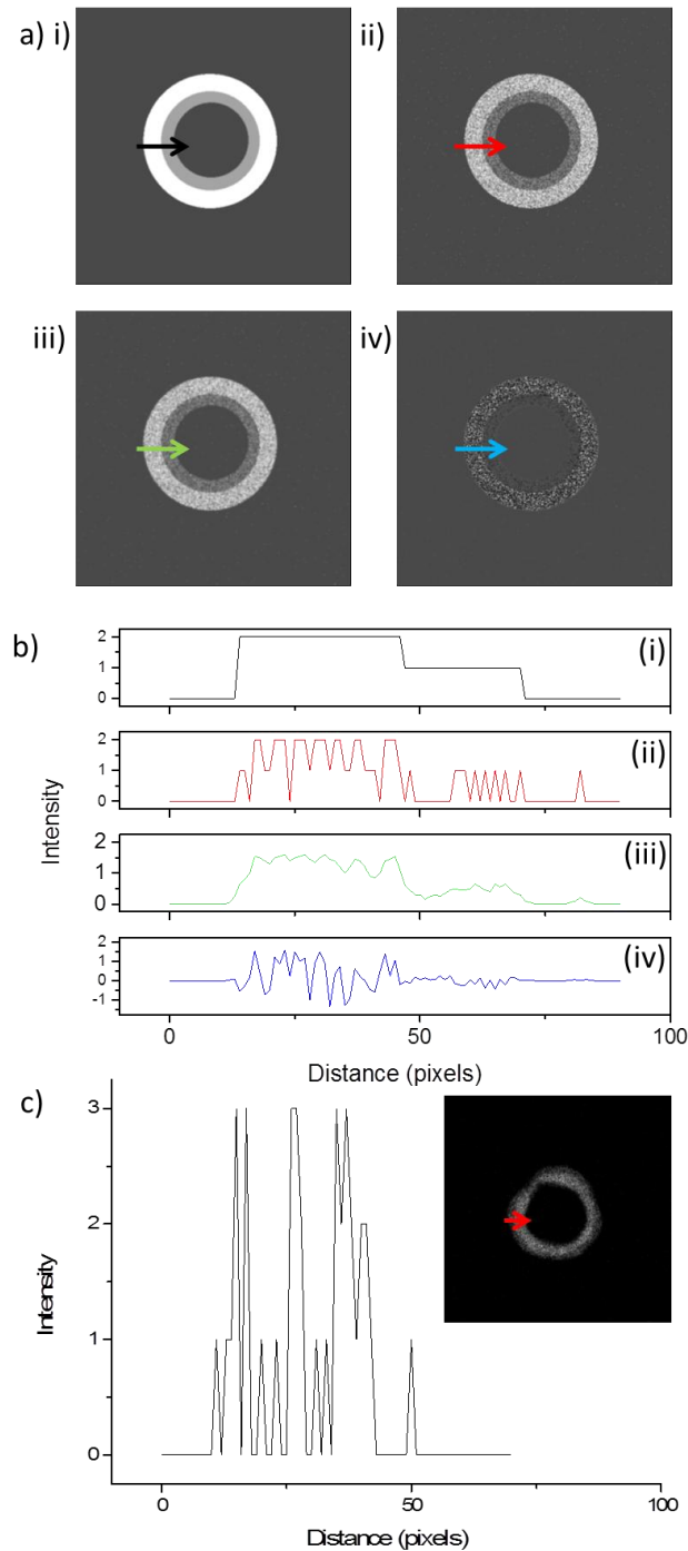
Figure 9. Producing a simulated EDX elemental map which closely resembles the experimental data. a) i) Initial test image of object representing a two phase nanoparticle. ii) Simulated elemental maps in which 30% of data points have been set to zero and Poisson noise added. iii) Image b processed with 5-pixel smoothing window showing effective suppression of noise in the image. iv) Image b processed with an edge preserving filter demonstrating the appearance of negative intensity artefacts within the nanoparticle. All images are shown with the same intensity scale and are 512x512 pixels. b) Line profiles (i-iv) through the images (a(i-iv)) respectively at the positions indicated by the arrows. c) Line profile taken from representative experimental dataset with the corresponding Au L \alpha map of an AgAu nanoparticle shown inset.
