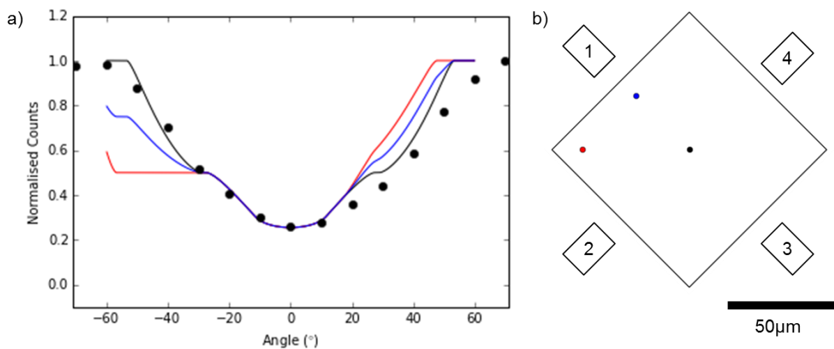
Figure 5. Modelling detector shadowing using the model of Yeoh et al [23]. a) Plot of normalised counts with respect to tilt angle for the positions within a grid square indicated in (b). Experimental data points for Au L \alpha (9.7 keV) X-rays (reproduced from Fig 2c) are also shown (black dots) for reference b) Diagram indicating nanoparticle position within a 90 \mu\text{m} x 90 \mu\text{m} grid square with black in the centre, blue 10 \mu\text{m} from the edge towards detector 1 and 45 \mu\text{m} from the edge towards detector 2 and red 10 \mu\text{m} from both edges towards detector 1 and detector 2.
