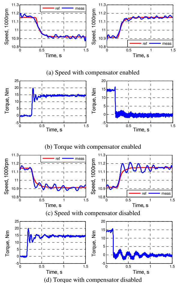
Figure 3. Emulation performance for the small inertia system (0.0187kgm 2 )
