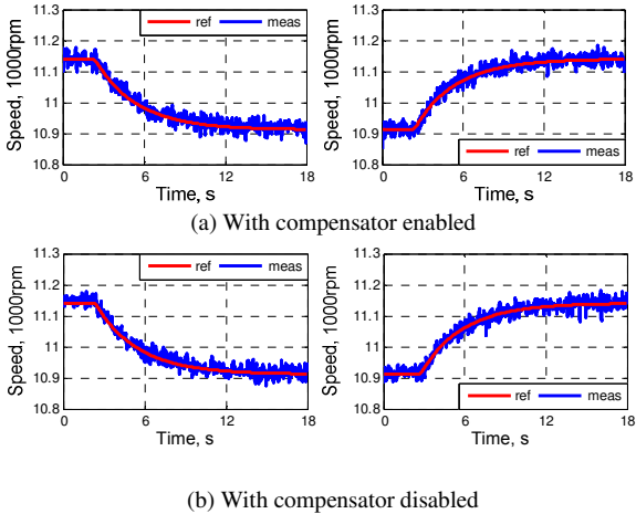
Figure 5. Emulation performance for the large inertia system ( 1.87\text{kgm}^2 ).
