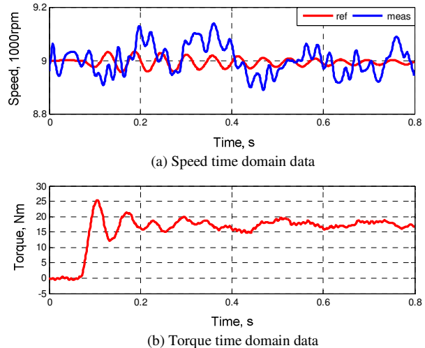
Figure 8. Key waveforms for the resonant mode of 12Hz in the mechanical drivetrain with the compensator enabled.
