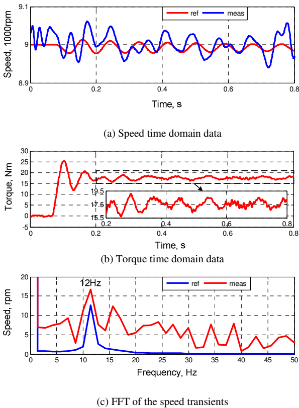
Figure 8. Key waveforms for the resonant mode of 12Hz in the mechanical drivetrain with the compensator enabled.
