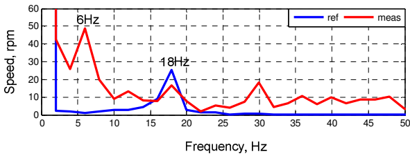
(c) FFT of the speed transients
