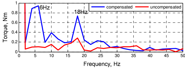
Figure 11. FFT of 18Hz resonance torque transients for the 0.7s time window after the electrical power step.
