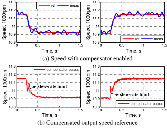
Figure 4. Emulation performance for the limiting inertia system ( 0.011\text{kgm}^2 ) with the compensator enabled.
