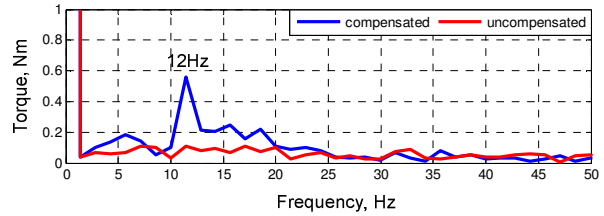
Figure 9. FFT of 12Hz resonance torque transients for the 0.7s time window after the electrical power step.
