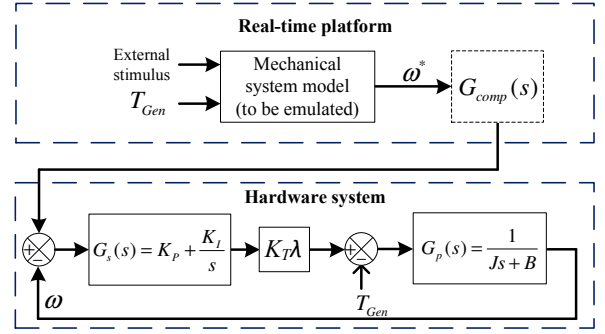
Figure 2. Block diagram of the compensator implementation. The speed control loop dynamics compensator can be determined analytically [10] using the theoretical transfer function of the speed controller, providing the parameters are known and there is no variation in response with operating point. However, not all of the system parameters in Fig. 2 are known, more specifically communication and microcontroller delays, and ADC/DAC conversion circuits are unknown, so the analytical compensator method is not suitable.
