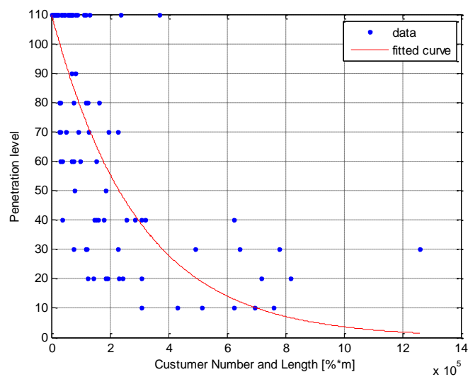
Figure 85: Customer Number and Feeder Length for the PV Case, R^2:0.63
