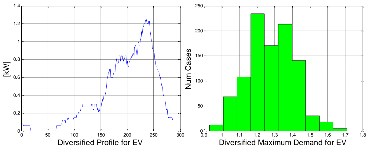
Figure 19: Diversified Profile and Maximum Demand Histogram for 100 EV profiles – Shifted Case
