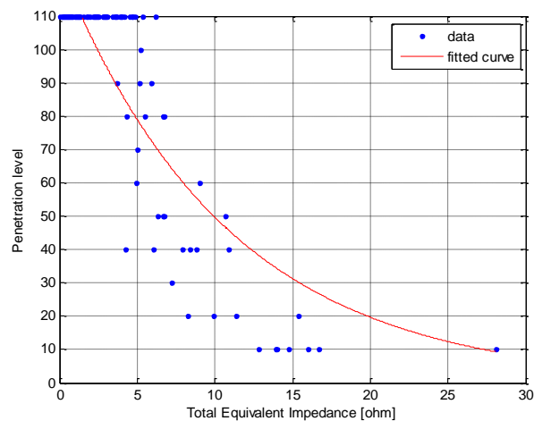
Figure 79: Total Path Impedance, R^2:0.75 – EV Shifted Case
