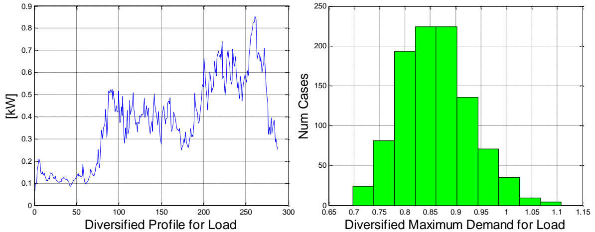
Figure 13: Diversified Profile and Maximum Demand Histogram for 100 load profiles
