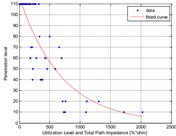
Figure 82: Initial Utilization Level and Total Path Impedance for the EV Case, R^2:0.79
