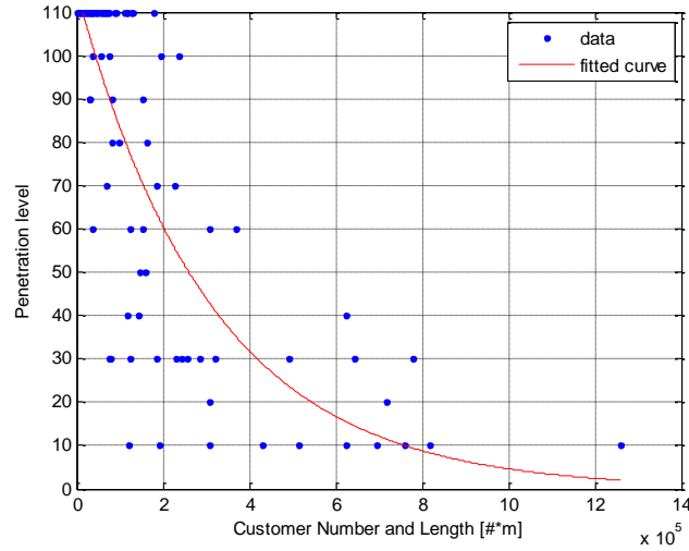
Figure 86: Customer Number and Feeder Length for the EHP Case, R^2:0.70
