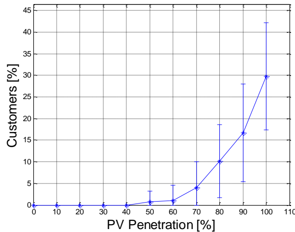
Figure 43: Voltage problems by using the ELEXON profile
