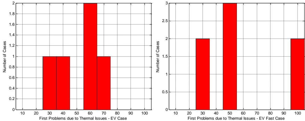
Figure 60: Histograms of First Penetration Level with Thermal Problems – EV and EV fast charging Cases
