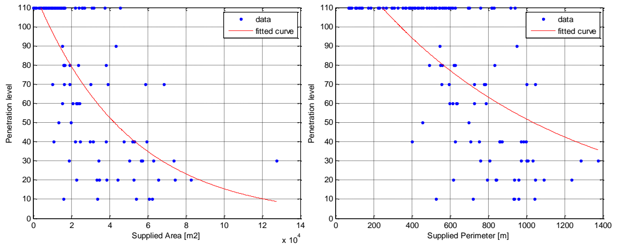
Figure 66: Supplied Area (left), R^2:0.56 and Supplied Perimeter (right), R^2:0.45 – PV Case
