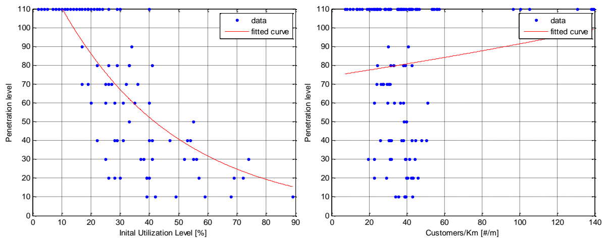
Figure 64: Initial utilization level (left), R^2 :0.65 and Customers per km. (right), R^2 :0.01 – PV Case
