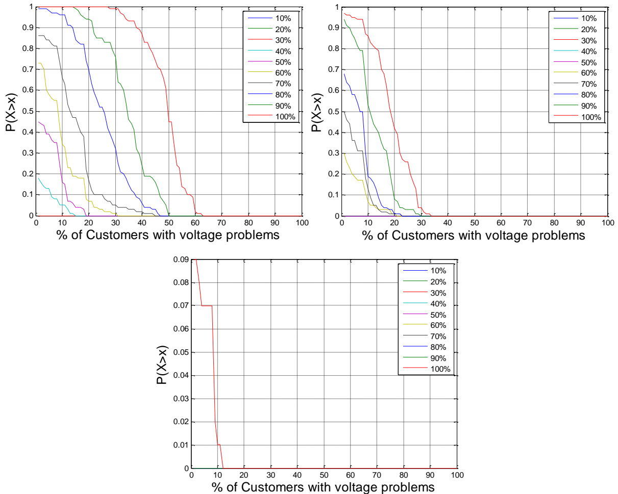
Figure 32: Example of probabilities to have at least X% of customers with problems: PV case (top-left), EHP case (top-right) and EV case (centre-down)
