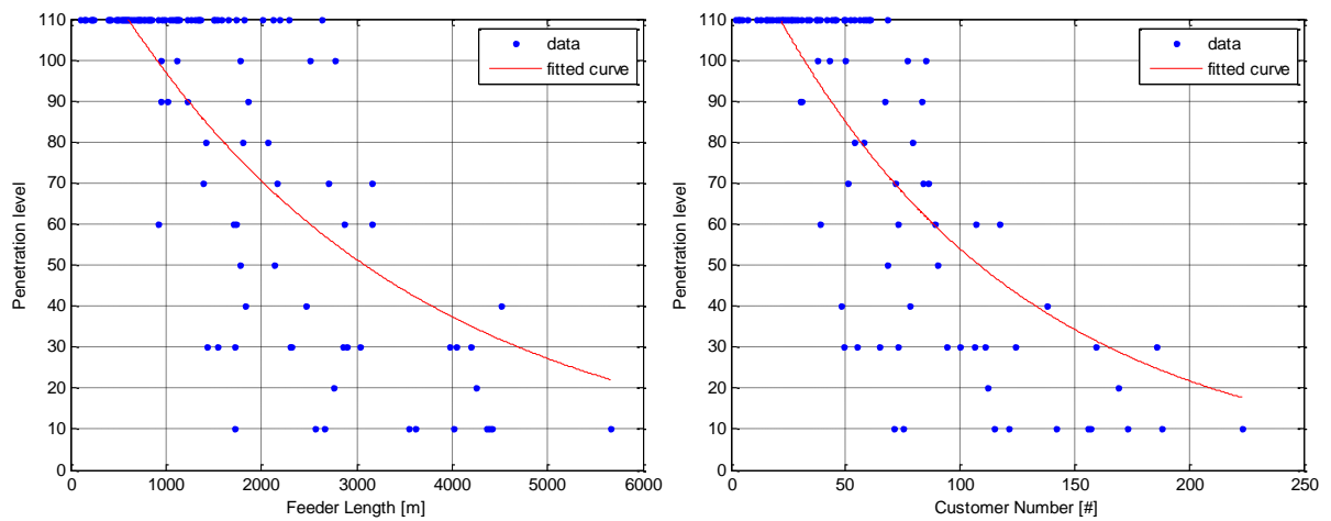
Figure 68: Feeder Length (left), R^2 :0.59 and Customer Number (right), R^2 :0.65 – EHP Case
