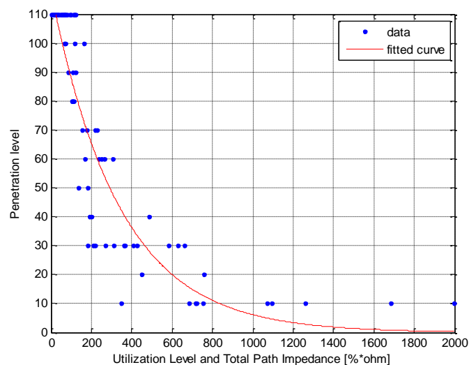
Figure 81: Initial Utilization Level and Total Path Impedance for the EHP Case, R^2:0.88
