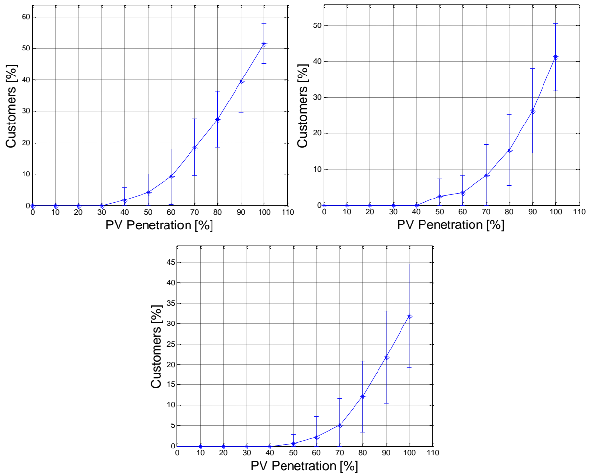
Figure 41: Voltage problems Comparison: Case 1 (top-left), Case 2 (top-right) and Case 3 (centre-down)
