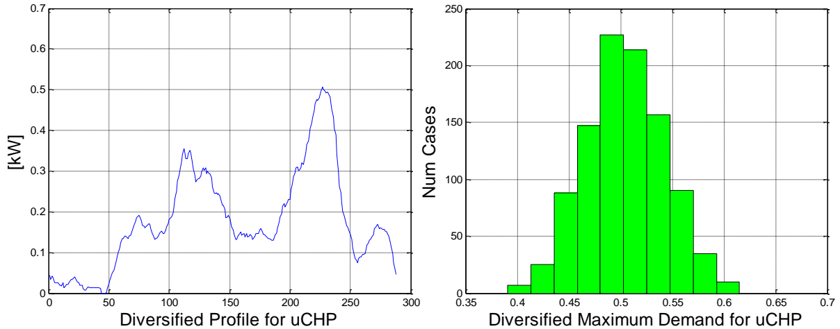
Figure 16: Diversified Profile and Maximum Demand Histogram for 100 \mu CHP profiles
