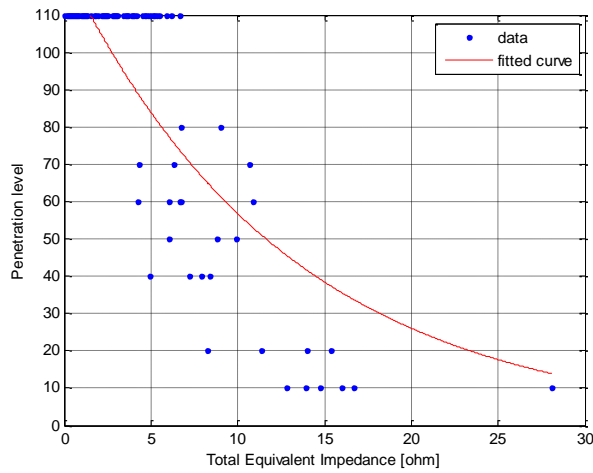
Figure 73: Total Path Impedance, R^2:0.70 – EV Base Case
