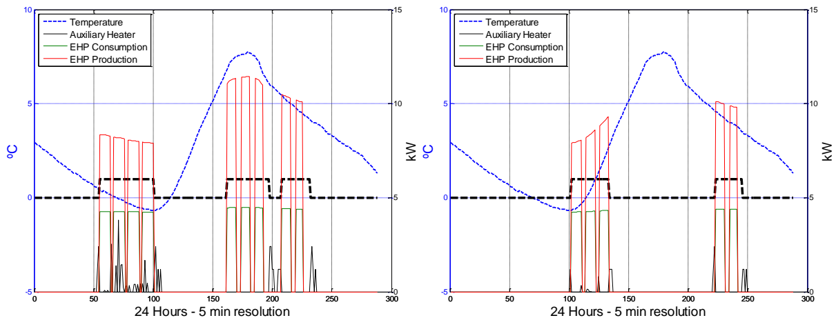
Figure 8: Example of EHP and auxiliary heater profiles for two different houses
