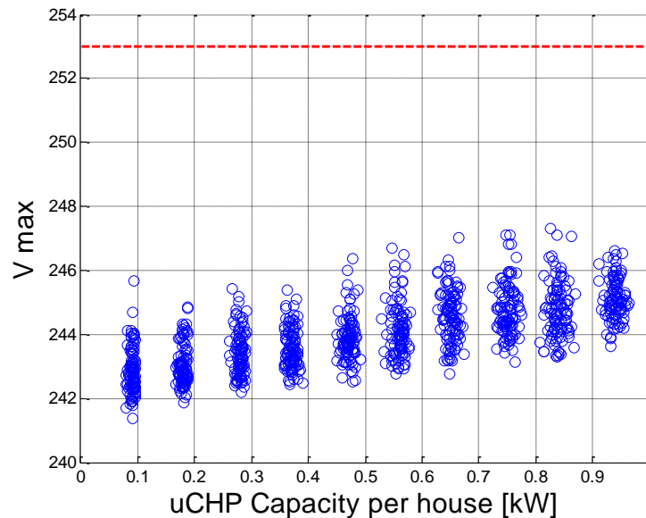
Figure 34: Maximum voltage per Average DG capacity – \mu CHP Case
