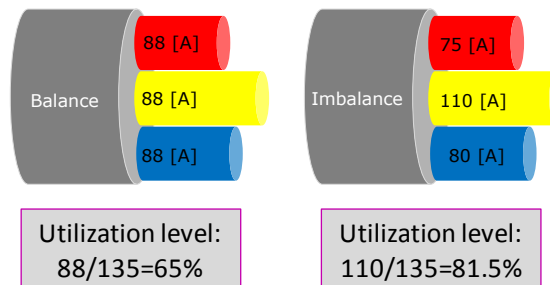
Figure 38: Calculation of the utilization level - Example
