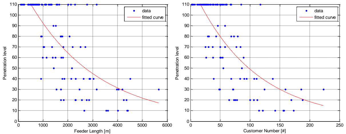
Figure 63: Feeder Length (left), R^2 :0.60 and Customer Number (right), R^2 :0.59 – PV Case
