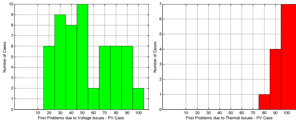
Figure 53: Histograms of First Penetration Level with Technical Problems – PV Case
