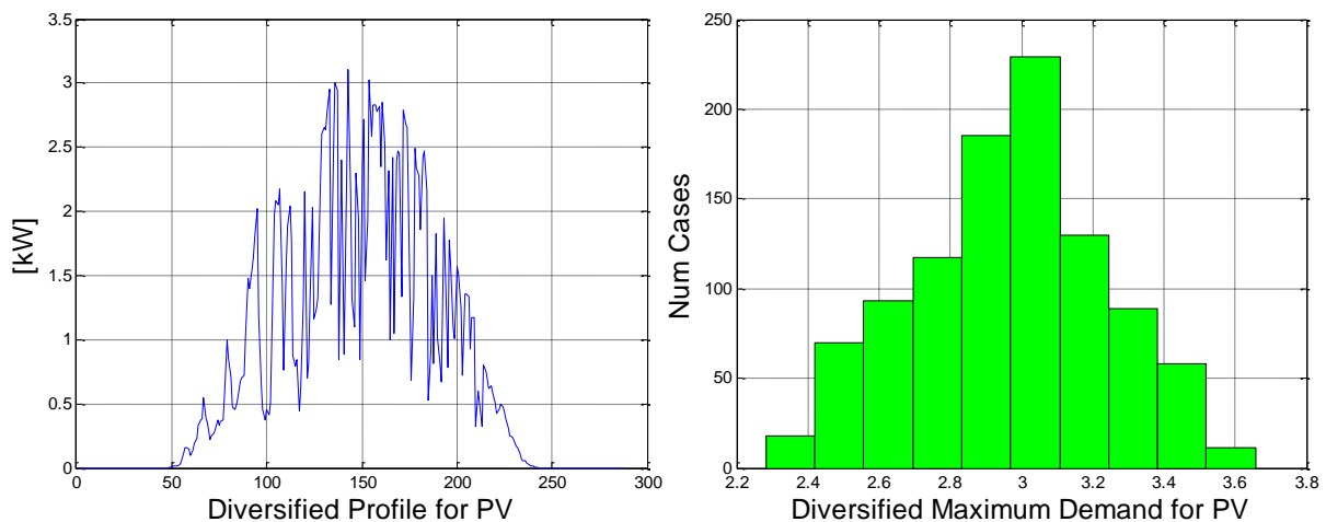
Figure 17: Diversified Profile and Maximum Demand Histogram for 100 PV profiles
