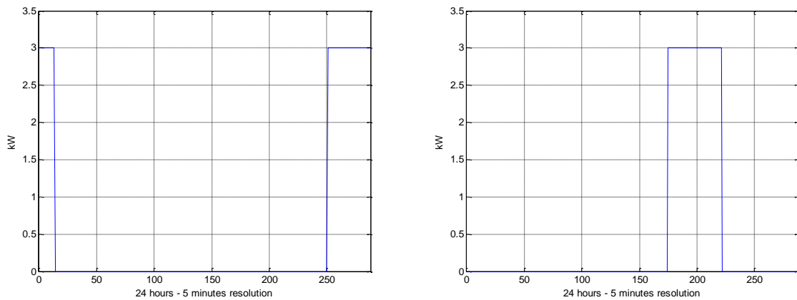
Figure 11: Example of individual EV profiles
