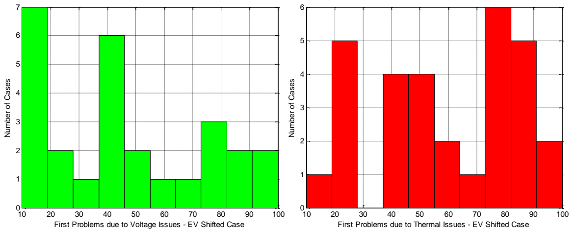
Figure 57: Histograms of First Penetration Level with Technical Problems – EV Shifted Case
