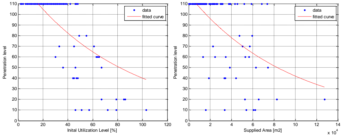
Figure 72: Initial Utilization Level (left), R^2:0.53 and Supplied Area (right), R^2:0.38 – EV Base Case
