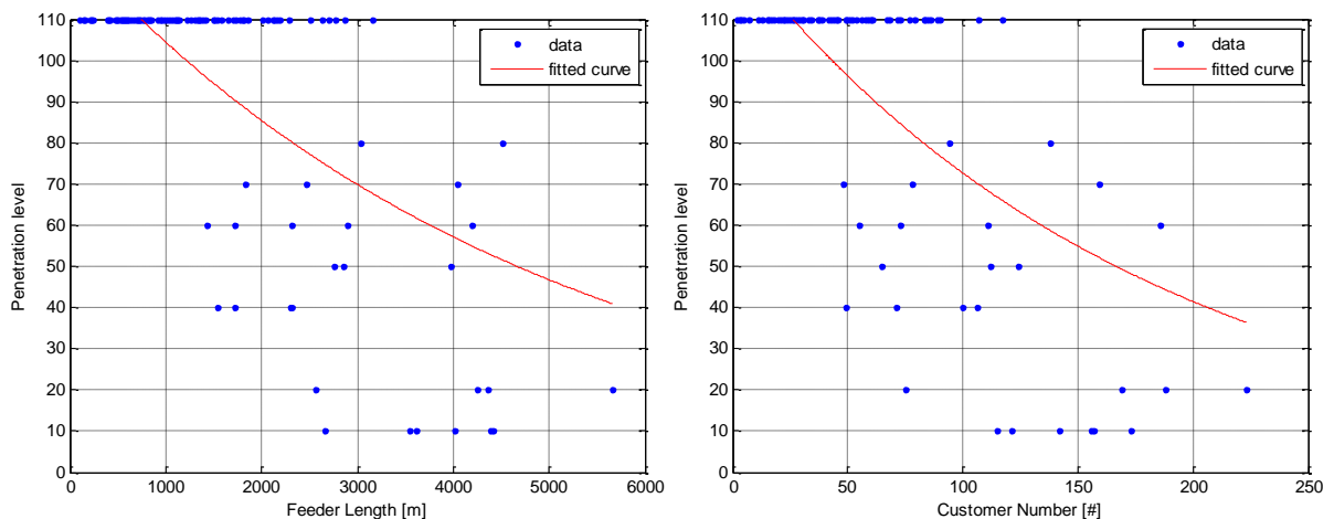
Figure 71: Feeder Length (left), R^2=0.47 and Customer Number (right), R^2=0.51 – EV Base Case
