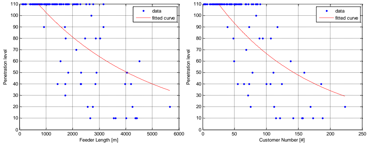
Figure 77: Feeder Length (left), R^2:0.52 and Customer Number (right), R^2:0.58 – EV Shifted Case
