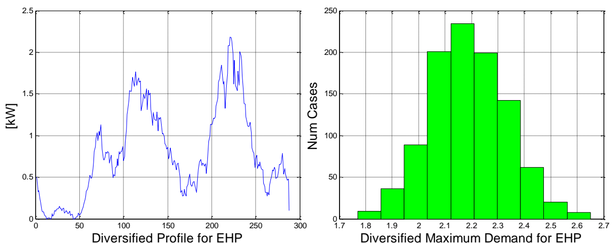
Figure 15: Diversified Profile and Maximum Demand Histogram for 100 EHP profiles
