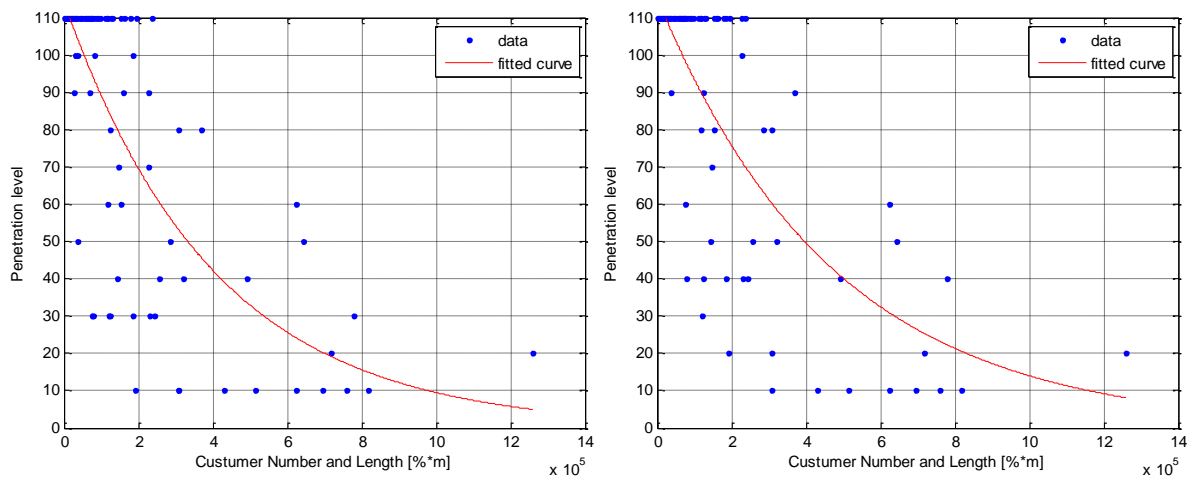
Figure 88: Customer Number and Feeder Length for the EV fast charging (left) and peak shifted (right), R^2:0.63 and R^2:0.66 , respectively.
