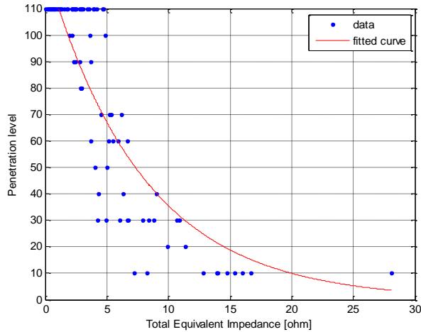
Figure 70: Total Path Impedance, R^2=0.78 – EHP Case
