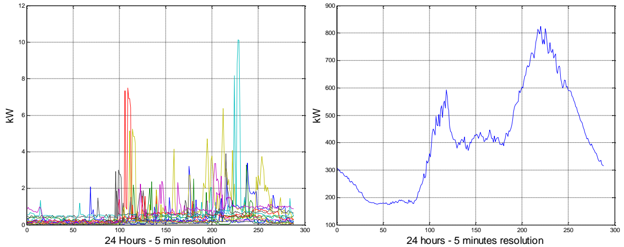
Figure 6: Individual (left) and aggregated (right) electricity load profiles
