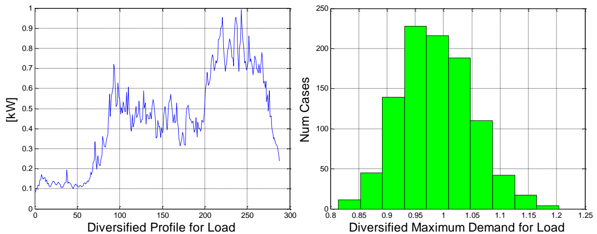
Figure 12: Diversified Profile and Maximum Demand Histogram for 100 winter load profiles
