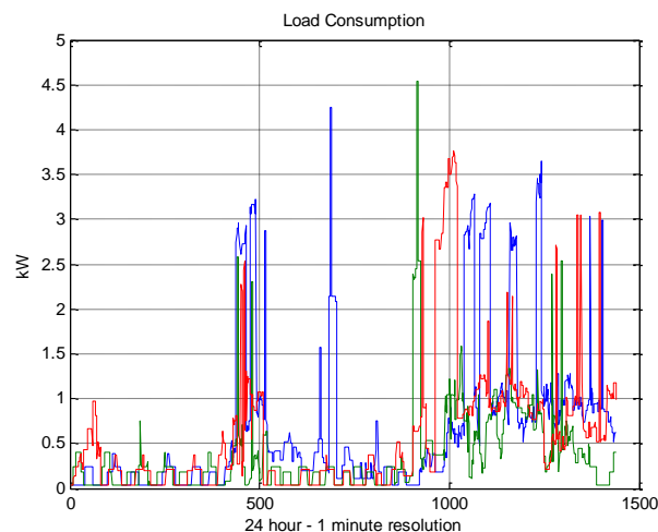
Figure 1: Individual load profiles – 1 minute resolution
