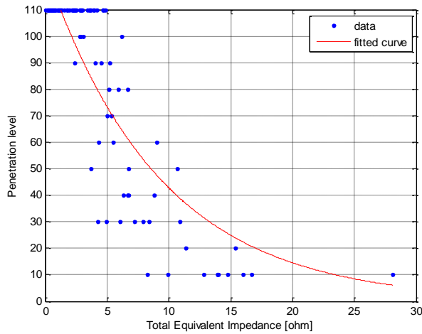
Figure 76: Total Path Impedance, R^2:0.75 – EV Fast Charging Case
