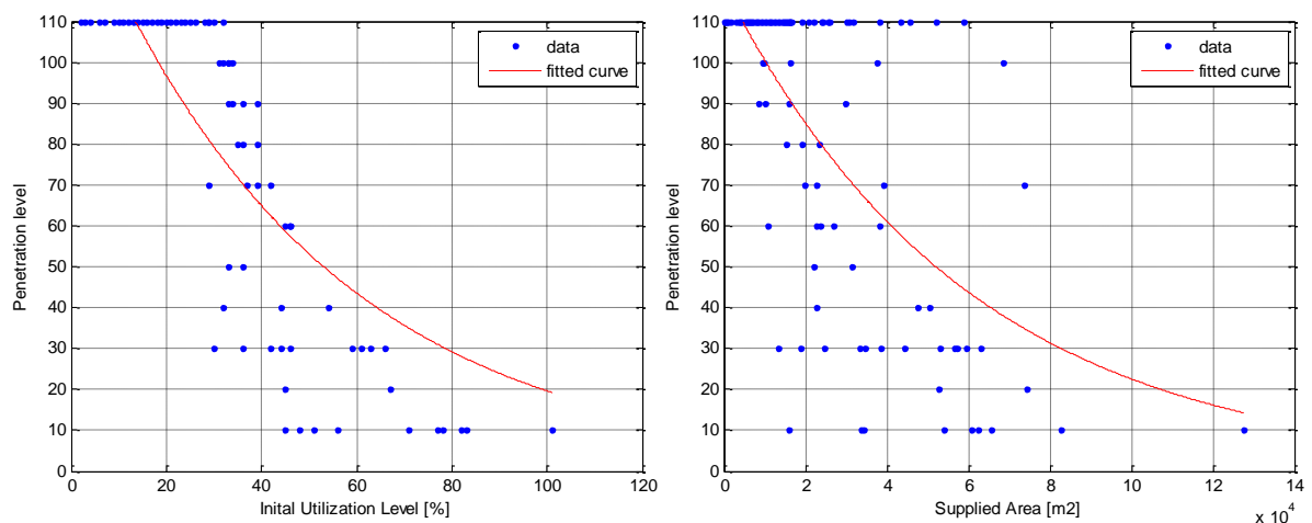
Figure 69: Initial Utilization Level (left), R^2 :0.70 and Supplied Area (right), R^2 :0.48 – EHP Case
