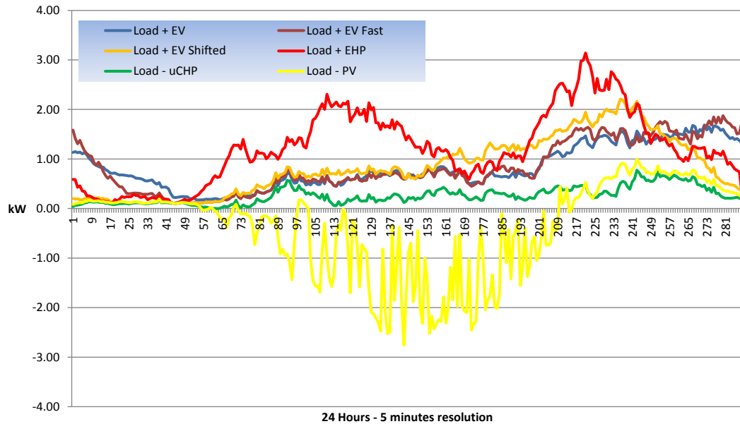
Figure 20: Comparison of diversified net profiles for different low carbon technologies
