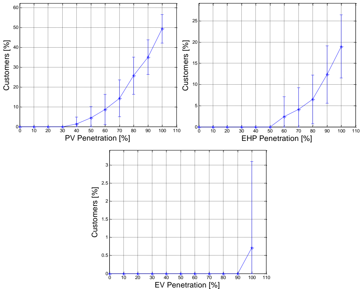
Figure 28: Example of customer voltage analysis for each technology
