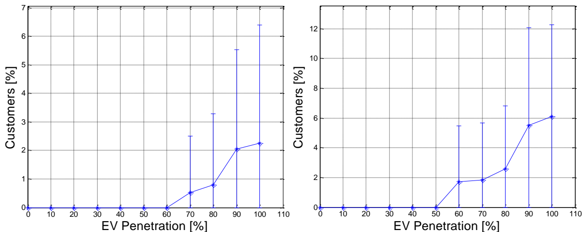
Figure 45: Percentage of customers with voltage problems for the EV case: EV shifted (left) and EV fast charging (right)
