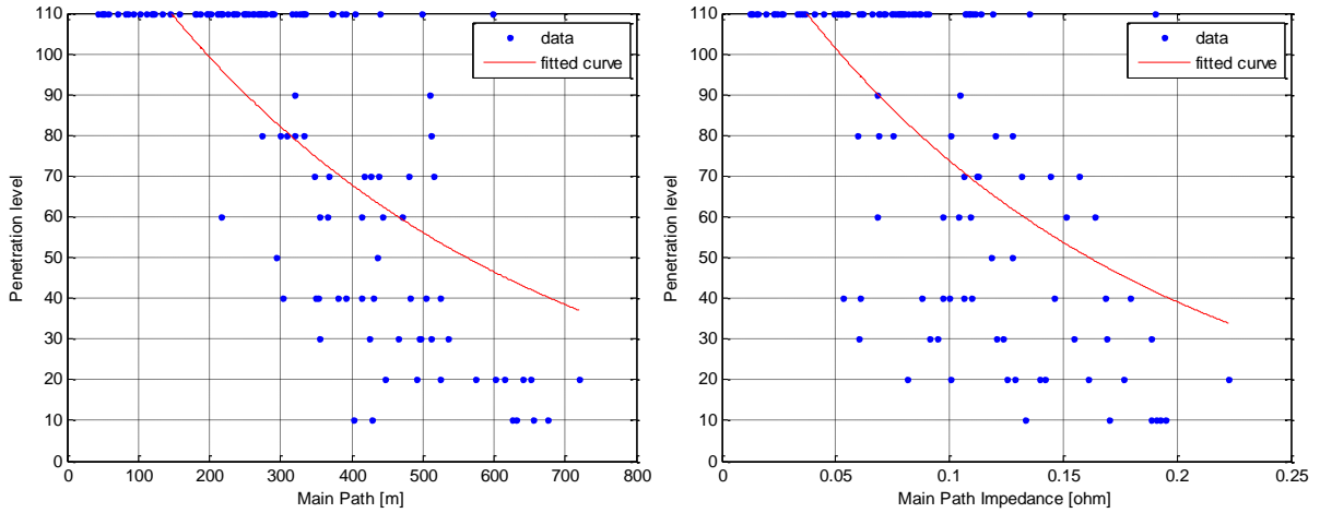
Figure 65: Main Path (left), R^2:0.50 and Main Path Impedance (right), R^2:0.43 – PV Case
