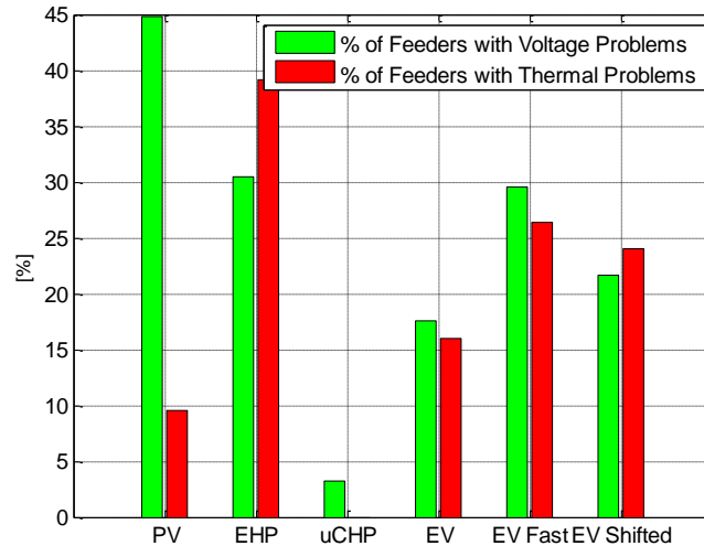
Figure 50: Feeders with technical problems per technology (any number of customers)
