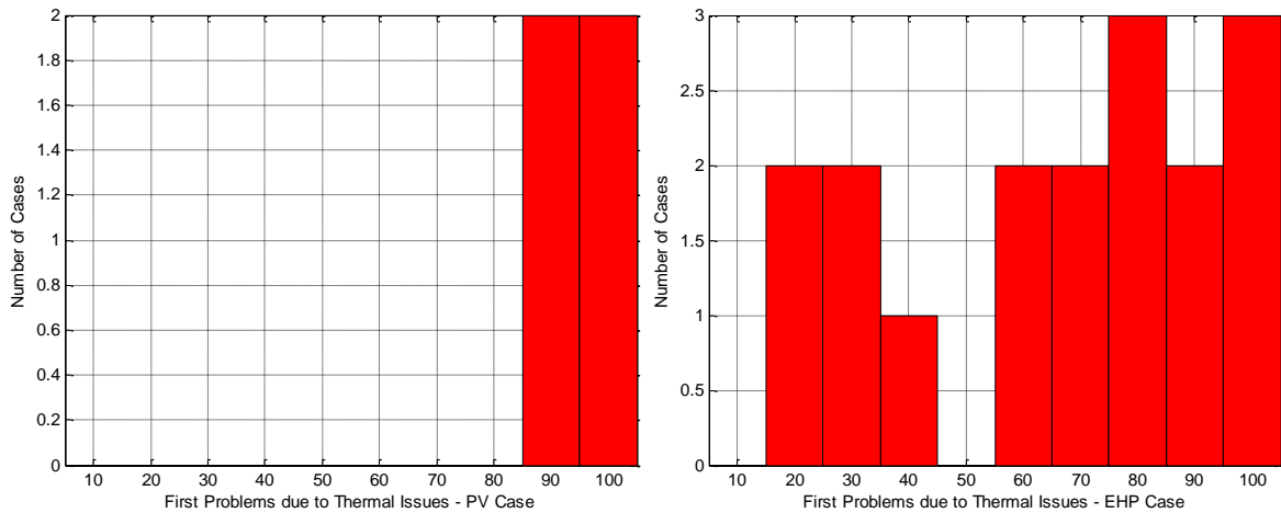
Figure 59: Histograms of First Penetration Level with Thermal Problems – PV and EHP Cases
