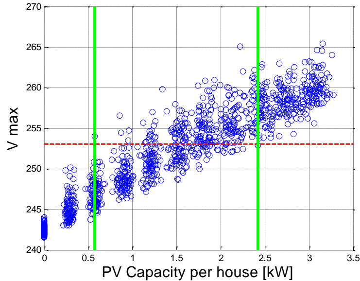
Figure 33: Example of maximum voltage per average DG capacity – PV Case
