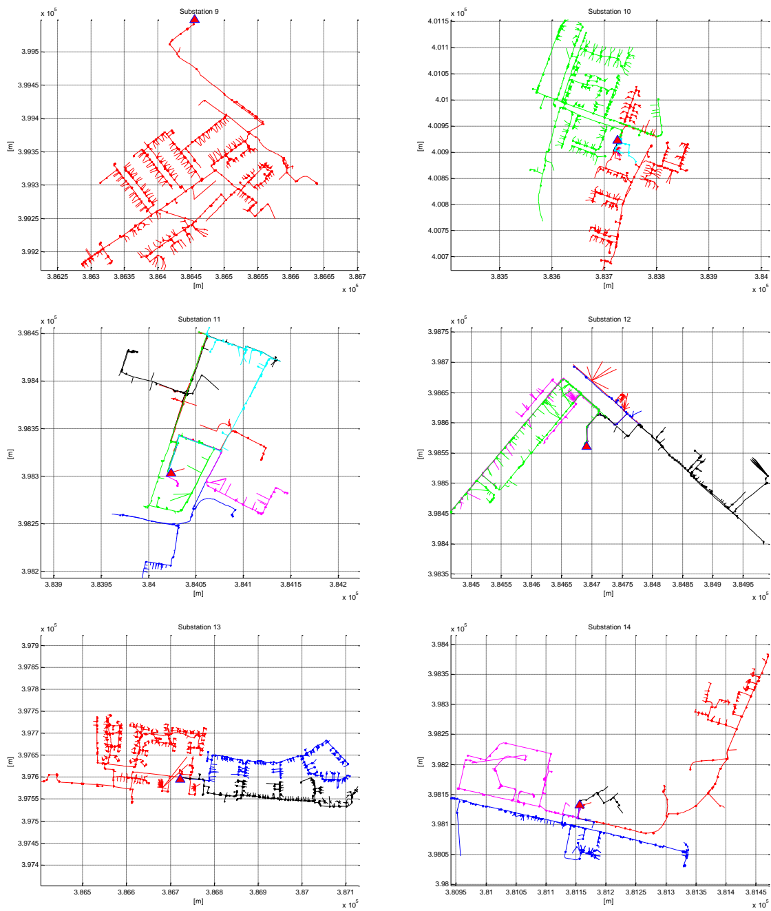
Figure 23: LV Networks 9-14
