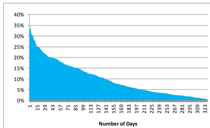
Figure 3: Capacity Factor
