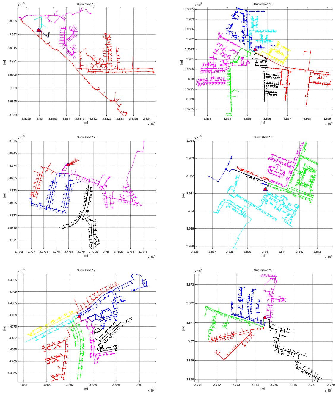
Figure 24: LV Networks 15-20
