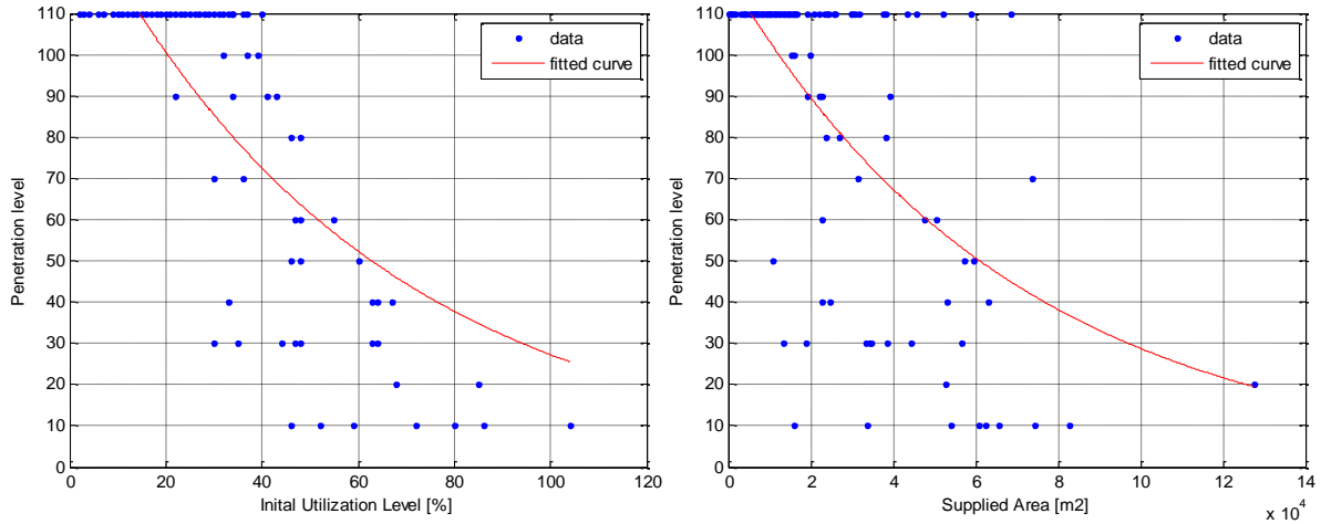
Figure 75: Initial Utilization Level (left), R^2:0.62 and Supplied Area (right), R^2:0.44 – EV Fast Charging Case
