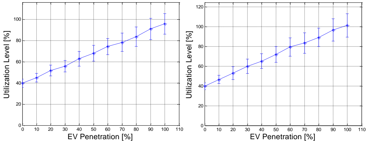
Figure 46: Utilization level at the head of the feeder for the EV case: EV shifted (left) and EV fast charging (right)
