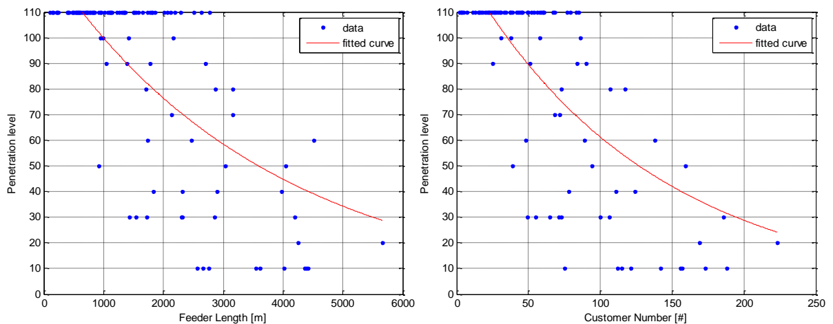
Figure 74: Feeder Length (left), R^2:0.52 and Customer Number (right), R^2:0.57 – EV Fast Charging Case
