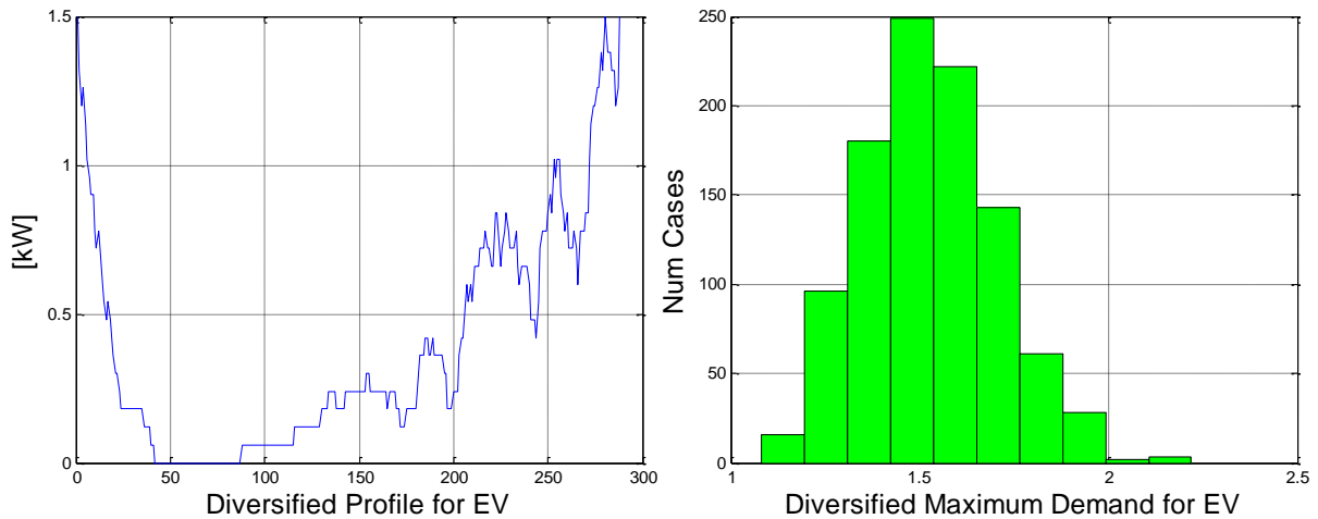
Figure 18: Diversified Profile and Maximum Demand Histogram for 100 Fast Charging EV profiles
