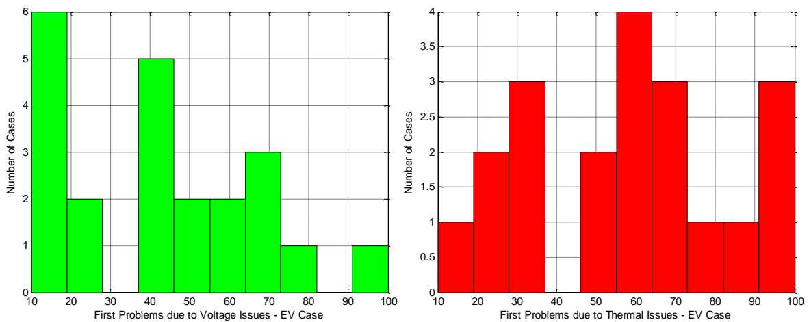
Figure 55: Histograms of First Penetration Level with Technical Problems – EV Case
