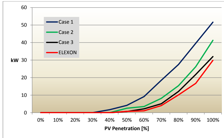
Figure 44: Average problems for the four cases analysed
