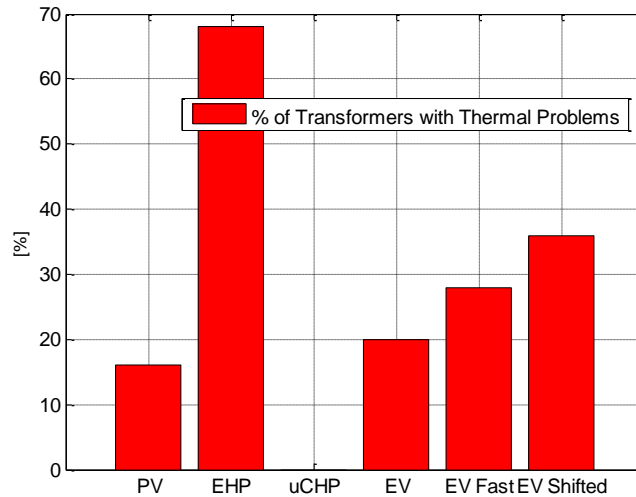
Figure 58: Transformers with thermal problems per technology
