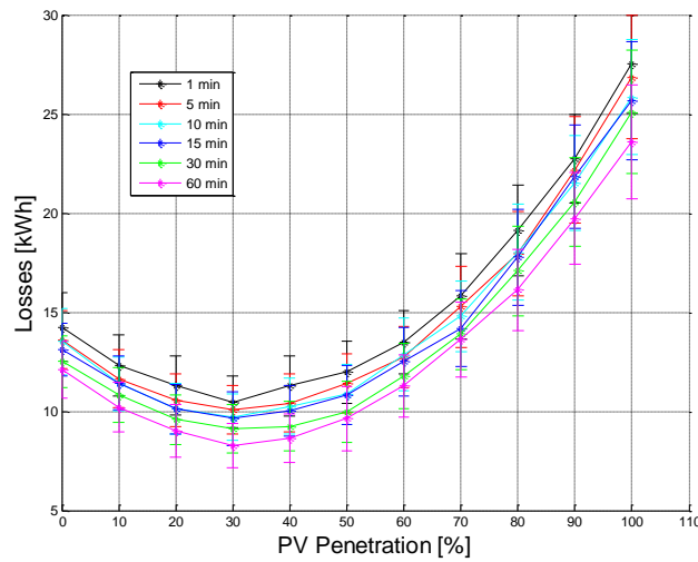
Figure 39: Daily energy losses – Data granularity
