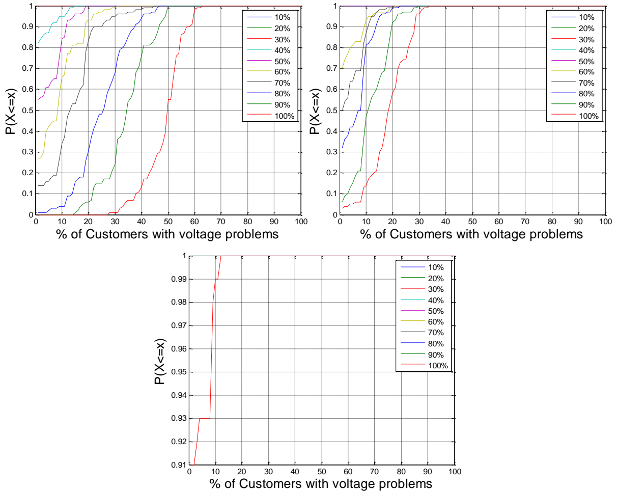
Figure 31: Example of probabilities to have at most X% of customers with problems: PV case (top-left), EHP case (top-right) and EV case (centre-down)
