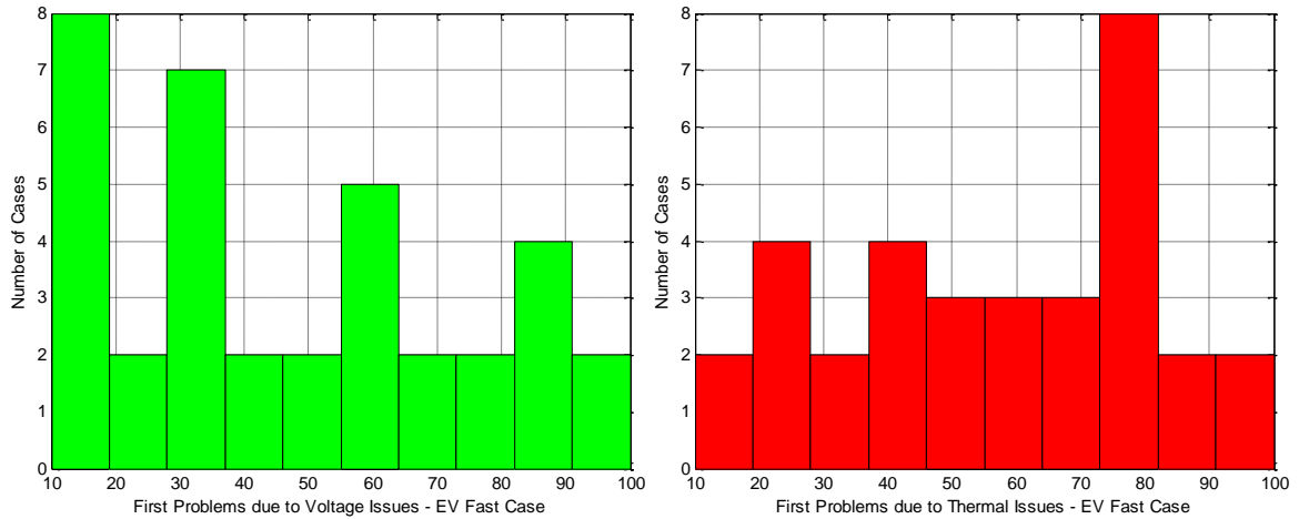
Figure 56: Histograms of First Penetration Level with Technical Problems – EV Fast Charging Case
