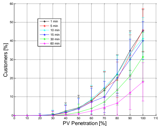
Figure 40: Voltage problems - Data granularity
