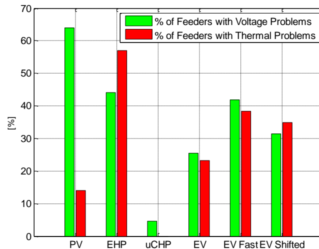
Figure 51: Feeders with technical problems per technology (more than 25 customers)
