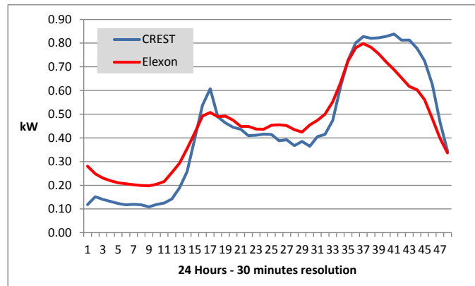
Figure 42: Diversified profile used in Case 3 (CREST) and closest ELEXON profile
