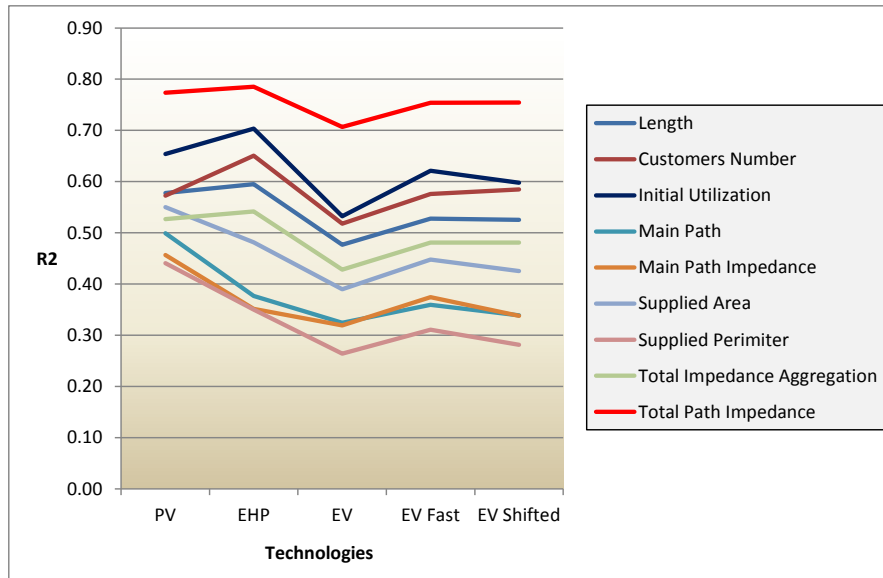
Figure 84: Coefficient of determination per metric and technology
