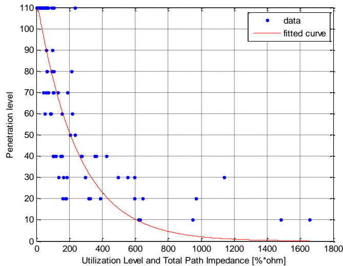
Figure 80: Initial Utilization Level and Total Path Impedance for the PV Case, R^2:0.80
