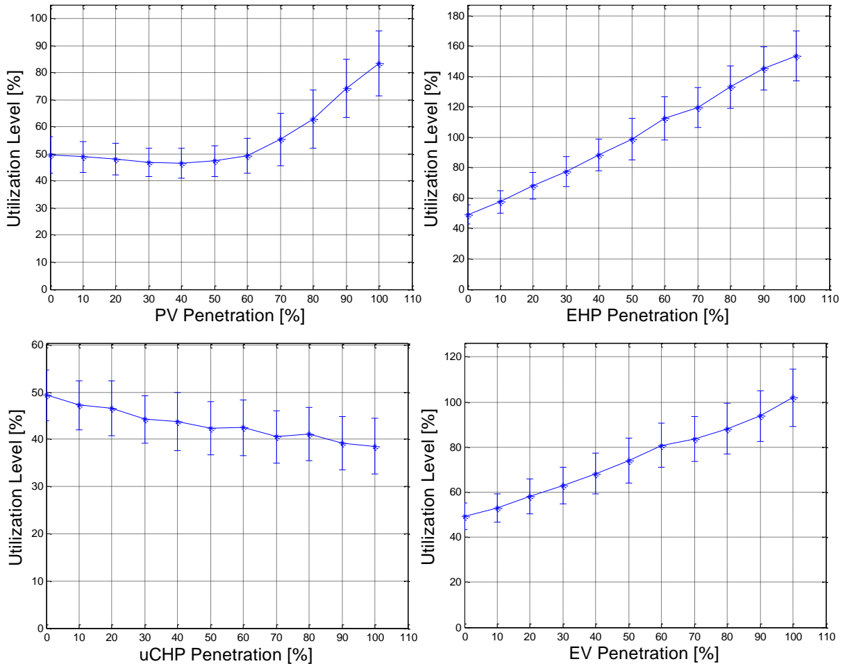
Figure 49: Utilization Level at the head of the feeder per technology
