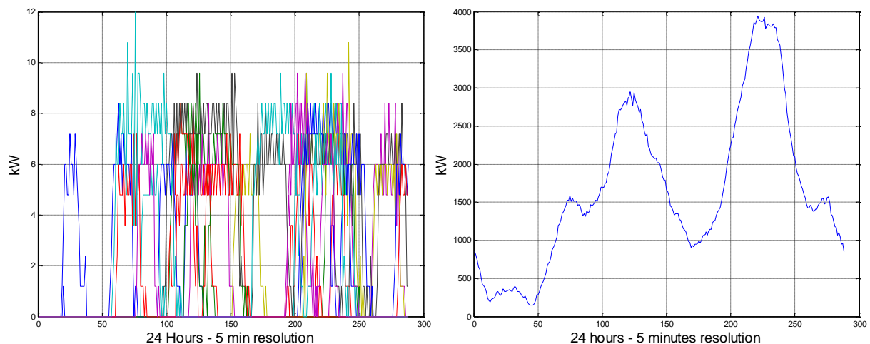
Figure 7: Individual (left) and aggregated (right) thermal load profiles
