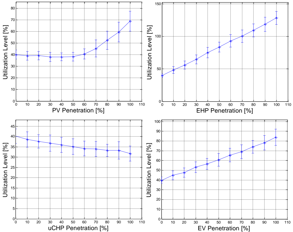
Figure 29: Example of feeder utilization for each technology
