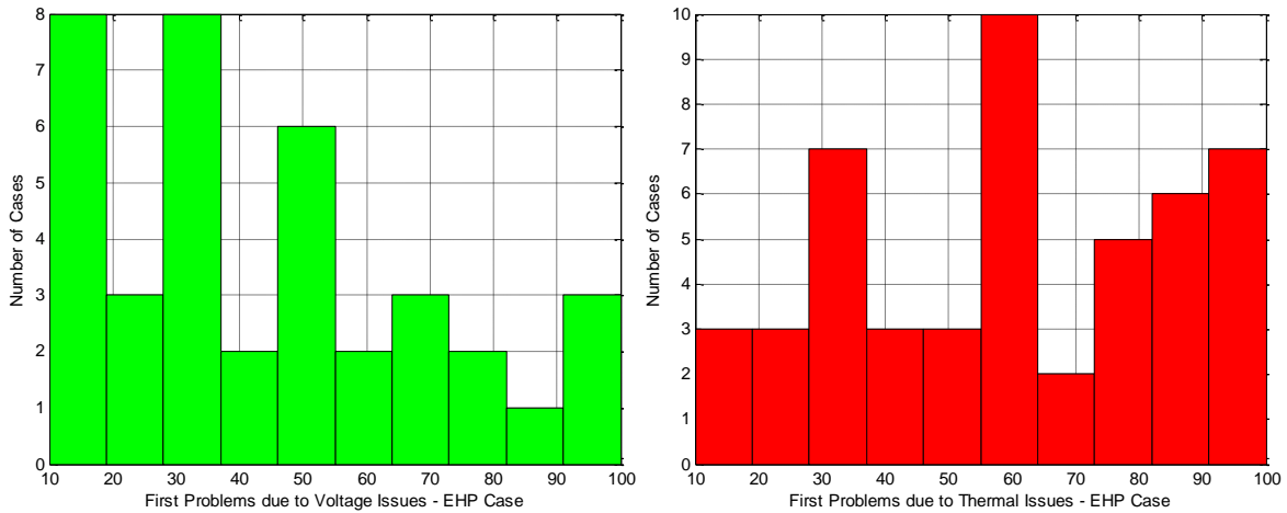
Figure 54: Histograms of First Penetration Level with Technical Problems – EHP Case
