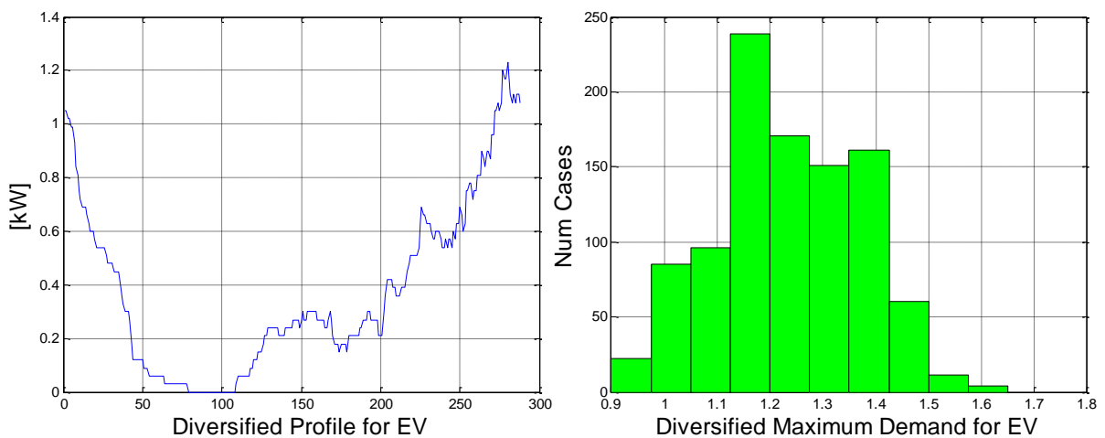
Figure 14: Diversified Profile and Maximum Demand Histogram for 100 EV profiles
