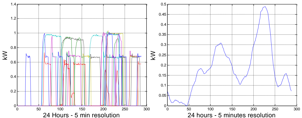
Figure 5: Individual (left) and aggregated (right) \mu CHP generation
