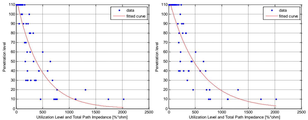
Figure 83: Initial Utilization Level and Total Path Impedance for the EV Fast Charging Case, R^2:0.83 (left) and EV Shifted Case (right), R^2:0.84
