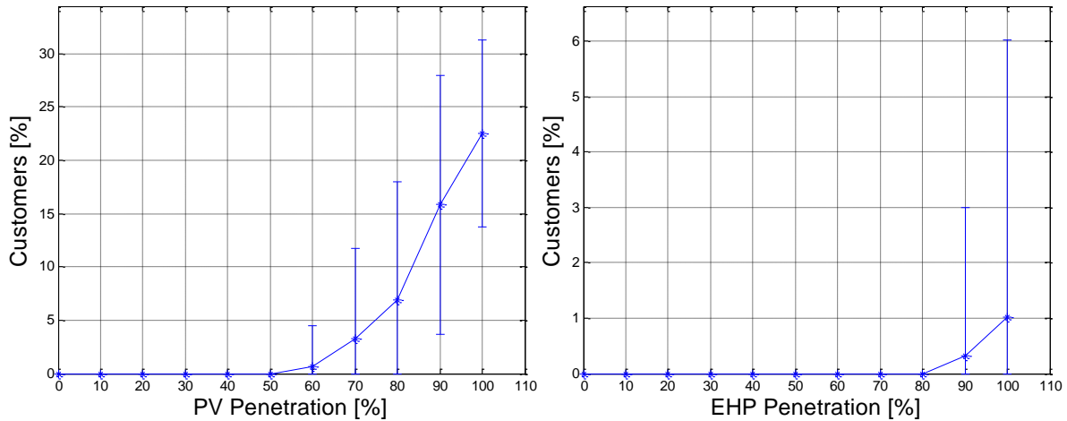
Figure 48: Percentage of customers with voltage problems per technology
