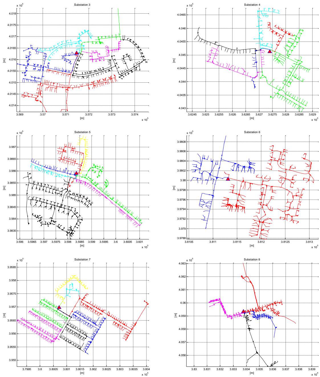
Figure 22: LV Networks 3-8 1
