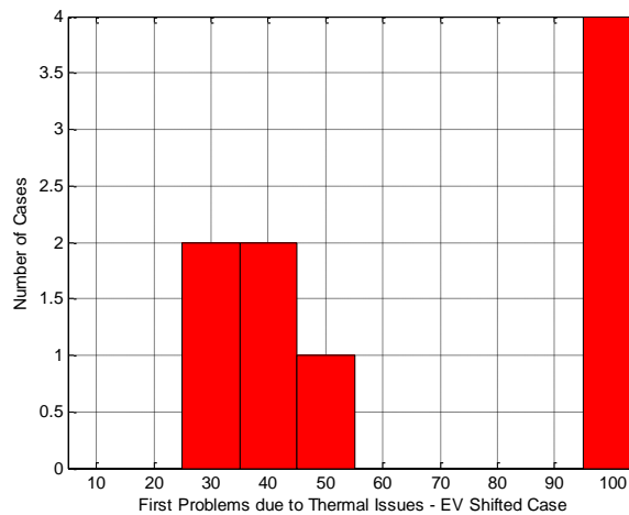
Figure 61: Histograms of First Penetration Level with Thermal Problems – EV peak shifted Case
