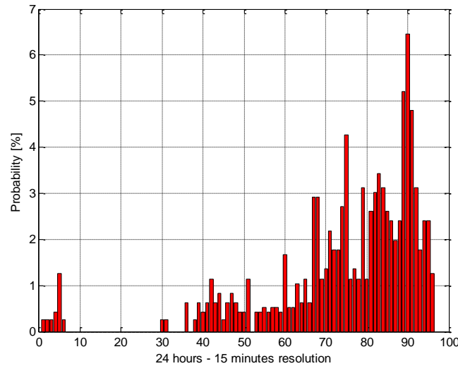
Figure 9: Probability distribution function of EV connection times
