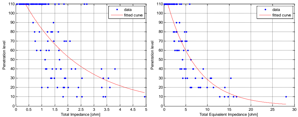
Figure 67: Total Impedance (left), R^2:0.55 and Total Path Impedance (right), R^2:0.78 – PV Case
