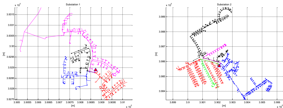
Figure 21: LV Networks 1-2
