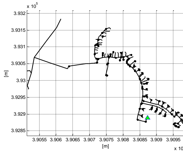
Figure 35: Feeder for the Balanced Case Study and for the Granularity Case Study
