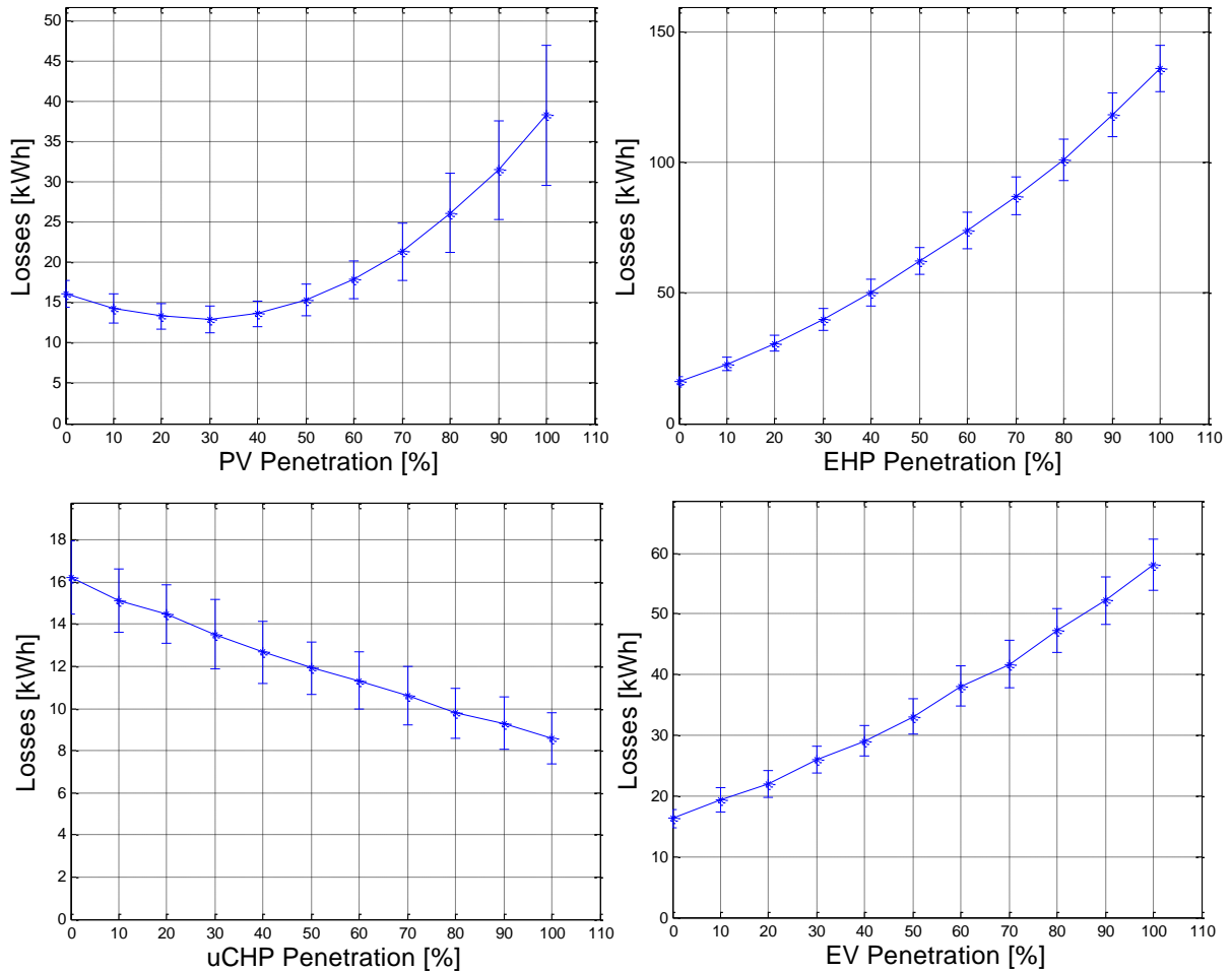
Figure 30: Example of daily energy losses for each technology
