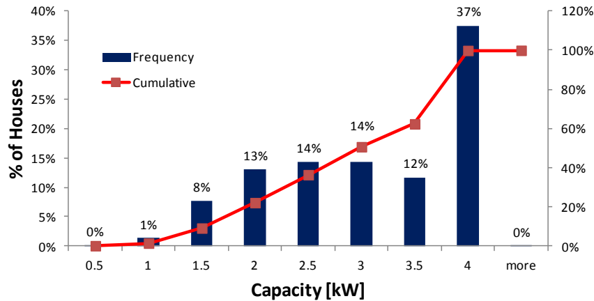
Figure 4: Distribution of residential PV panels in UK
