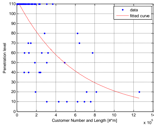
Figure 87: Customer Number and Feeder Length for the EV Case, R^2:0.59
