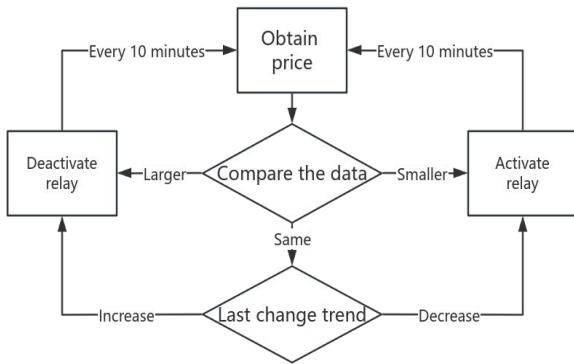
Fig. 15. The software structure of the refrigerator controller
