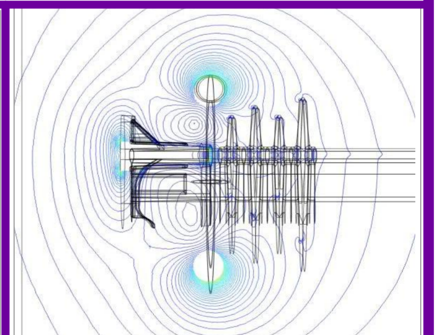
Figure 8 – Electrical FEA
