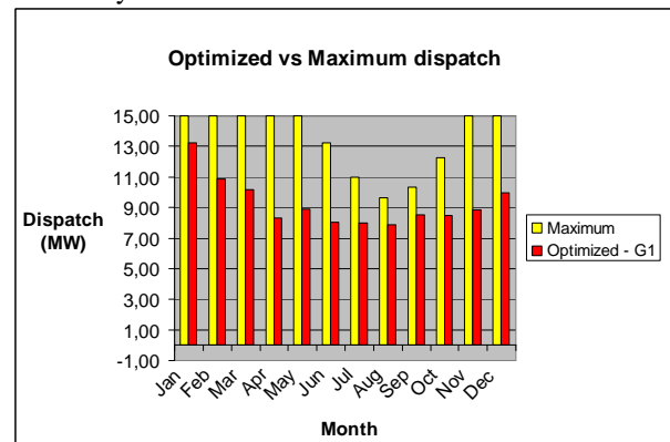
Figure 2: Optimized dispatch VS maximum generation
