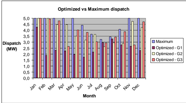
Figure 3: Optimized dispatch VS maximum generation for the second configuration.
