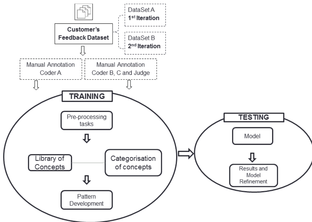
Figure 1. Text mining process.
