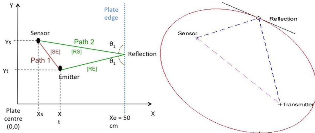
Figure 6: Example of the direct path (path 1) and first reflected path (path 2) from the closest edge (left) and an example of an ellipse with the possible location of the closest edge (in red) (right).
