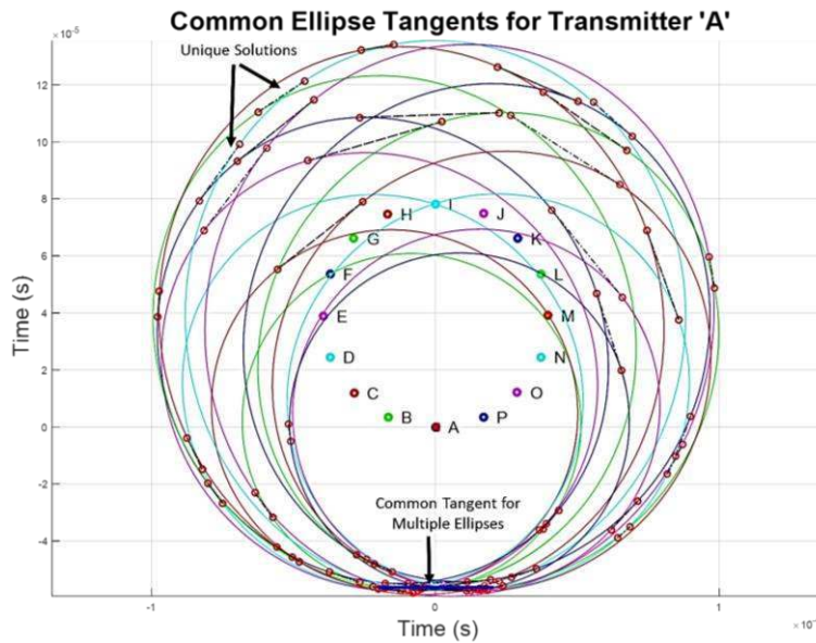
Figure 7: Representation of the detection of the edge location using common ellipse solution (in the time domain).
