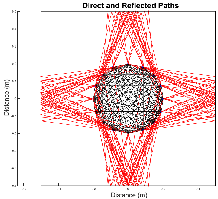
Figure 9: Representation in the special domain of the direct wave's paths (in black) and the reflected wave's paths validated with common tangents (in red).
