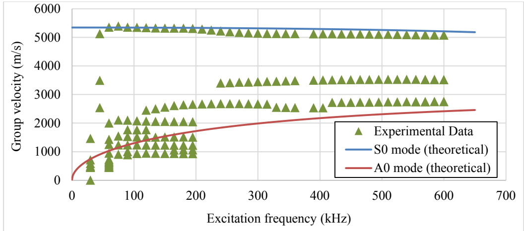
Figure 2: Dispersion curves of the aluminium plate.
