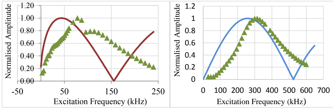
Figure 3: Tuning curve of the antisymmetric mode in red (left) and the symmetric mode in blue (right); the theoretical data (represented in green).
