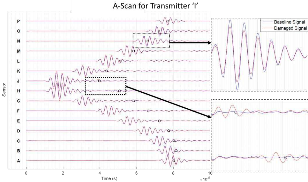
Figure 10: A-scans results obtained for the baseline signal, and after the implementation of a 10mm circular hole, when transducer 'I' is transmitting.
