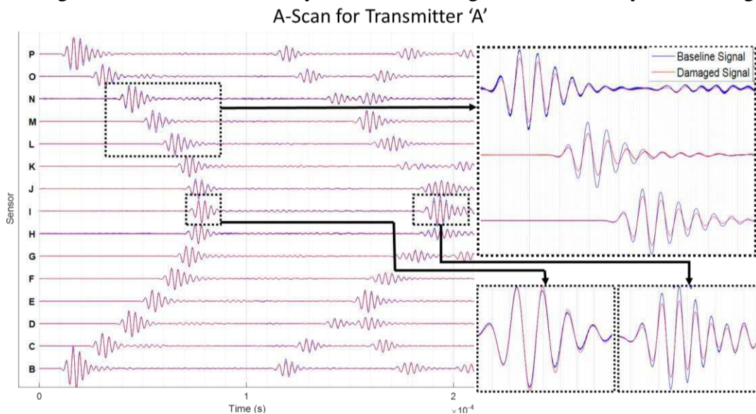
Figure 11: A-scans results obtained for the baseline signal, and after the implementation two coupling defects, when transducer 'A' is transmitting.
