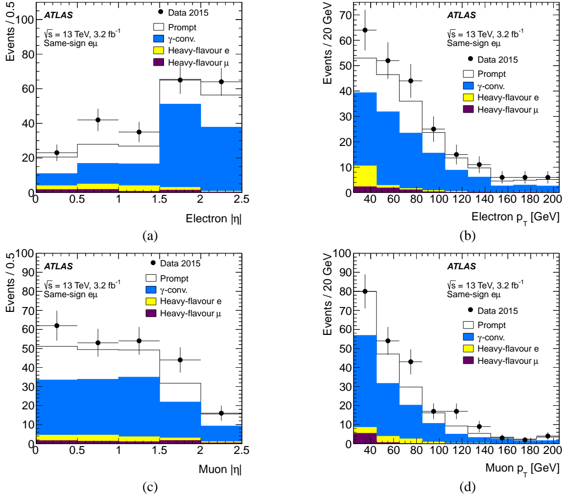
Figure 3: Distributions of electron and muon |\eta| and p_T in same-sign e\mu events with at least one b -tagged jet. The simulation prediction is normalised to the same integrated luminosity as the data, and broken down into contributions where both leptons are prompt, or one is a misidentified lepton from a photon conversion or heavy-flavour decay. In the p_T distributions, the last bin includes the overflow.
