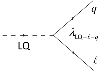
Figure 1: Feynman diagram showing the Yukawa coupling \lambda_{LQ\rightarrow\ell q} between a leptoquark, a lepton and a quark.
