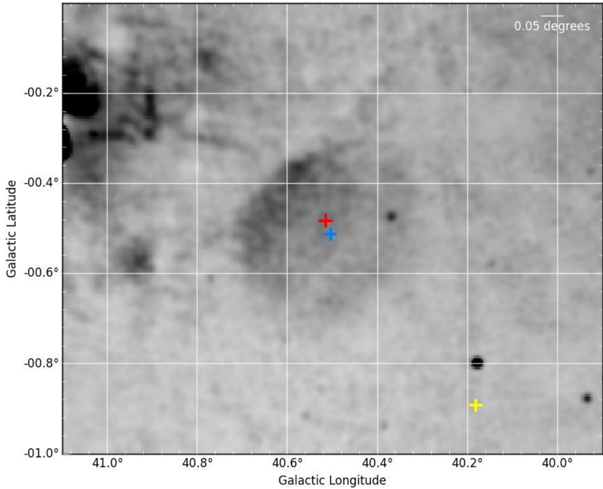
Fig. 6.— A radio image of the region around PSR J1907+0631 in galactic coordinates, taken from the VLA Galactic Plane Survey (VGPS) at 1420 MHz (?). The red cross is the position of the pulsar, the blue cross is the center of the supernova remnant G40.5–0.5 given by Abdo et al. (2010) and the yellow cross is the position of the gamma-ray pulsar, PSR J1907+0602.
