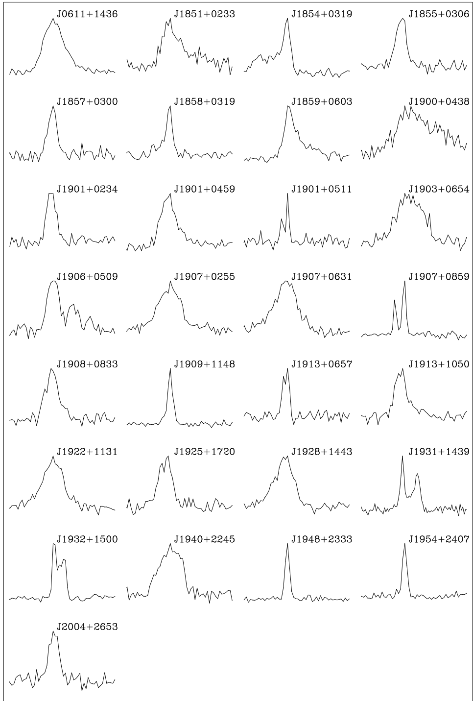
Fig. 4.— The same pulse profiles as presented in Figure ?? but now expanded to show the 20% of the profile around the main peak.
