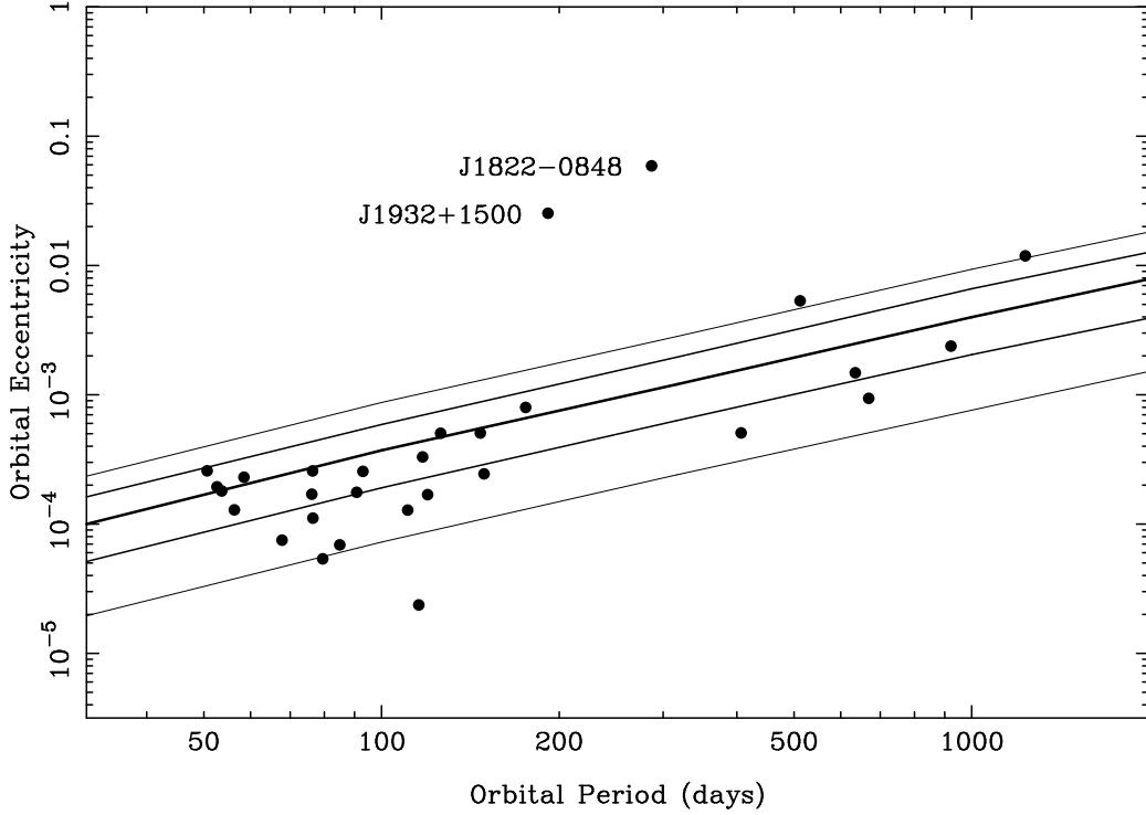
Fig. 7.— The anomalous eccentricities of PSRs J1932+1500 and PSR 1822–0848, compared with those of other long-period, mildly recycled pulsars and the predictions of ?. This diagram includes all known Galactic binary pulsars with orbital period greater than 50 d and minimum companion mass less than 0.5 M_{\odot} (Table ??). The central curve represents the median eccentricity predicted by the convective fluctuation-dissipation theory of ?. The adjacent pairs of lines are predicted to contain 68% and 95% of the resultant eccentricities. Excluding PSRs J1932+1500 and PSR 1822–0848, the observed occupancies of the two ranges are 56% and 85% respectively and are reasonably consistent with the theory.
