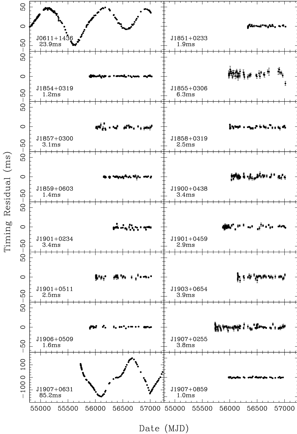
Fig. 1.— Residual pulse arrival times of all pulsars in this paper are given in Figures ?? and ?? to indicate the levels of timing noise. For each pulsar, the residual plot was made by performing a timing fit for just spin-period and spin-down rate, with the best-fit positions given in Table ?? and any binary or glitch parameters given in Tables ?? or ?? held fixed. The root-mean-square of the residuals is given beneath each pulsar name.
