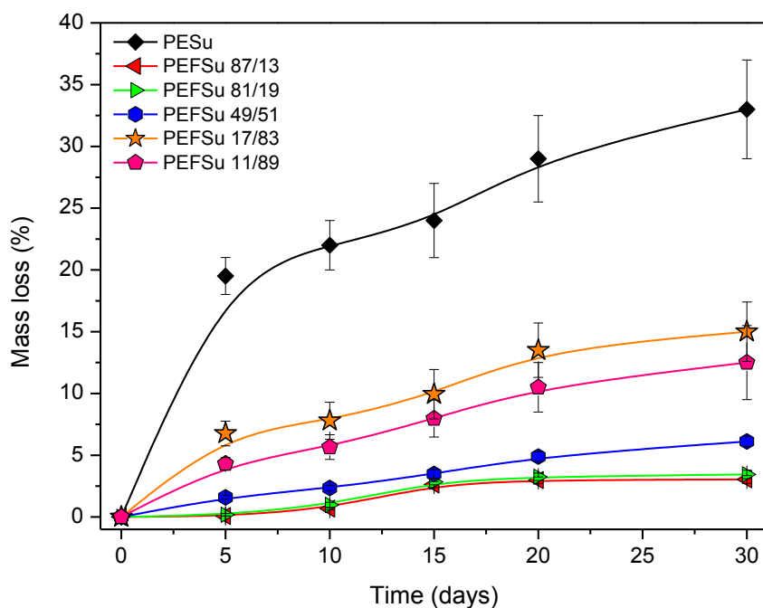
Figure 11. Weight loss plots during enzymatic hydrolysis.
