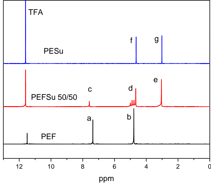
Figure 1. ^1\text{H} NMR spectra of PEF, PESu and the PEFSu 50/50 copolymer.
