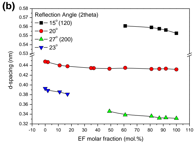
Figure 7. a) WAXD patterns of the PEFSu copolymers and the PEF and PESu homopolymers, b) variation of the interplanar distances (d-spacing) with the composition of PEFSu copolymers
