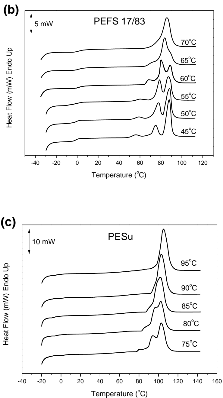
Figure 6. DSC traces of a) PEFSu 92/8, b) PEFSu 17/83 and c) neat PESu samples crystallized at different temperatures.
