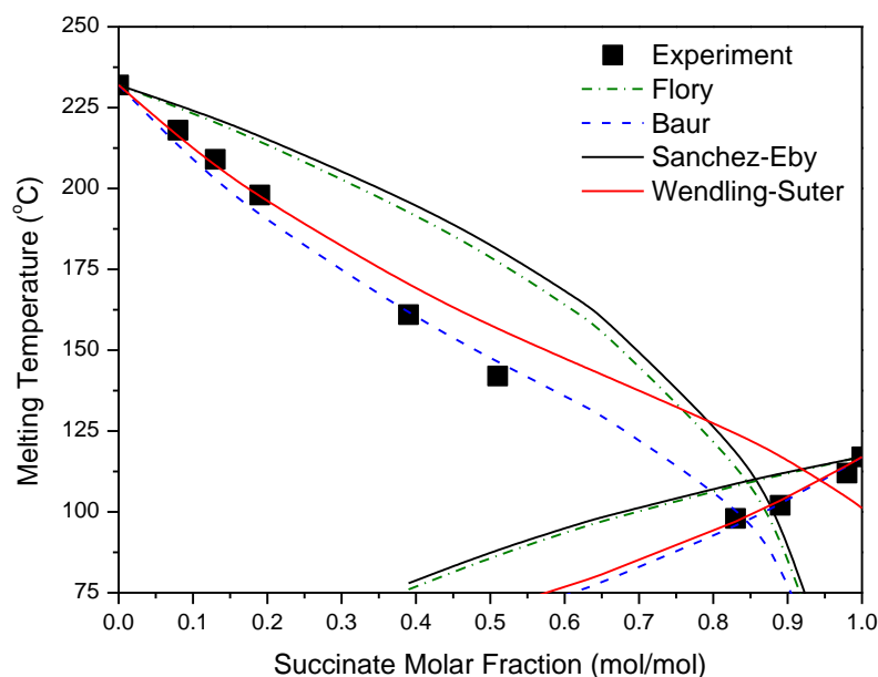
Figure 8. Experimental and predicted melting point as a function of the succinate molar fraction.
