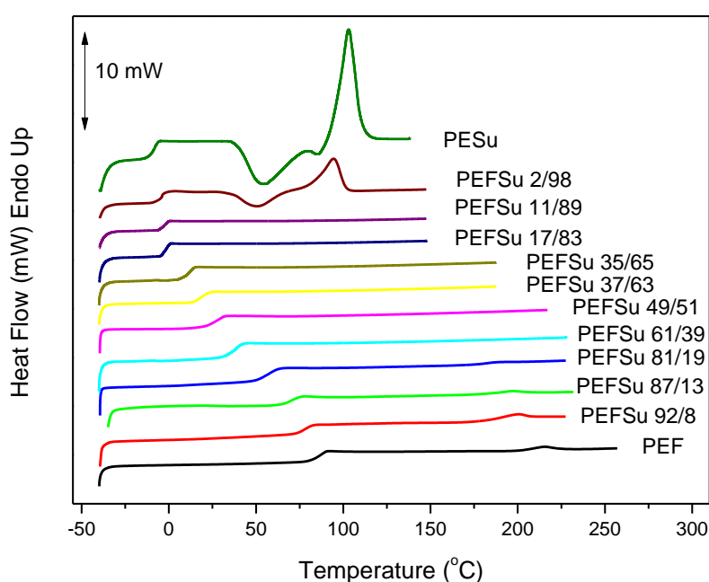
Figure 3. DSC traces of quenched PEF, PESu and PEFSu copolymers.
