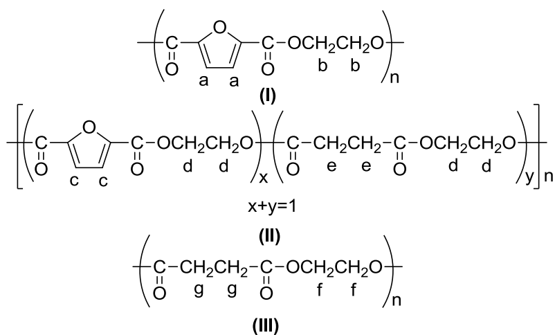
Scheme 1. Chemical structures of PEF (I), the PEFSu copolymers (II) and PESu (III).
