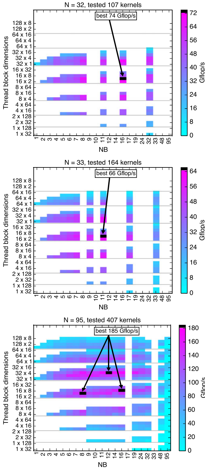
Fig. 14. Performance of all tested kernels for three different matrix sizes, N = 32, 33 , and 95.
