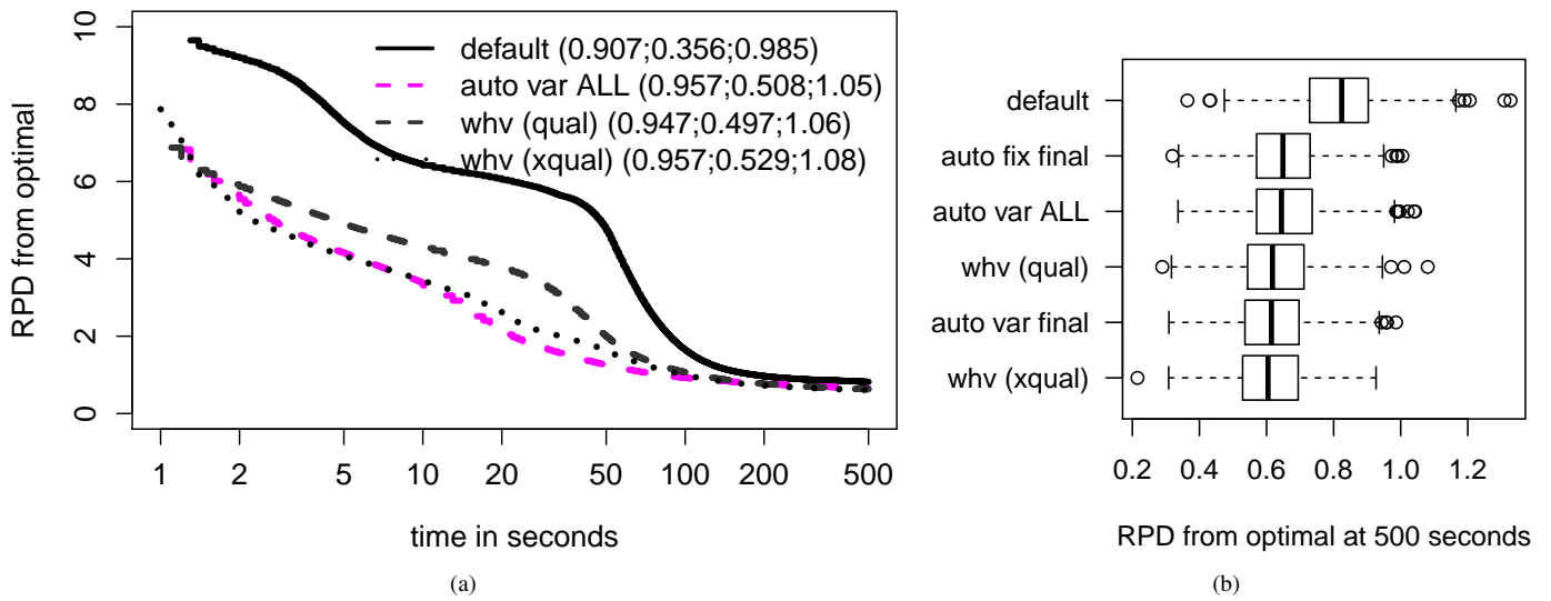
Figure 7: Automatically tuned configurations of MMAS vs. the default configuration. (a) SQT curves, the legend shows the classical hypervolume, and the weighted hypervolume variants w^{\text{qual}} and w^{\text{xqual}} ; (b) Final quality achieved. For the meaning of the labels, see the caption of Table 4.
