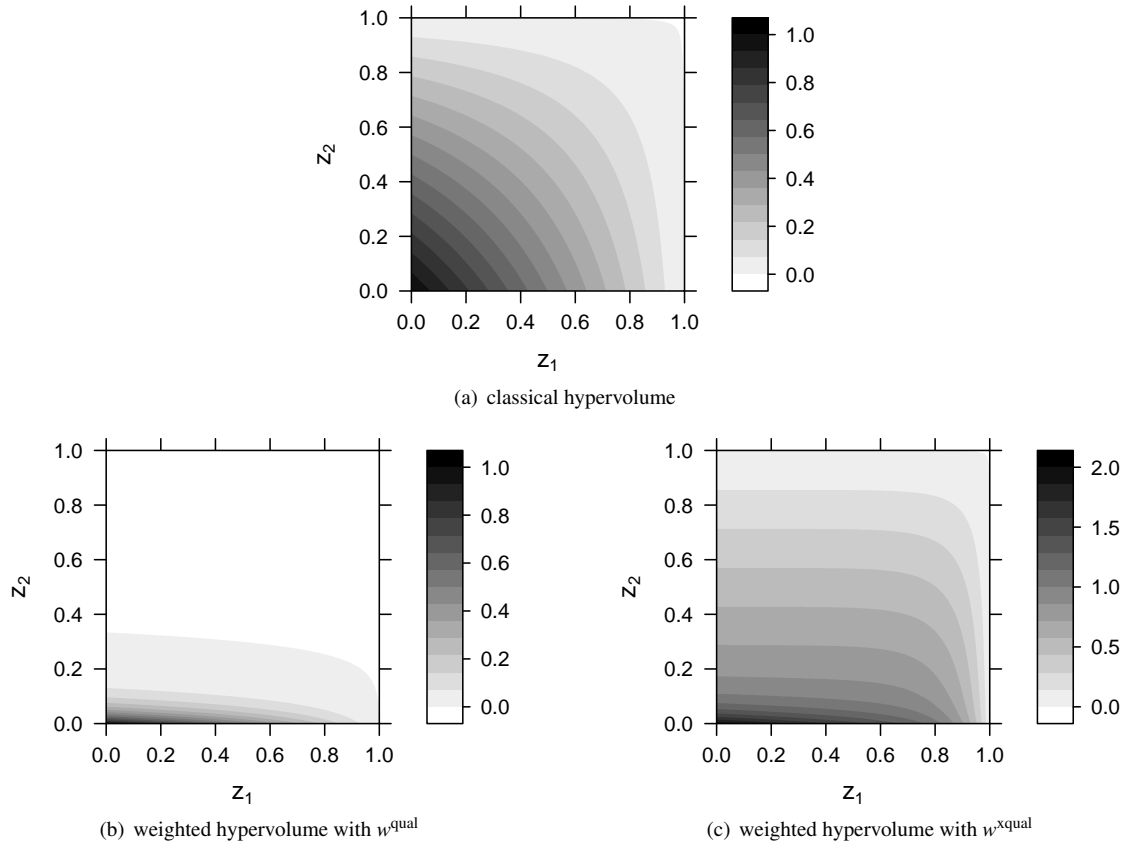
Figure 5: Value of the classical hypervolume (a) and the weighted hypervolume when using weight functions w^{\text{qual}} (b) and w^{\text{xqual}} (c) on the normalised objective space. The grey level at each point gives the (weighted) hypervolume of that individual point, which is computed as the integral of the weight function over the region dominated by the point and bounded above by the reference point (1, 1).
