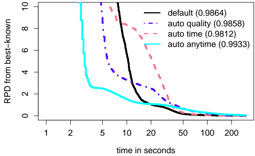
Figure 8: Mean RPD over all test instances for different configurations of SCIP. The number in parentheses is the mean hypervolume corresponding to that configuration.
