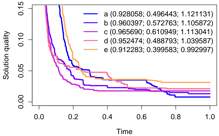
Figure 6: For each performance profile, the legend shows the classical hypervolume, and the weighted hypervolume variants w^{\text{qual}} and w^{\text{xqual}} .
