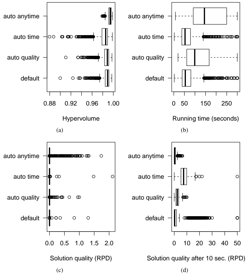
Figure 9: Boxplots of the results obtained by four different parameter configurations of SCIP according to various evaluation criteria.
