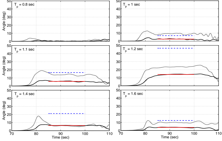
FIGURE 10. Envelopes of the hinge angle response of the M4 machine with time, which have been multiplied by \exp[0.023\omega_R(t - 85)] , for all wave group tests and for two amplitudes: A_c = 0.0245 m shown in black lines, and A_c = 0.08 m in grey lines. Red solid line is the average of the smaller amplitude response taken from 85 – 100 sec, while blue dashed line is the same response scaled up by the ratio of the large to small linear amplitudes at focus, over the same time interval.
