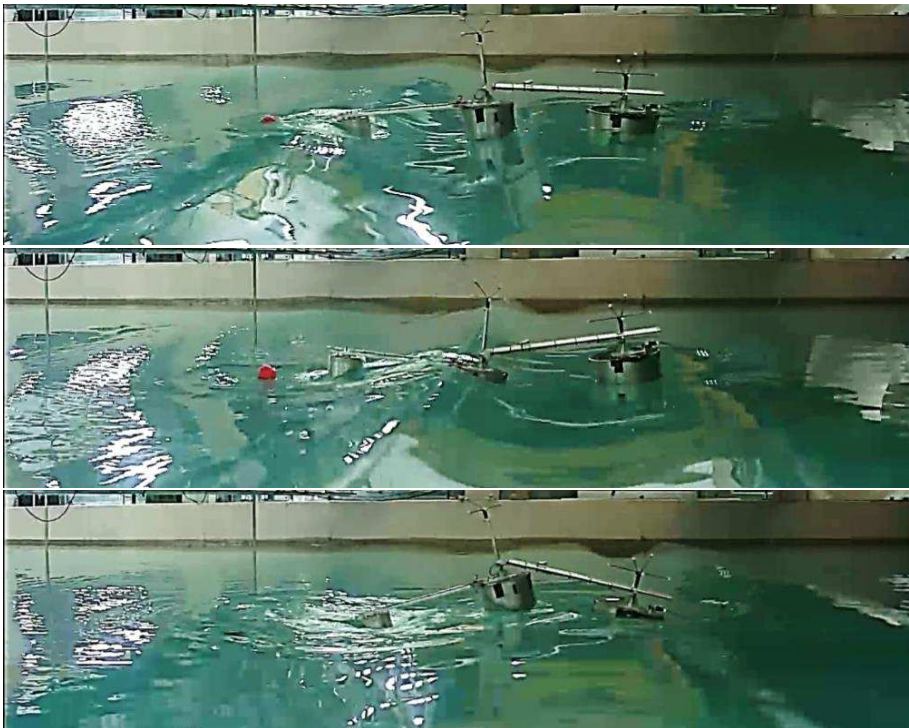
FIGURE 3. Series of snapshots of the M4 machine for the focussed wave group of A_c = 0.08 m and T_p = 1.2 sec. Top figure shows float 1 and (red) buoy being dunked as the wave group was arriving. Middle figure shows float 2 being dunked when the wave group was focussed in space and time. Bottom figure shows the maximum hinge angle (almost self-collision) during free vibration as the wave group passed through the model, where floats 1 and 3 were almost dunked and (red) buoy completely submerged from the water surface. The two vertical bars at the left side of each figure are the upstream wave probes. The wave group travels from left to right.
