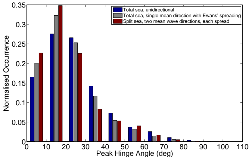
FIGURE 18. Histogram of the peak hinge angle distribution of the M4 machine from 1958 – 2011 at Orkney for three different sea-state assumptions. The probability of a response level in each 10^\circ bin is given by the height of the bar in that bin.
