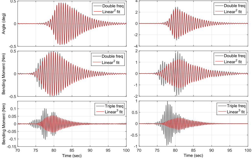
FIGURE 5. Comparison of the higher harmonic signals (thick grey line) and the fit using linear signal approximations (thin red line) for A_c = 0.0245 m (left panel) and 0.08 m (right panel), all for T_p = 1.2 sec. First row shows shape comparison in terms of double frequency component of hinge angle. Second and third rows show shape comparison in terms of double and triple frequency component of bending moment.
