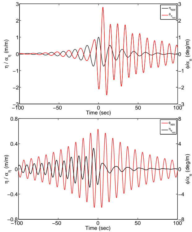
FIGURE 15. Top figure: Plot of the NewWave focussed wave group in time at the focus location without the presence of the M4 machine (black line), and the associated response in time due to the wave group (red line) for 1 in 3 hour response level. Bottom figure: Plot of the NewWave machine response in time (red line), and the associated input designer wave group that leads to the maximum expected response (black line). All plots are normalised by \alpha_\eta .
