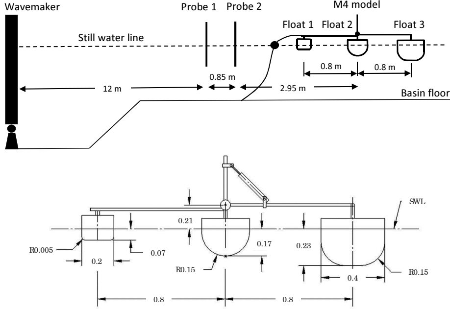
FIGURE 1. Top figure shows the layout (side view) of the experimental setup with the lab-scale M4 model (not to scale). Bottom figure show the dimensions (in m) of the M4 model. Note the power take off is shown above the beam while this would be connected to the deck on a prototype. For the present tests in extreme conditions it is disconnected.
