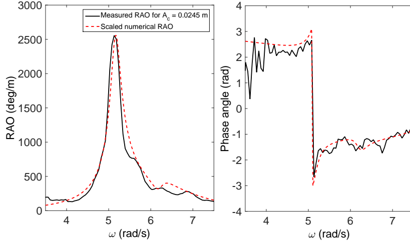
FIGURE 8. Comparison of the RAOs derived from wave group experiments with A_c = 0.0245 (solid line) and scaled RAO using DIFFRACT (dashed line) in terms of amplitude (left figure) and phase angle (right figure).
