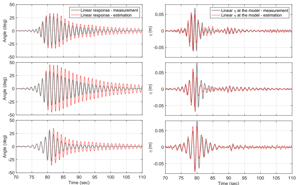
FIGURE 11. Left panel: Comparison between the measured linear hinge angle (grey lines) and the estimated linear response based on the large input wave history and the small wave group RAO (red lines). Right panel: Comparison between the measured linear surface elevation (grey lines) and the estimated linear surface elevation based on the actual large machine motion and the small wave group RAO (red lines) at the model. All plots are for A_c = 0.08 m and T_p = 1.1 sec (top), 1.2 sec (middle) and 1.4 sec (bottom).
