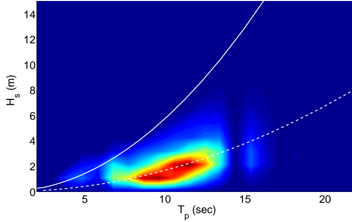
FIGURE 13. Scatter diagram of normalised occurrence of H_s and T_p at Orkney from 1958–2011, with red region indicating the highest number of occurrences. Solid line represents the constant limiting steepness, dashed line represents the constant average steepness.
