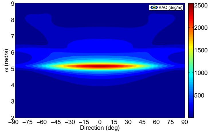
FIGURE 9. Presentation of the numerically derived 2D RAO as a function of frequency and incident wave direction.
