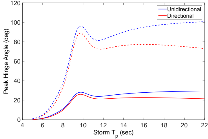
FIGURE 16. Peak hinge angle response for unidirectional (blue lines) and directional (red lines) sea-states along the limiting steepness lines (dashed lines) and the mean steepness lines (solid lines).
