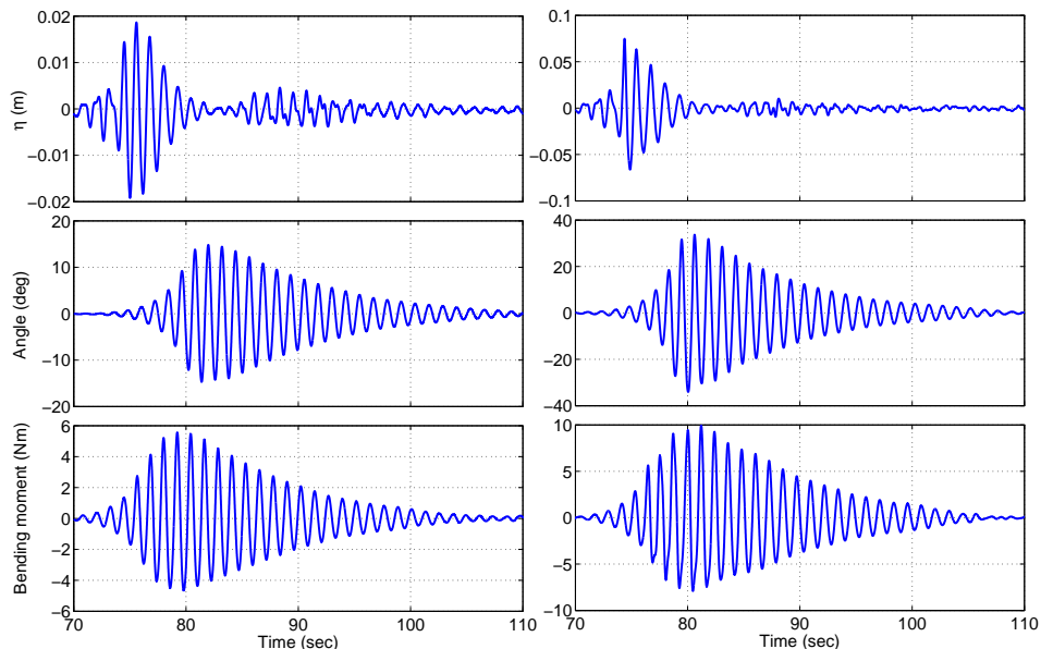
FIGURE 2. Examples of the measured data for A_c = 0.0245 m (left panel) and 0.08 m (right panel), all for T_p = 1.2 sec. Top row shows the surface elevation time history from probe 1 upstream of the M4 machine, see figure 1. Middle row shows the hinge angle response time history. Bottom row shows the bending moment time history between float 1 and 2, see figure 1.
