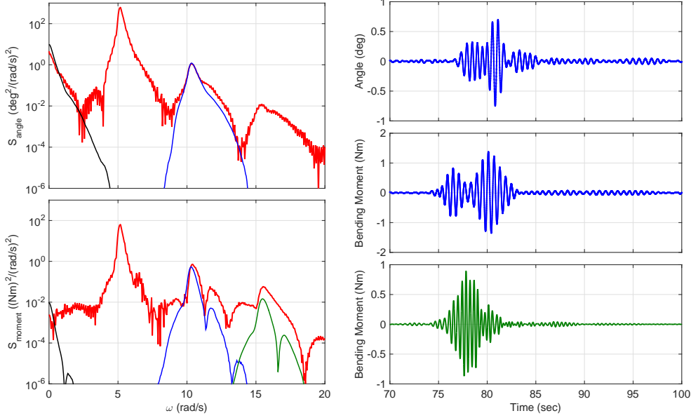
FIGURE 6. Left panel: Power spectra of the total signals in terms of hinge angle (top) and bending moment (bottom), all shown in thick red lines. The thin lines correspond to the spectra of the fitted Stokes-like harmonics shown previously in figure 5 and with the same colour coding as figure 4. The difference in the spectral shape for each harmonics corresponds to the non Stokes-like contributions in frequency, this is plotted in the right panel in time. Right panel: The difference in the higher harmonic signals and the fit using linear signal approximations. First row shows the difference in double frequency component of hinge angle. Second and third rows show the difference in double and triple frequency component of bending moment. All plots are for A_c = 0.08 m and T_p = 1.2 sec.
