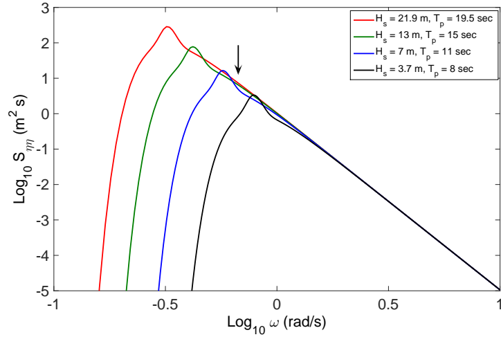
FIGURE 17. Universal tail form of the standard JONSWAP spectrum for all storms with same steepness ( H_s/T_p^2 ). The downward pointing black arrow indicates the frequency of the peak RAO of the full scale M4 machine.
