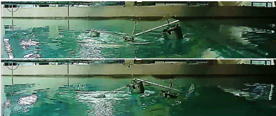
FIGURE 12. Snapshots of the M4 machine during violent focussed wave group test.
