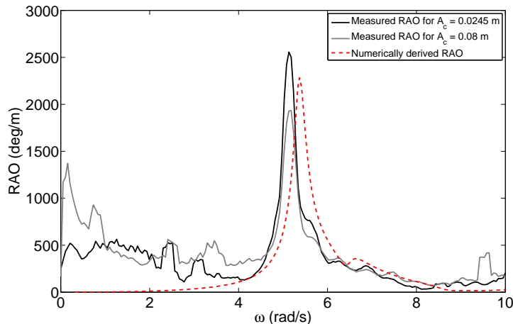
FIGURE 7. Comparison of the RAOs derived from wave group experiments with A_c = 0.0245 and 0.08 m (black and grey lines, respectively) and numerically derived RAO using linear potential diffraction solver DIFFRACT (dashed line).
