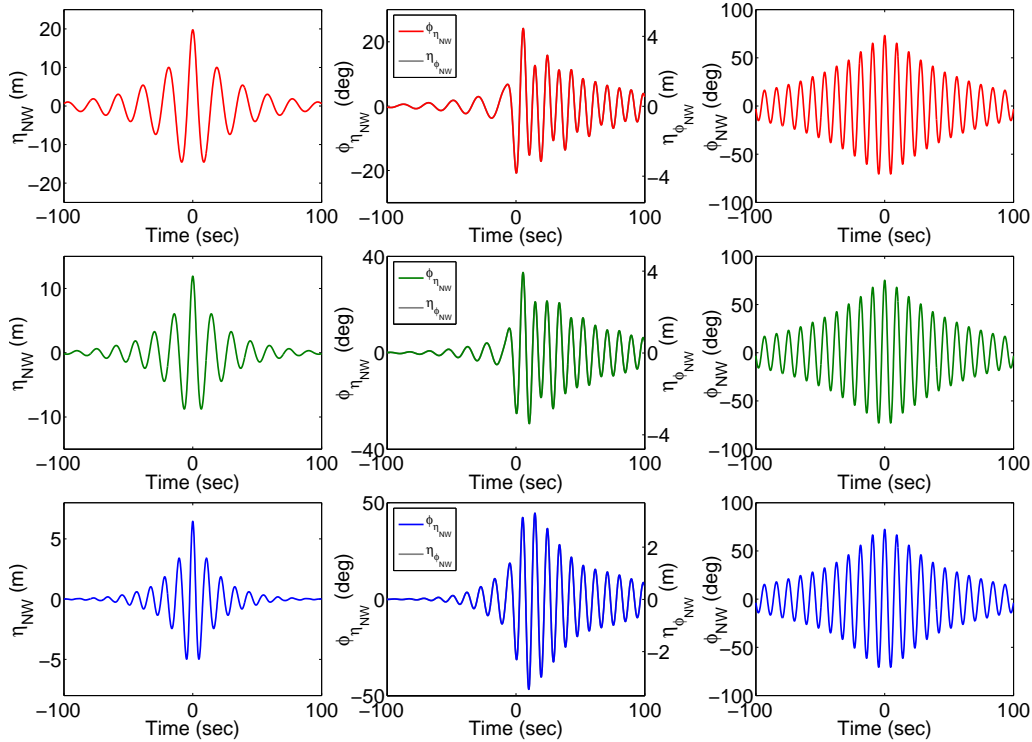
FIGURE 19. Plots of wave and machine response time histories for limiting steepness storms with T_p = 19.5 sec (top panel), T_p = 15 (middle panel) and T_p = 11 sec (bottom panel). Left hand column shows the shape of the most probable maximum wave crests in 3 hours for each sea-state ( \eta_{NW} ). Right hand column shows the most probable maximum response in time in 3 hours for each sea-state ( \phi_{NW} ). Centre column shows the machine response given an input wave group matching the most probable maximum wave in time ( \phi_{\eta_{NW}} ), and also the wave group (with the time axis reversed) which would produce the most probable machine response in time ( \eta_{\phi_{NW}} ).
