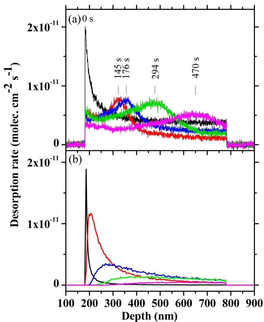
Figure 7: The depth dependence of the yields of HD: (a) produced from thin films of ASW layered as H 2 O/D 2 O/H 2 O for samples when the experiment started a time zero but the electron gun started emitting electrons at 180 sec.; S1 (black), S2 (red), S3 (blue), S4 (green) and S5 (magenta) (Table 1) and (b) the results from MC simulation at the same conditions of samples from S1 to S5. All films were exposed to 450 eV electrons.
