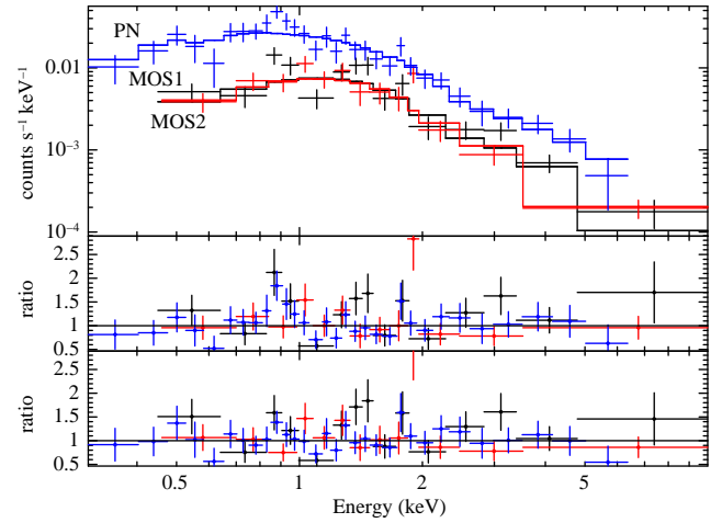
Figure 6. XMM-Newton spectrum of IC 883. Middle and lower panels correspond to the data to model residuals, \text{tbabs}^*\text{powerlaw} and \text{tbabs}^*(\text{powerlaw} + \text{apec}) , respectively.
