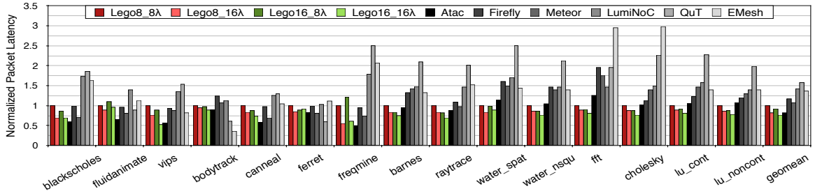
Figure 14: Average packet latency on SPLASH-2/PARSEC benchmarks normalized to Lego8_8λ
