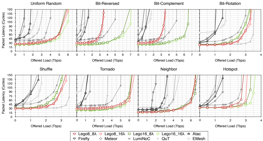
Figure 13: Average packet latency on synthetic workloads
