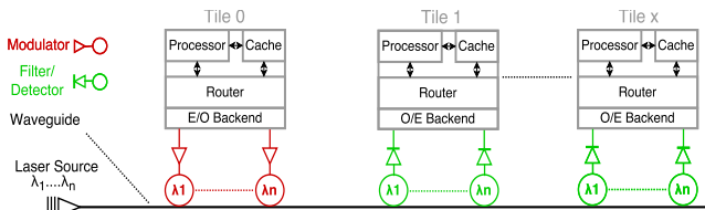
Figure 1: Single-Writer-Multiple-Reader Optical Bus
