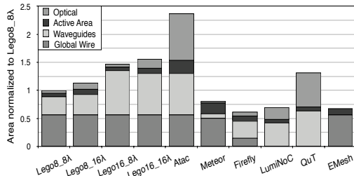
Figure 18: Normalized Area Breakdown
