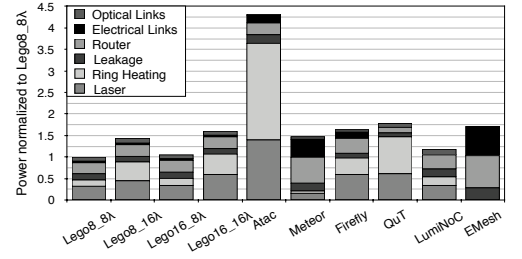
Figure 16: Power breakdown
