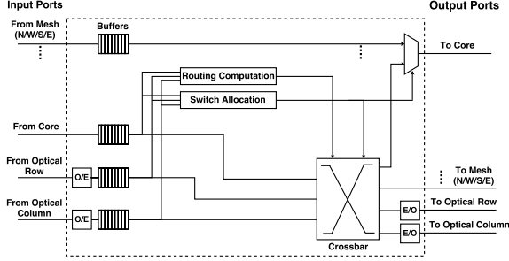
Figure 12: Router Architecture
