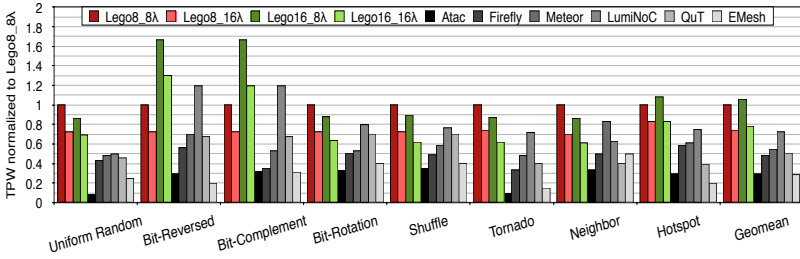
Figure 15: Normalized Throughput-per-Watt
