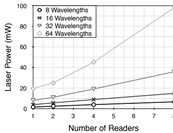
Figure 3: Laser Power vs. Num. of Receivers in a SWMR bus
