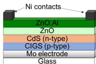
Figure 10. The typical architecture of a CIGS device.
