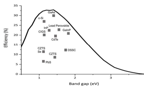
Figure 2. An illustration of the Shockley-Queisser limit (maximum theoretical efficiency) for solar cells under AM 1.5 illumination. The band gaps of a selection of photovoltaic materials is shown for comparison.
