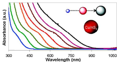
Figure 8. Absorption spectra of CIS nanocrystals of different sizes between 2 and 16 nm. Reprinted with permission from ref. [92], ©2013 American Chemical Society.
