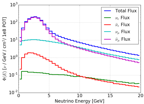
Figure 2. Neutrino flux at the ArgoNeuT detector in anti-neutrino mode.
