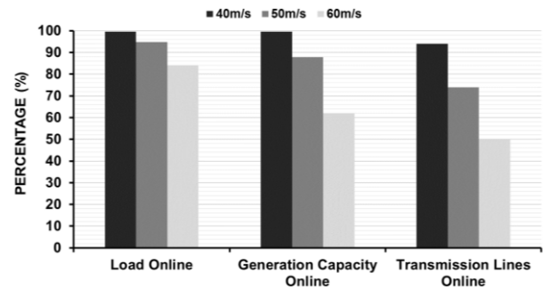
Fig. 8. The A -metric for the base case scenario
