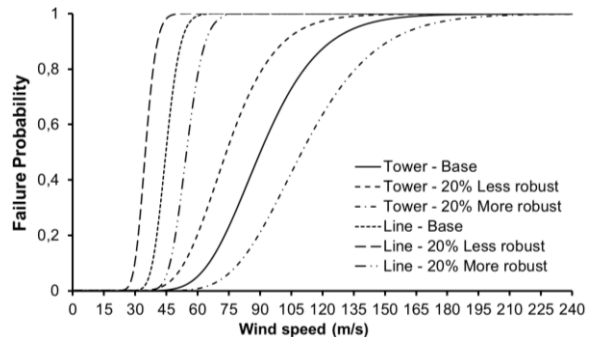
Fig. 6. Wind fragility curves used in the base and robust case scenario
