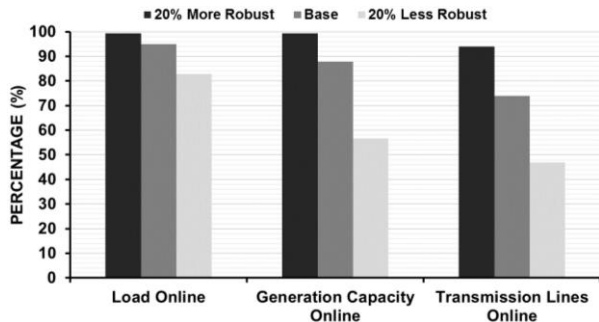
Fig. 9. The A -metric for the robust case scenario and WS_{50m/s} .
