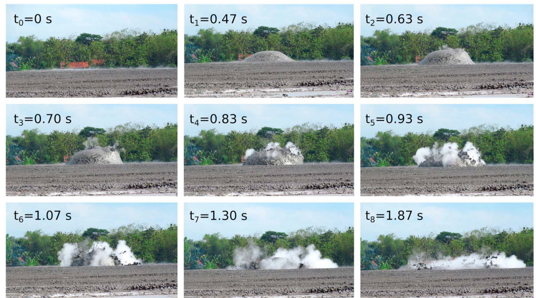
Figure 2. Snapshots of a bursting gas bubble of the main vent (vent II) at the Bledug Kuwu complex. The bursts had a duration of approximately \sim 2 s.
