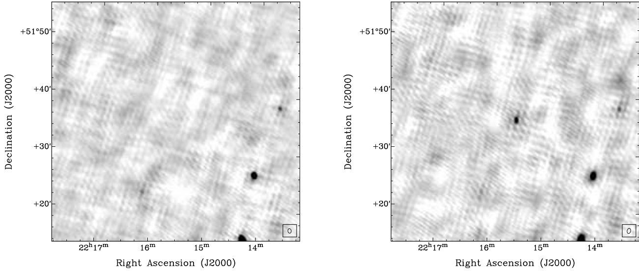
Figure 1. Left: 124-MHz LOFAR map from 2013 February 10 (MJD 56333.509), zoomed in on the position of PSR J2215+5135. The angular resolution is 48 arcsec \times 35 arcsec (synthesized beam position angle 10^\circ ), and the rms noise level is 13 mJy beam ^{-1} . The pulsar is not detected. Right: The same field, but from the observation on 2014 January 15 (MJD 56672.578). In this case, the angular resolution is 55 arcsec \times 37 arcsec (beam position angle -11^\circ ), and the rms noise level is 15 mJy beam ^{-1} . PSR J2215+5135 is now detected at approximately 15 times the local rms noise level, with a flux density of 228 mJy. The synthesized beam is shown in the bottom right-hand corner of each panel.
