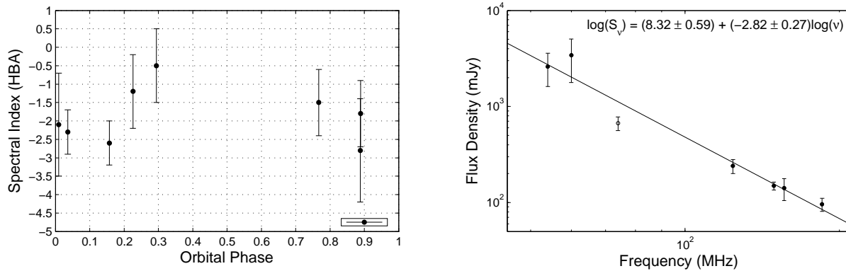
Figure 4. Left: Spectral index in the high band, as a function of orbital phase. We follow the same conventions as in Figure 2. Right: Radio spectrum for PSR J2215+5135. The filled circles are the LOFAR mean fitted flux densities from Table 4, and the open circle is the 74-MHz VLSSr flux density, adjusted to the scale of Baars et al. (1977). A linear least-squares fit in \log(S_\nu) – \log(\nu) space, with inverse-variance weighting, to the six LOFAR data points, is shown (solid line); the reduced \chi^2 value is 0.59.
