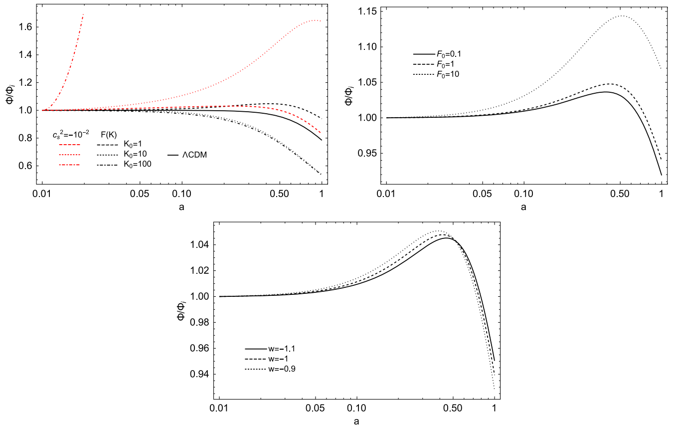
FIG. 4. Top left panel: The evolution of the Newtonian potential, \Phi , in \Lambda\text{CDM} (black solid line) and for different scales in a designer \mathcal{F}(\mathcal{K}) model (dashed and dotted lines) for \mathcal{F}_0 = 1 and w_{\text{de}} = -1 . Note that the potential for the \Lambda\text{CDM} model is scale independent. For comparison we also show the evolution of \Phi with the presence of a dark energy fluid with w_{\text{de}} = -1 and a constant negative squared sound speed of c_s^2 = -10^{-2} (red lines), calculated using (144). Top right panel: The evolution of \Phi in a generalized Einstein-Aether universe with varying \mathcal{F}_0 for w_{\text{de}} = -1 and K_0 = 1 fixed. Bottom panel: The evolution of \Phi for a general Einstein-Aether fluid with w_{\text{de}} varying around -1 , with \mathcal{F}_0 = 1 and K_0 = 1 fixed.
