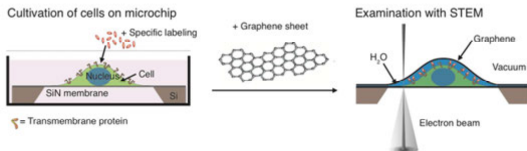
Figure 1. Scanning transmission electron microscopy (STEM) of quantum dot (QD) labeled ErbB2 proteins in graphene-enclosed, hydrated cells. Schematic of the experimental approach, showing a eukaryotic cell (green), cultivated on a silicon microchip with a silicon nitride (SiN)-window in a cell culture dish. After the specific labeling of ErbB2 proteins (orange) with QDs (red), the hydrated fixed cells are coated with a graphene sheet, and subsequently studied with electron microscopy.
