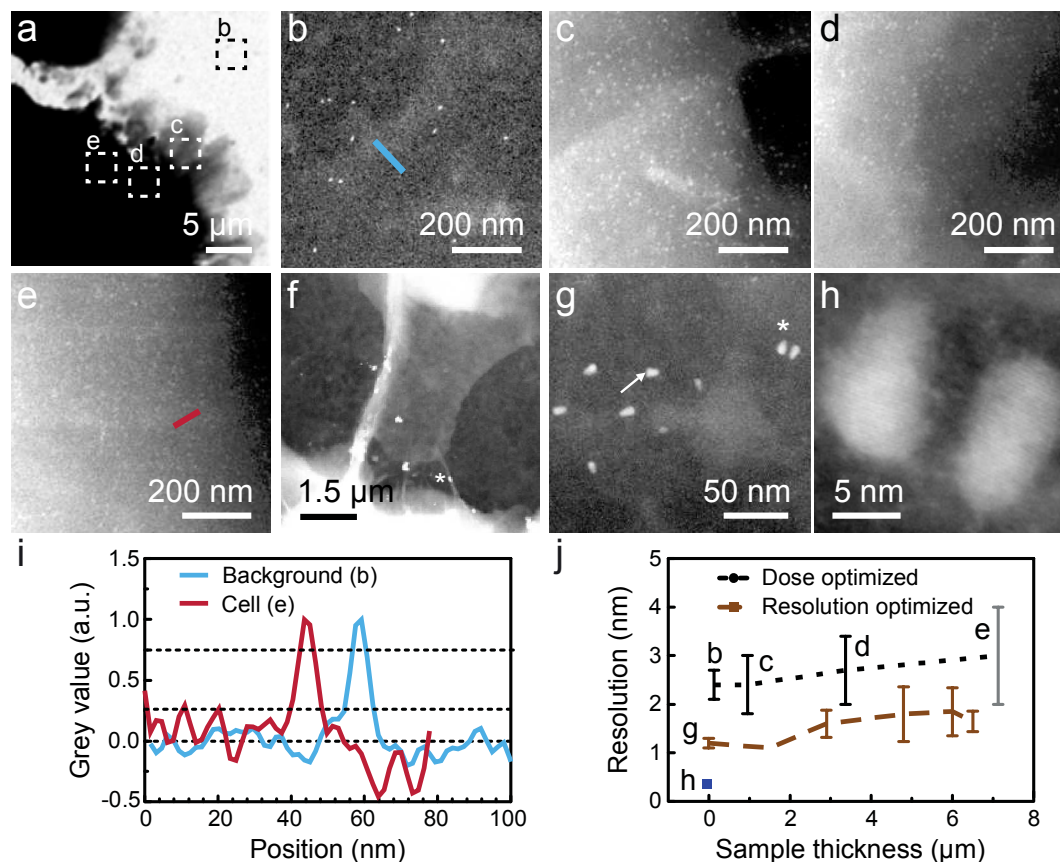
Figure 4. Spatial resolution obtained on Quantum Dots (QDs) in STEM images in relation to the sample-thickness of graphene covered, hydrated cells. (a) Overview bright field STEM image acquired with M = 2.500\times . (b-e) STEM images showing individual QDs recorded regions of increasing sample thickness of \sim 0, 1, 3, and 7 \mu\text{m} in addition to the thickness of the SiN membrane. The signal-to-noise-ratio decreased with increasing thickness, and the background signal varies over the images reflecting thickness and density variations of the cell. The images were acquired for low dose settings using M = 120,000\times , d = 1.6 \text{ nm} , I_p = 20 \text{ pA} , and q = 10 \text{ e}^-/\text{\AA}^2 . A noise filter was applied to the images, and cropped regions are shown. The locations of the images are indicated in panel a. (f) Dark-field overview STEM image ( 2048 \times 2048 pixels) obtained using M = 20,000\times . (g) STEM image of QDs acquired with settings optimized for high resolution in a thin sample region, using M = 400,000\times , d = 0.24 \text{ nm} , I_p = 44 \text{ pA} , and q = 9.8 \times 10^2
