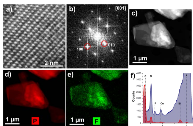
Figure 2. (a) HRTEM image and (b) the associated fast Fourier transform (FFT). The FFT indexes to black phosphorus viewed down the [001] zone axis. (c) High angle annular dark field scanning transmission electron microscope (HAADF STEM) image of freshly prepared FL-BP. EDX spectrum imaging of the region shown in (c) was used to produce maps of P (d) and F (e) demonstrating colocalization of P and F. (f) Comparison of spectra taken from the flake in (c) (shown in blue) and from the surrounding carbon support (shown in red), further demonstrate that F is spatially co-localised with P.
