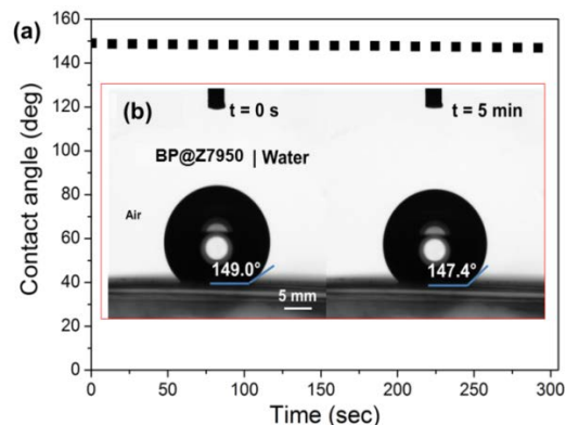
Figure 4. Contact angle measurements on a PVDF membrane with BP immobilized at the surface. (a) Plot of contact angle ( ^\circ ) over time for a drop of deionized water on the BP supported by PVDF membrane. (b) Optical images (CCD camera) of the contact angle of a deionised water droplet on the BP-coated membrane at t = 0 and 5 min.
