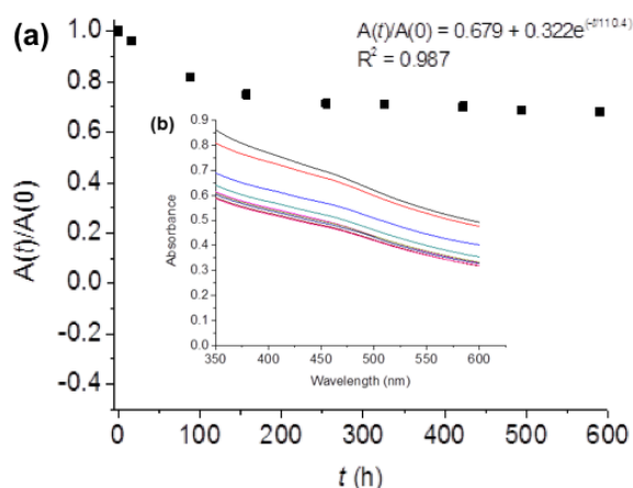
Figure 3. Stability of BP flakes in solution. (a) The degradation of FL-BP flakes in aqueous 1% w/v Z7950 determined by the ratio of optical absorption at 465 nm at time t and time zero. The observed lifetime from the fitted decay is around 110 h, whilst ca. 68% of the flakes remains undegraded over a period of ca. 1 month in this media. Inset: data fitting and R^2 . (b) UV-Vis absorption data used to construct the plot in (a).
