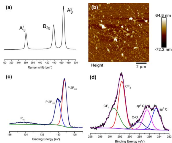
Figure 1. Characterization of as-prepared BP nanosheets from liquid phase exfoliation of bulk BP in 1% w/v Zonyl 7950. (a) Raman spectrum of BP nanosheets showing the characteristic optical phonons at 361, 438 and 465 \text{cm}^{-1} . (b) AFM of as-prepared BP nanosheets, with z = 17.1 \pm 2.1 nm ( N = 50 ). (c) High resolution XP spectrum of the phosphorus region of BP nanosheets, showing minimal oxidized species (Pox). (d) High resolution XP spectrum of the carbon region of BP nanosheets, showing the presence of \text{CF}_3 , \text{CF}_2 and C-O, all associated with the binding of Z7950 to BP.
