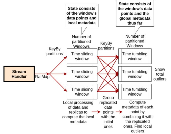
Fig. 4. Main implementation rationale with random partitioning, where the parallelized sliding window is followed by a partitioned tumbling meta-window.
