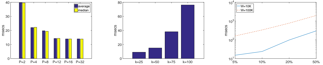
Fig. 8. The impact of the degree of parallelism P (left), k (middle) and the window size W (right) on pMCOd's performance.
