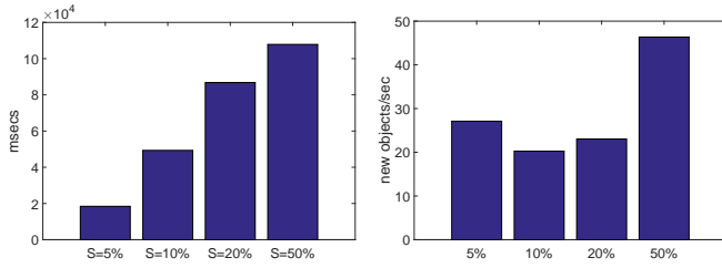
Fig. 3. Average processing time per slide (left) and input stream consumption rate (right) for the baseline approach.
