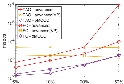
Fig. 10. Average slide processing time for different slide sizes for the TAO and FC datasets
