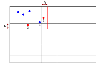
Fig. 5. Value-based partitioning
