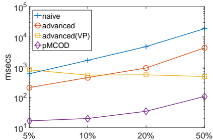
Fig. 9. Average slide processing time for different slide sizes for the artificial dataset
