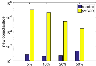
Fig. 7. Throughput comparison for W = 10K .
