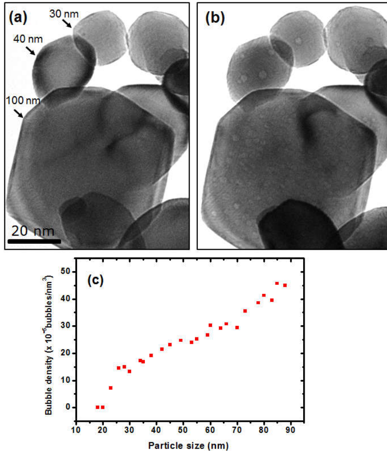
Figure 4. Underfocus BF-TEM images for W NPs: (a) unirradiated and (b) irradiated to a fluence of 1.1 \times 10^{17} ions/cm 2 showing the bubble distributions in NPs of different sizes. The relationship between bubble density and particle size for W NPs with different diameters irradiated to a fluence of 1.1 \times 10^{17} ions/cm 2 is shown in (c). (The scale marker in (a) applies to both images.)
