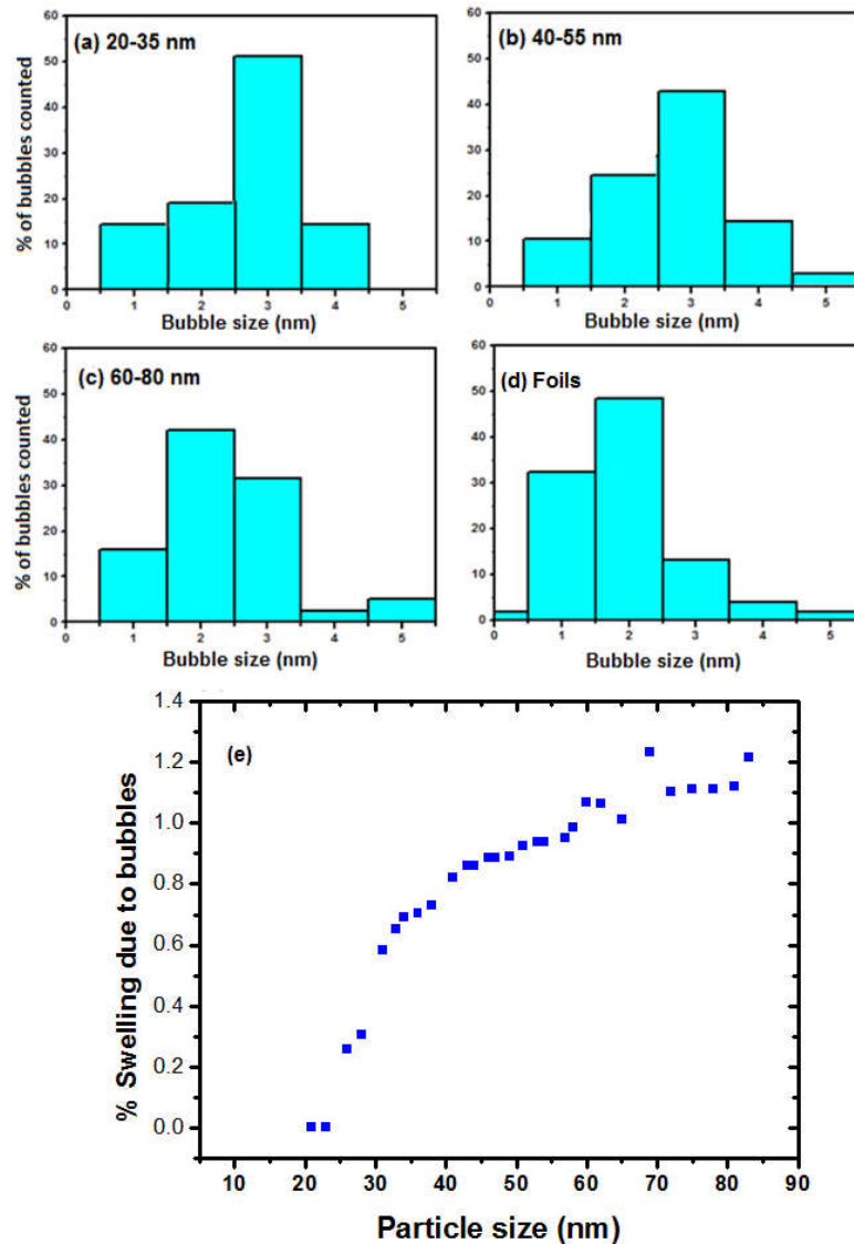
Figure 5. Distribution of bubble sizes in W irradiated with 15 keV He to a fluence of 1.1 \times 10^{17} ions·cm -2 : (a) 20–35 nm NPs (sample = 80 bubbles in 20 NPs); (b) 40–55 nm (sample = 200 bubbles in 20 NPs); (c) 60–80 nm (sample = 280 bubbles in 28 NPs); and (d) the foils (sample = 280 bubbles). (e) Plot of the size dependence of swelling due to bubbles for W NPs of different diameters.
