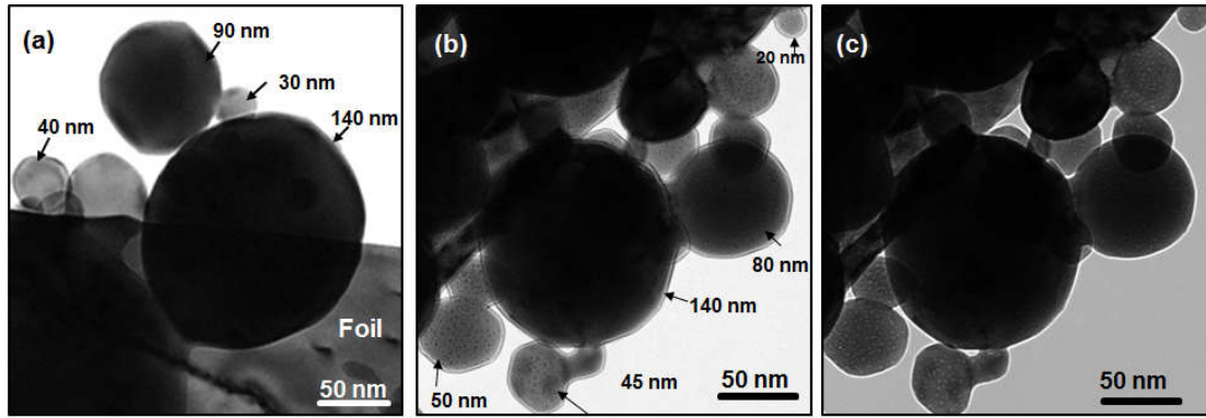
Figure 2. Bright-field TEM images showing the distribution of bubbles in W NPs of different sizes after irradiation with 15 keV He to a fluence of 9.6 \times 10^{16} ions-cm ^{-2} at 750 °C showing: (a) a distribution of NPs of different sizes dispersed at the edge of the electropolished region of a W foil before irradiation; (b) 800 nm overfocus; and (c) 800 nm underfocus after irradiation. Small bubbles appear as black spots in overfocus and white spots in underfocus.
