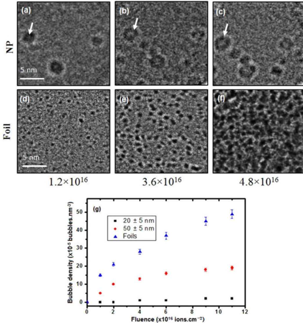
Figure 3. BF-TEM images comparing bubbles in a 35 nm diameter W NP (a–c) and foil (d–f) as a function of fluence taken at 400 nm overfocus. The arrows in a–c highlight the growth of a bubble in the NP as the fluence increases. (Scale marker in (a) and (d) applies to all images.) Figure (g) shows the relationship between bubble density and fluence for NPs with diameters of 20 \pm 5 and 50 \pm 5 nm in the foil.
