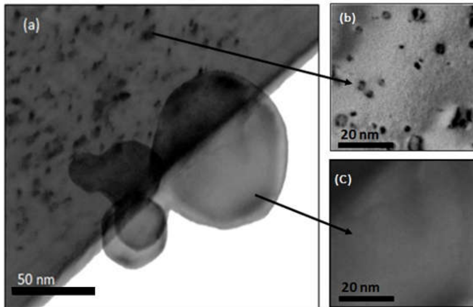
Figure 7. TEM images of: (a) NPs of different sizes and W foil irradiated to 1.1 \times 10^{17} ions·cm -2 ; (b) enlarged area of the foil after tilting >15^\circ to be close to a different zone axis to that shown in (a) to avoid any possible g · b invisibility criteria; and (c) enlarged area of NP after equivalent tilting of >15^\circ . Note the complete absence of dislocation loops in the NPs evident in (a) and (c).
