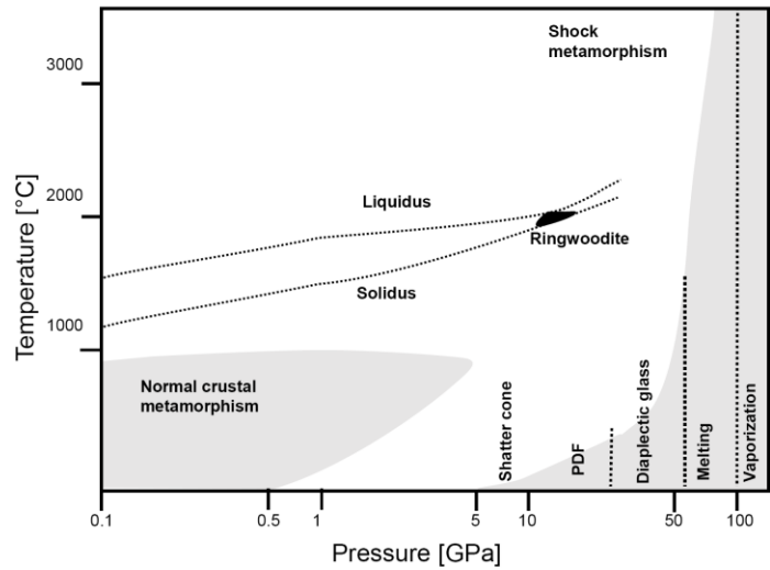
Figure 3. Pressure vs. temperature diagram for regional metamorphism in the Earth’s crust compared to shock compression of non-porous silicate rocks (modified after French 1998). The liquidus, solidus and stability field of ringwoodite, a high pressure phase of olivine, is displayed as a simplified version of a phase diagram for the composition of the carbonaceous chondrite Allende (Agee et al. 1995). During shock compression a local temperature excursion in the host rock is required to reach the stability field of ringwoodite.
