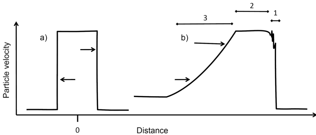
Figure 5. Propagation of the release wave following a strong shock shown as particle velocity with distance to the plane of impact. The plane of impact is at zero distance. a) Arrows indicate the direction of the shock waves that move from the point of impact into the target and into the projectile. b) Arrows indicate the direction and pressure (length of arrows) of the release wave that was reflected from the back of the projectile (see Text). 1] rise of the shock; 2] broad plateau; 3] decompression.
