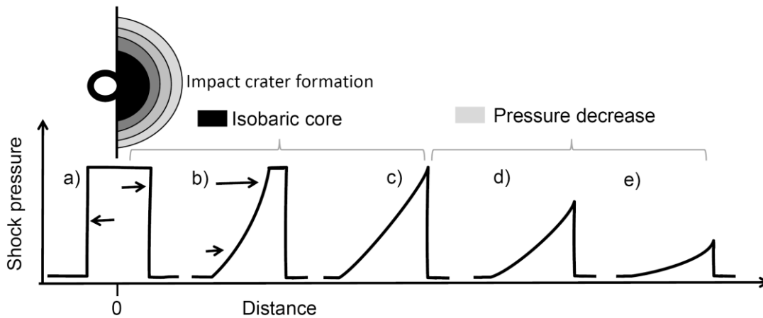
Figure 6. Pulse length and intensity of a shock wave with distance to the plane of impact. The plane of impact is at zero distance. a) Arrows with different directions show the shock waves that move into the target and into the projectile. b) Arrows with different length show the velocity of the release wave that was reflected from the back of the projectile (see text). The propagating shock wave interacts with the following faster release wave. a-c) In the isobaric core the shock pressure remains high but the width and, thus, the temporal duration of the broad pressure plateau decreases. d-e) After the shock wave lost the broad pressure plateau the pressure starts to decrease by interacting with the release wave.
