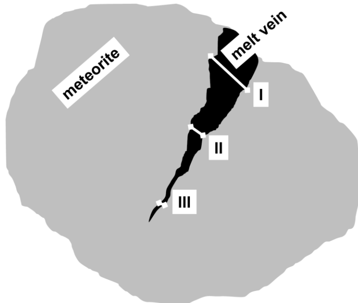
Figure 10. Sketch of a meteorite hosting a melt vein with different thickness. Depending on the size of the melt, it quenches at time scales I) longer, II) equal to or III) shorter than the duration of the shock. This means the melt vein quenches in situation I) after pressure release, in situation II) during pressure release, and in situation III) at isobaric conditions if the host rock is within the isobaric core or during declining shock pressure if the rock is outside the isobaric core.
