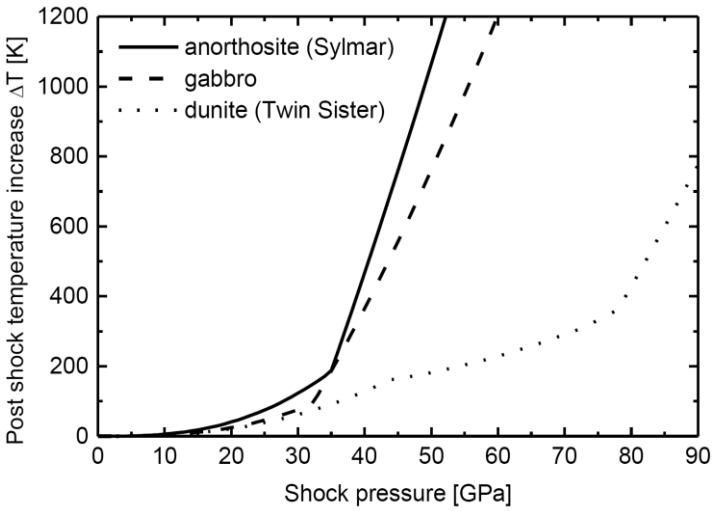
Figure 4. Post shock temperature increase calculated for different materials using the experimentally measured Hugoniot data of Twin Sister dunite, Sylmar anorthosite (Stöffler, 1982) and a gabbro (Trunin et al. 2001). The post shock temperature increase is calculated using the linear relation of shock wave and particle velocity across specific shock pressure intervals as described by Artemieva and Ivanov (2004) and Fritz et al. (2005b). Anorthosite = a felsic igneous rock composed mainly of plagioclase; Gabbro = a mafic plutonic rock composed mostly of plagioclase and pyroxene and sometimes olivine. Dunite = an ultramafic plutonic rock composed mainly of olivine.
