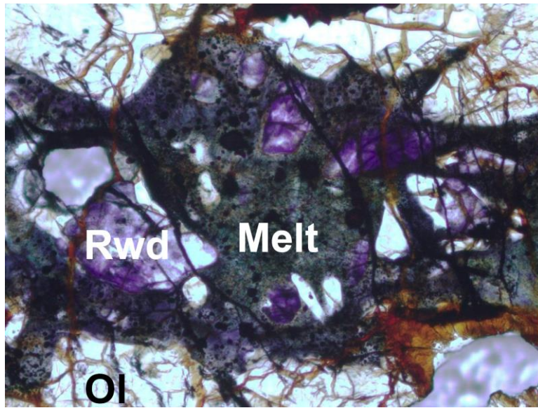
Figure 9. Transmitted light optical microscope image of pink to greenish ringwoodite in the melt vein of the L6 chondrite Northwest Africa 6525. Field of view is 400 \mu\text{m} wide. Rwd = ringwoodite; Ol = olivine.
