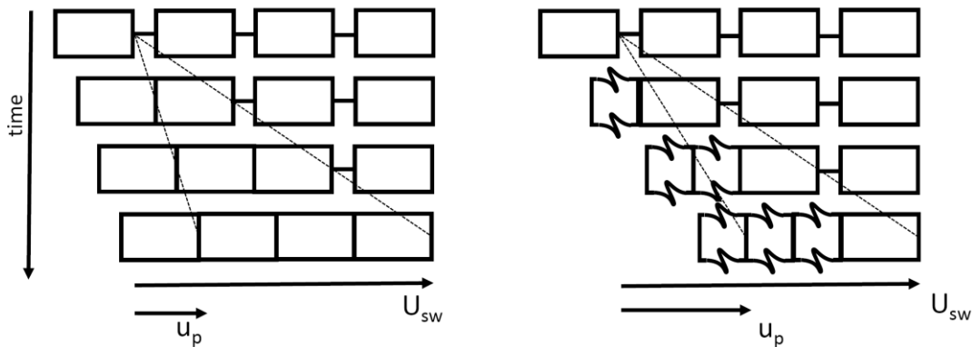
Figure 1. Illustration of the propagation of the shock wave and the material (particle) for materials of different compressibility. This could be two materials of different compressibility or material shocked to two different pressures at which the compressibility of the material substantially differs. Shock wave velocity = U_{sw} ; particle velocity = u_p .
