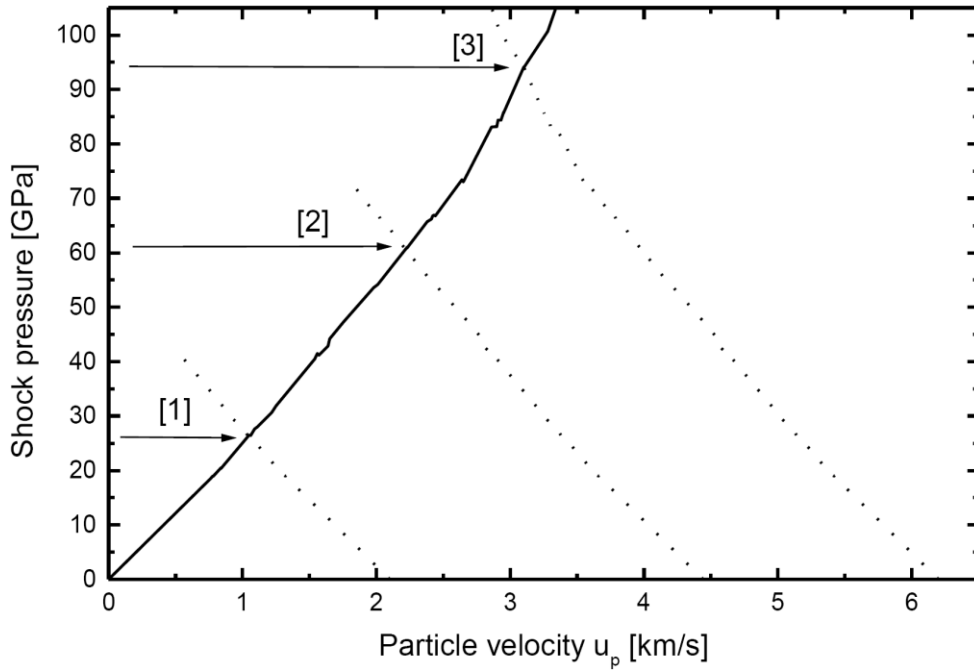
Figure 7. Graphical determination of the shock pressures produced during planar impacts at different velocities of a projectile and target both made of dunite. The Hugoniot curve for the Twin Sister dunite (data from Stöffler 1982) is displayed as a function of pressure and particle velocity.
