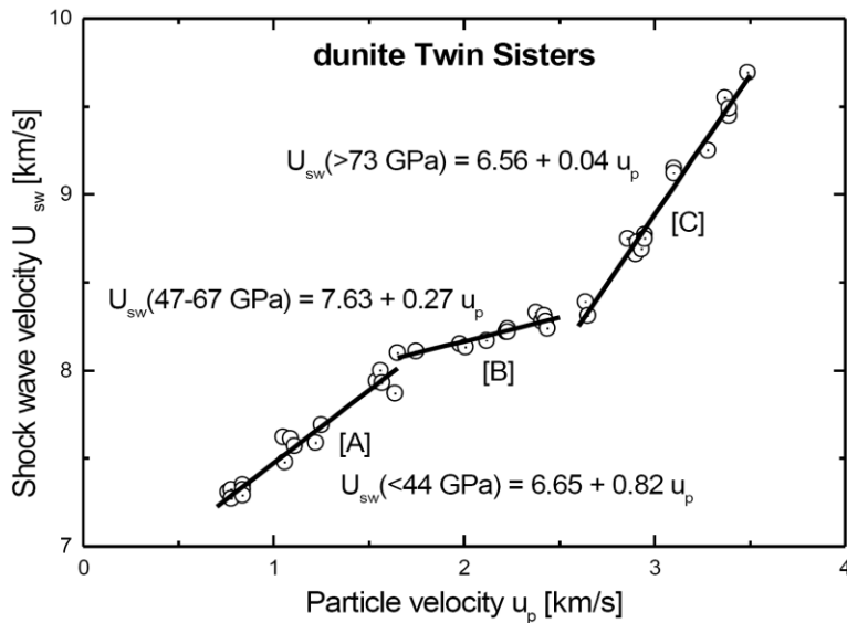
Figure 8. Experimentally determined shock wave and particle velocity for the Twin Sister dunite as tabulated by Stöffler (1982). The three branches with a linear increase in shock wave and particle velocity are labelled A, B, and C. They reflect substantial changes in the compressibility of the material at these shock pressures. The linear regression given as U_{sw} = C + S * u_p and these C and S values for specific shock pressure intervals can be used to calculate the shock induced temperature increase (see Figure 4).
