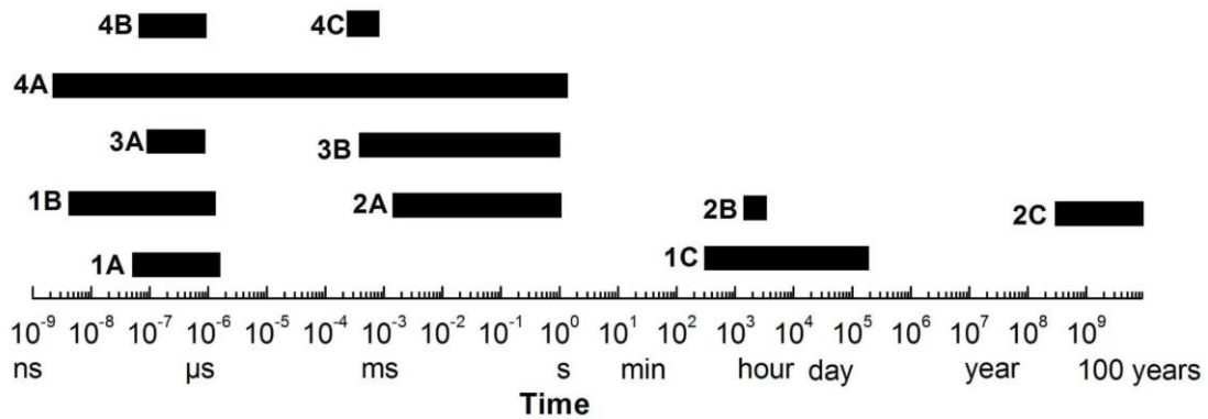
Figure 2. Overview of the time intervals of shock and thermal effects during impact cratering. Displayed are the duration of shock and static experiments (Langenhorst et al. 2002; Fritz et al. 2011), shock pulses in rocks during natural impact events and cooling times of millimetre to hundreds of meter sized rock units (Chen et al. 1996; Beck et al. 2005; Fritz et al. 2005; Xie et al. 2006; Fritz and Greshake 2009). [1A] Free surface velocity measurements of Hugoniot data; [1B] Shock recovery experiments; [1C] Static experiments; [2A] Cooling time of 0.1 to 1 mm wide shock melt veins; [2B] Cooling time of 0.4 to 1 meter in diameter sized rocks in space; 2C) Cooling time of 10 to 100 meter wide lithologies; [3A] Generation of destructive shock effects; [3B] High pressure phase formation in >10 \mu\text{m} wide melt veins of meteorites; [4A] Shock duration in natural impacts; [4B] Localized shock pressure peaks on the millimetre scale; [4C] Shock pressure equilibration on the meter scale.
