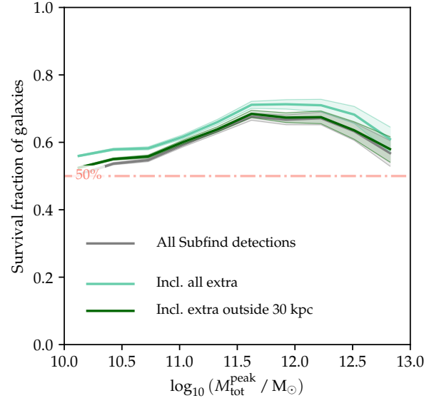
Figure B2. Fraction of galaxies in massive clusters ( M_{200c}^{z=0} > 10^{14.5} M_\odot ) that survive to z=0 . The grey line includes all galaxies present in the SUBFIND catalogue. The light green line adds galaxies which retain a self-bound remnant with at least ten particles when starting from all particles that are part of the galaxy in its last snapshot. The dark green line limits those recovered detections to only those that lie away from subhaloes in the SUBFIND catalogue (see text for details). There is no significant population of surviving galaxies that is missed by SUBFIND, particularly with the more restrictive definition (dark green).
