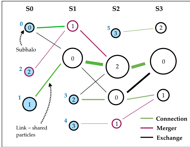
Figure A1. Example tracing situation with 14 subhaloes (circles with inscribed number representing their arbitrary ID and size indicating their mass) in 4 snapshots S0–S3 (different columns). Lines represent links, i.e., particle overlaps between subhaloes, whose width scales with link particle number (for simplicity assuming that all particles have equal mass). Green lines represent links that connect successive subhaloes of the same galaxy. The first subhalo of each galaxy is shaded blue, with a number to the left indicating the (arbitrary) galaxy ID. Purple circles indicate the last subhalo of a galaxy about to disrupt/merge, with the corresponding purple link pointing to the galaxy’s carrier in the next snapshot. Black lines represent exchange links between galaxies.
